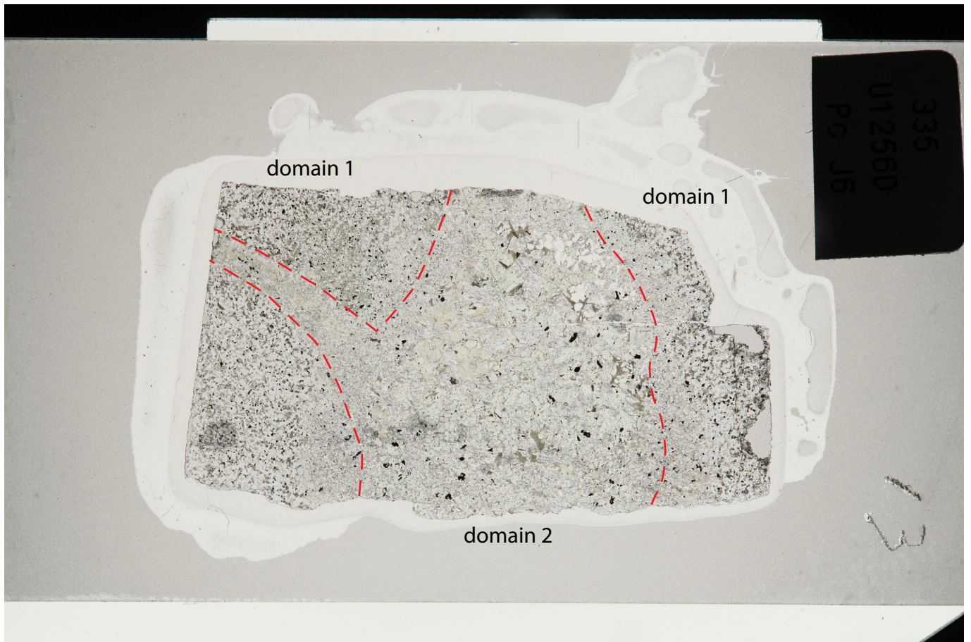
Sample 335-1256D-Run11-EXJB-J6 (Thin Section 13)
