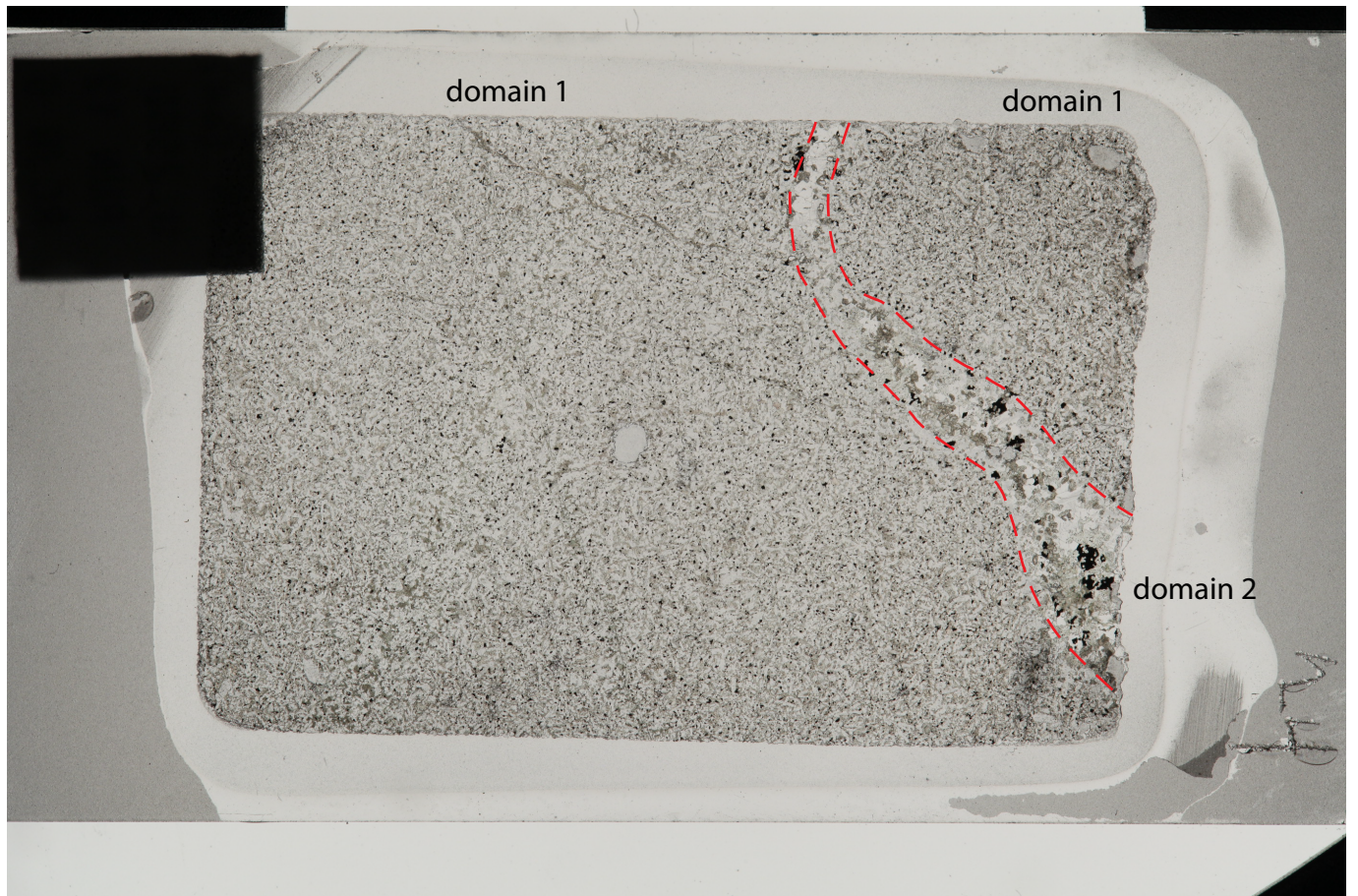
Sample 335-1256D-Run12-RCJB-Rock G (Thin Section 24)
