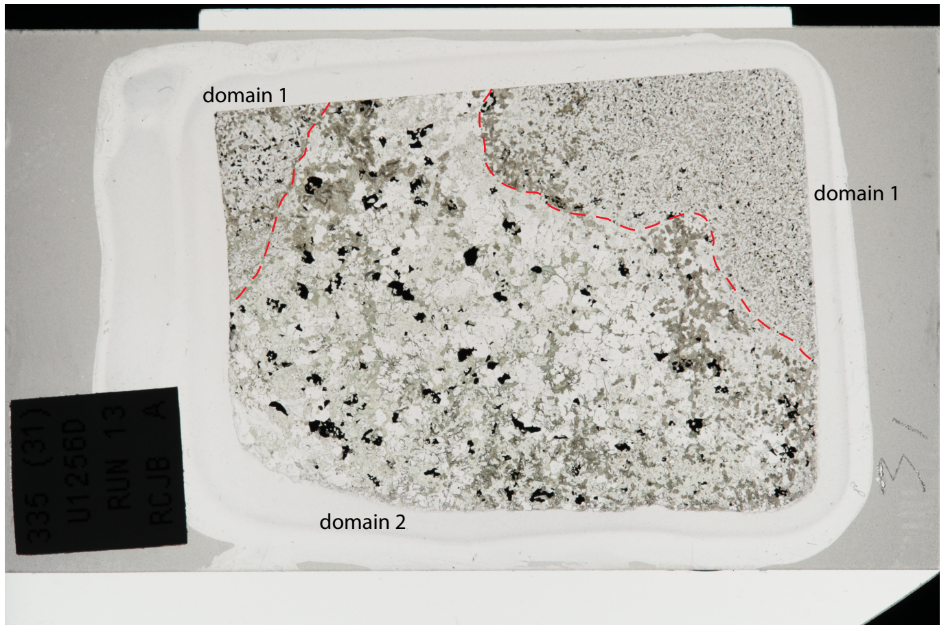
Sample 335-1256D-Run13-RCJB-Rock A (Thin Section 31)
