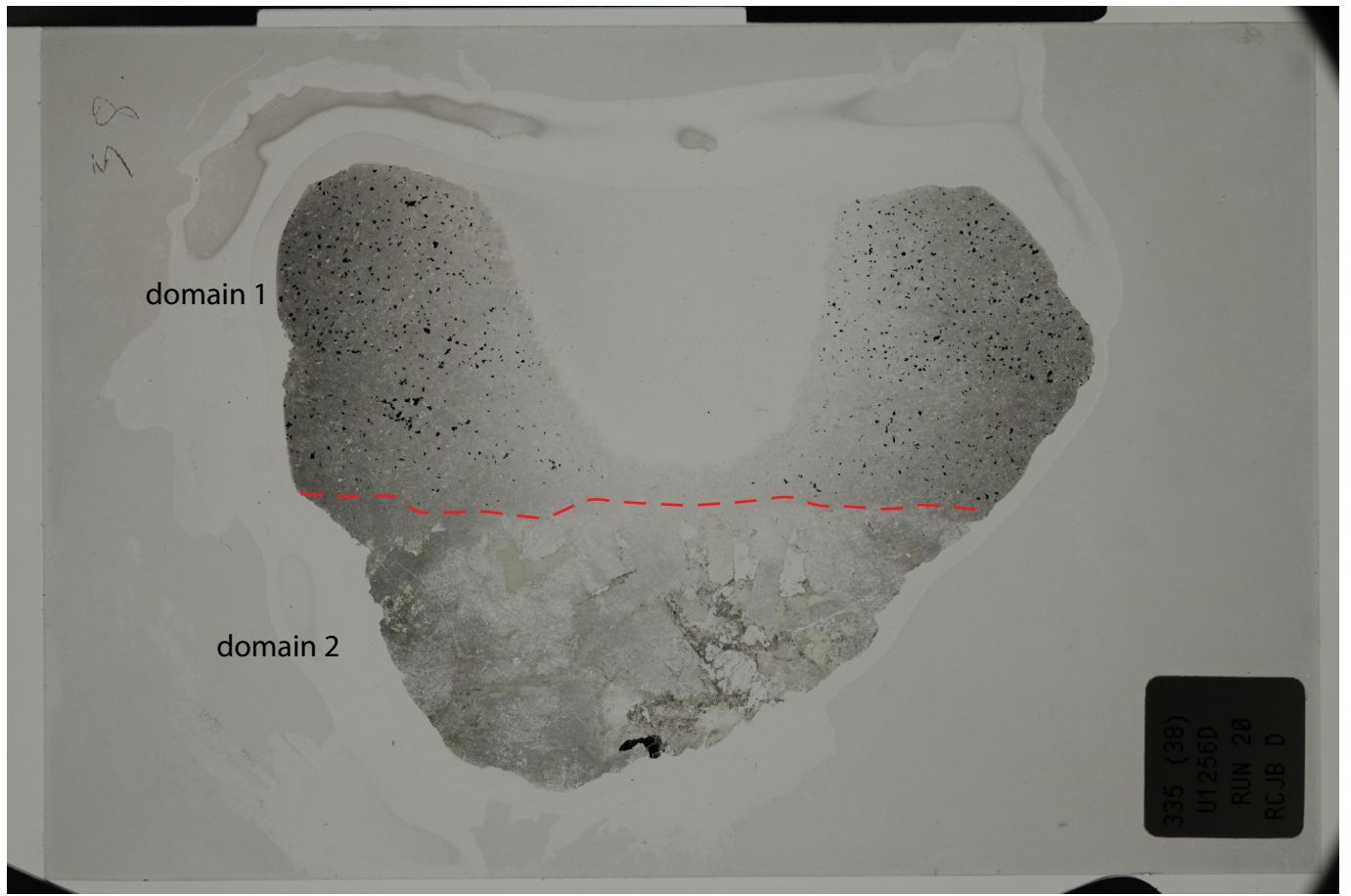
Sample 335-1256D-Run20-RCJB-Rock D (Thin Section 38)
