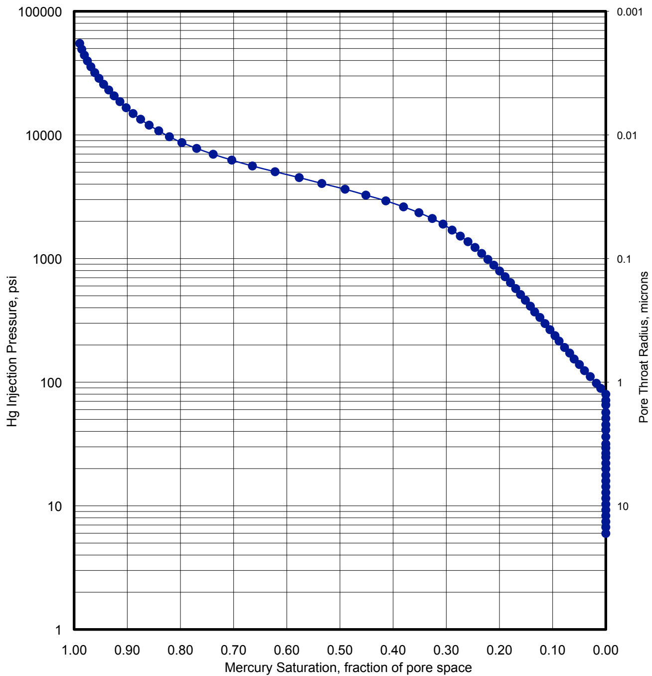
Figure S3. Mercury injection data for Sample 338-C0002F-167SMW
