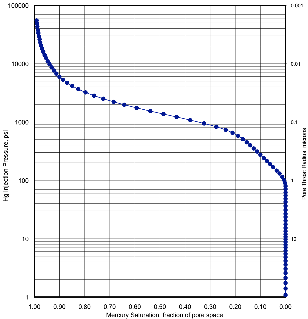
Figure S8. Mercury injection data for Sample 338-C0002J-1R-7
