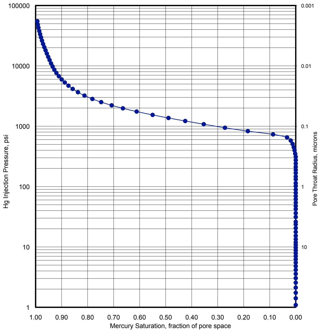
Figure S19. Mercury injection data for Sample 338-C0002L-20X-6
