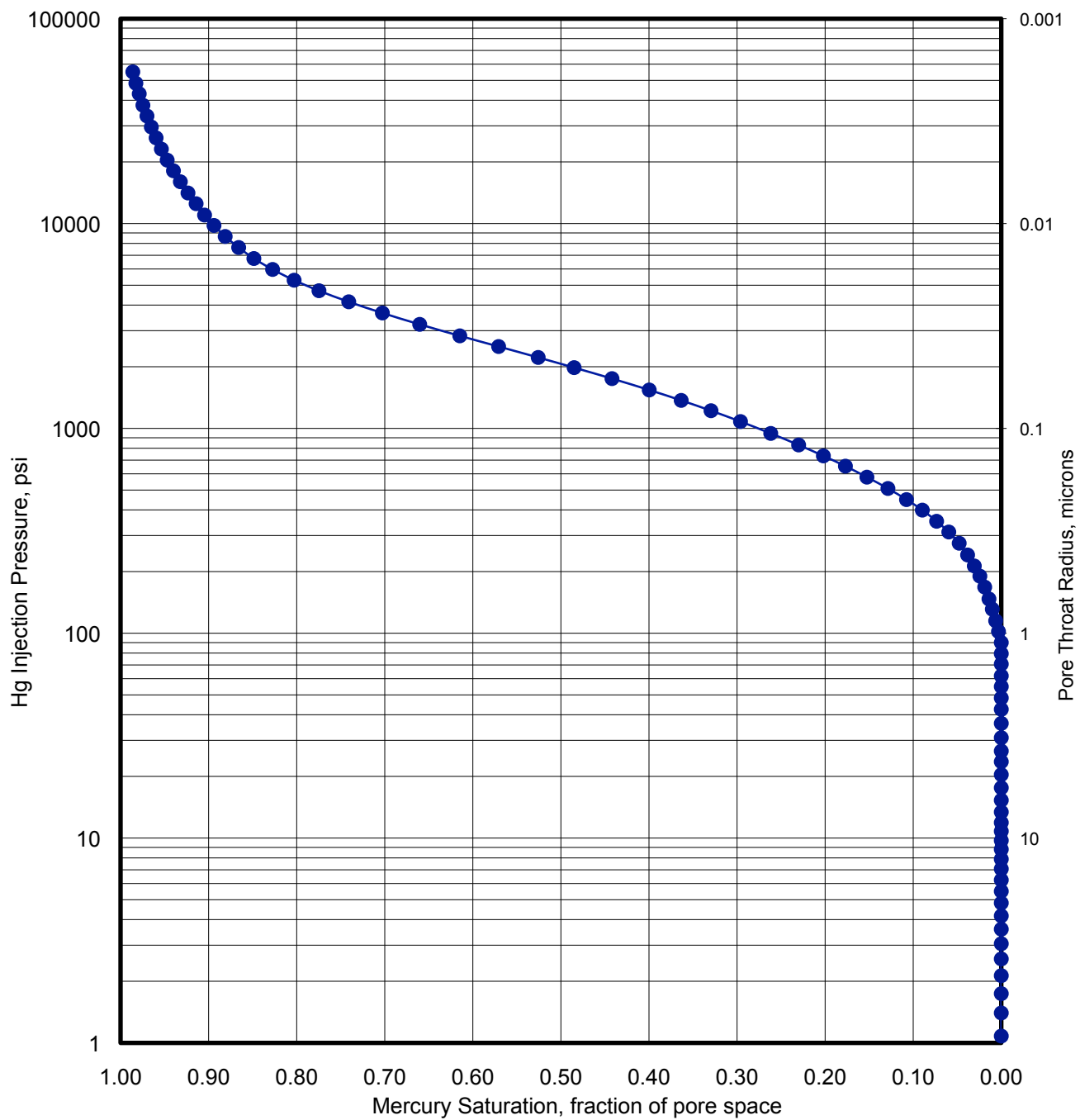
Figure S9. Mercury injection data for Sample 338-C0002J-3R-1
