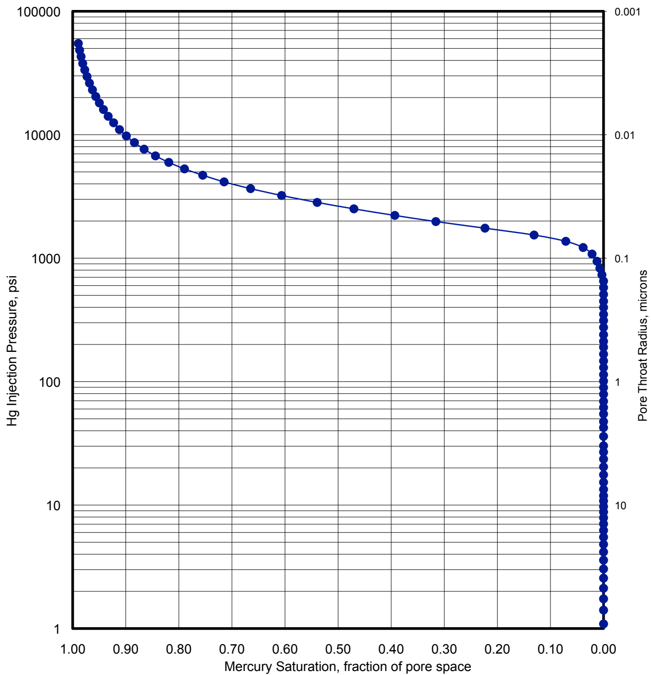
Figure S10. Mercury injection data for Sample 338-C0002J-5R-7
