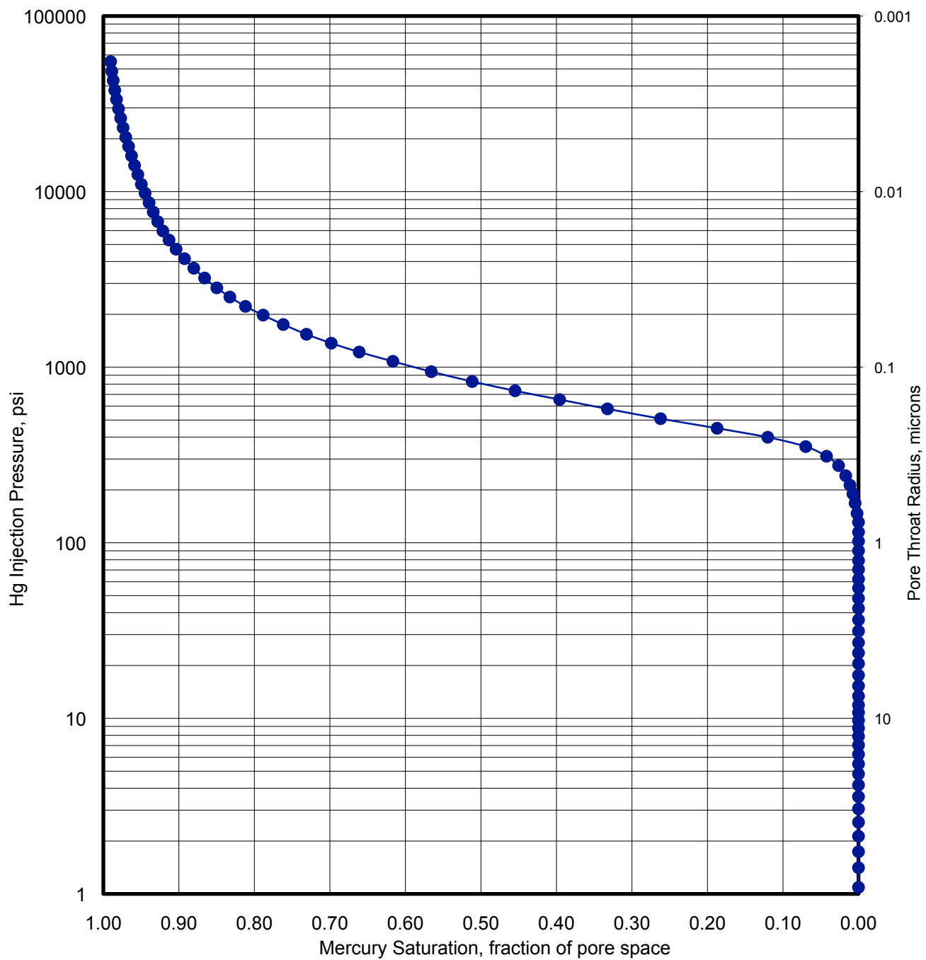
Figure S16. Mercury injection data for Sample 338-C0002L-11X-5
