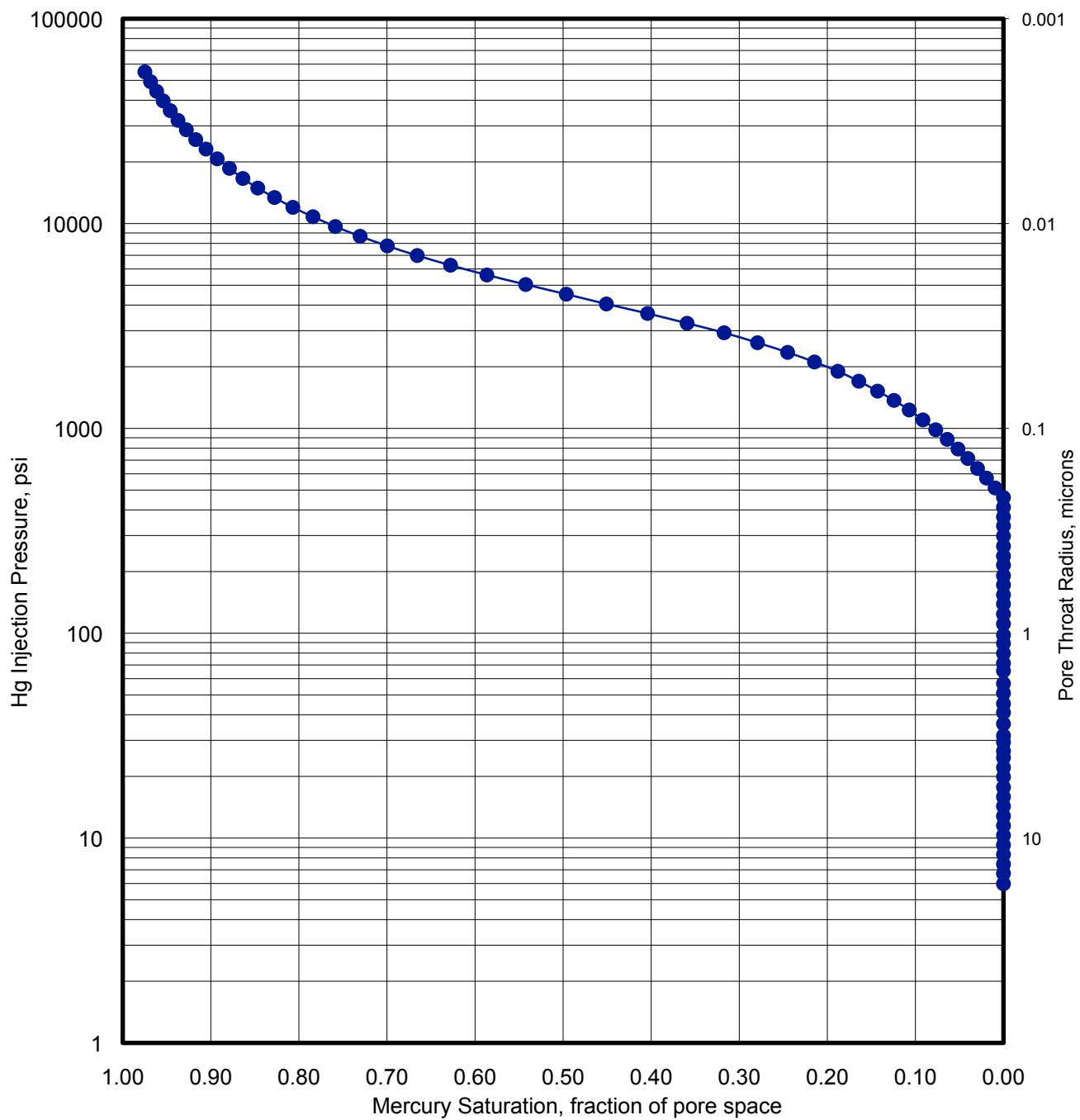
Figure S4. Mercury injection data for Sample 338-C0002F-211SMW
