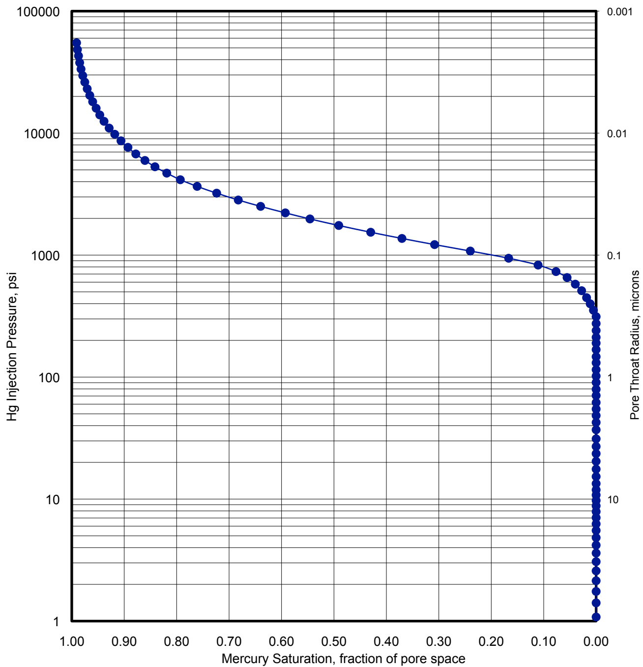
Figure S7. Mercury injection data for Sample 338-C0002H-2R-1
