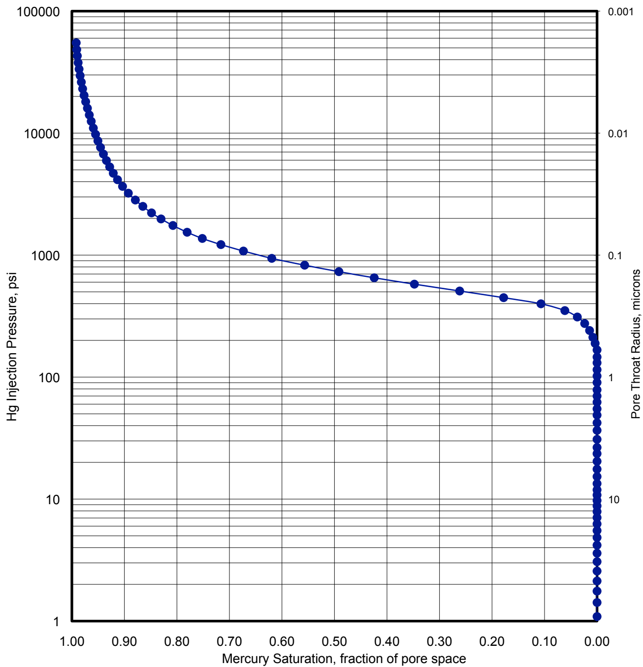
Figure S12. Mercury injection data for Sample 338-C0002K-8X-5
