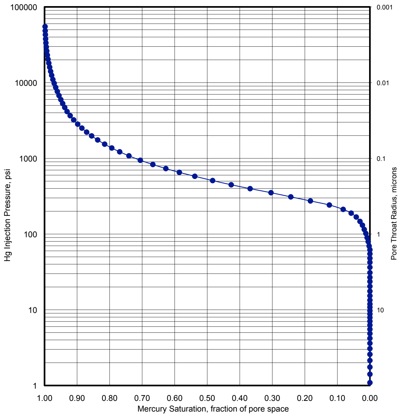
Figure S13. Mercury injection data for Sample 338-C0002L-1X-3
