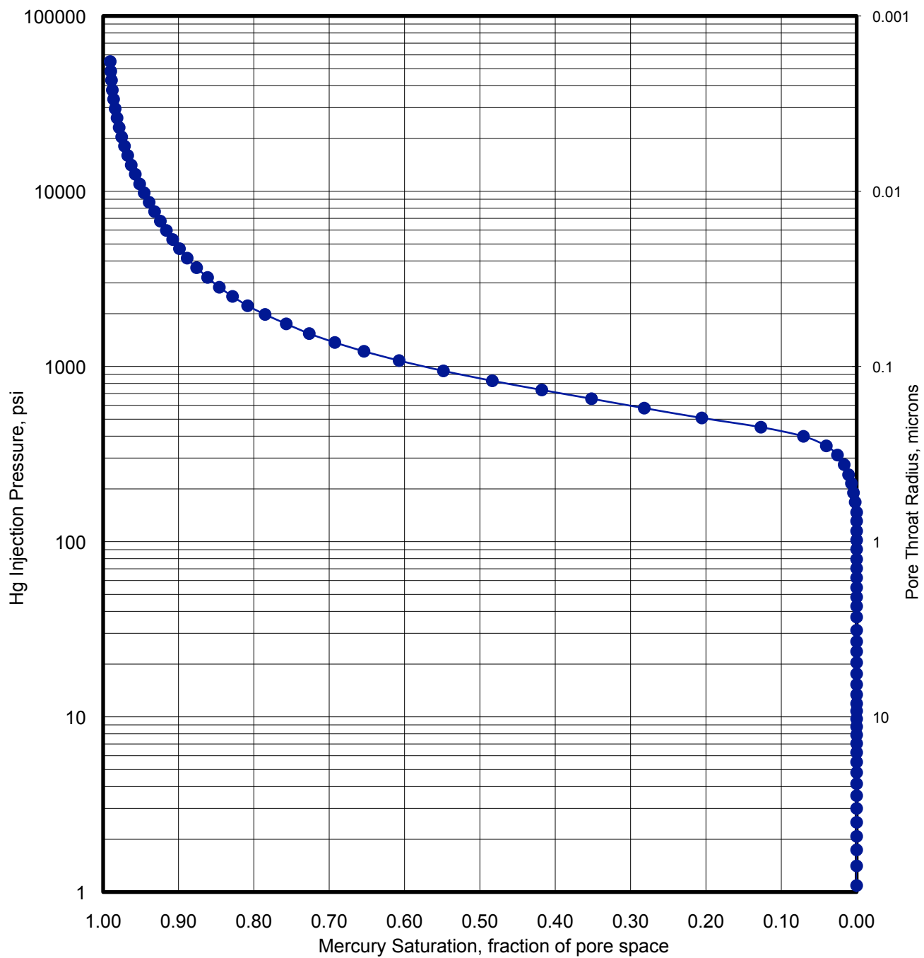
Figure S15. Mercury injection data for Sample 338-C0002L-8X-6
