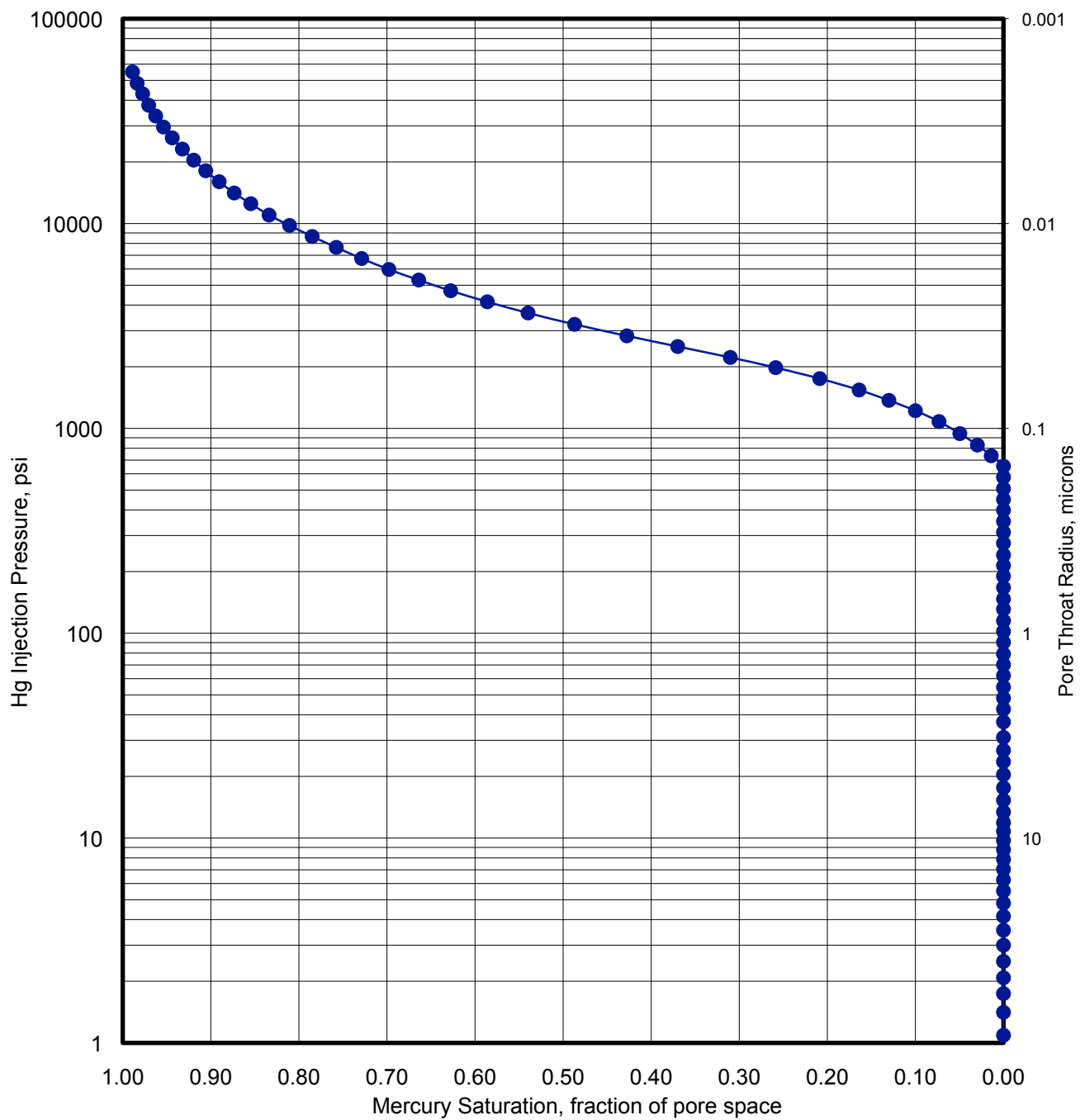
Figure S2. Mercury injection data for Sample 338-C0002F-110SMW
