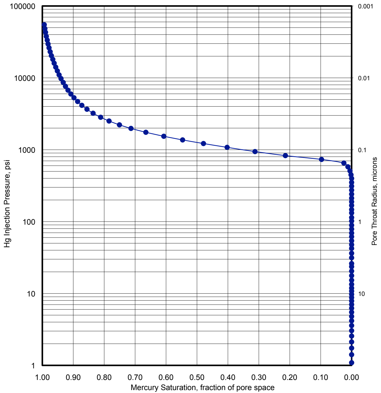
Figure S18. Mercury injection data for Sample 338-C0002L-17X-7
