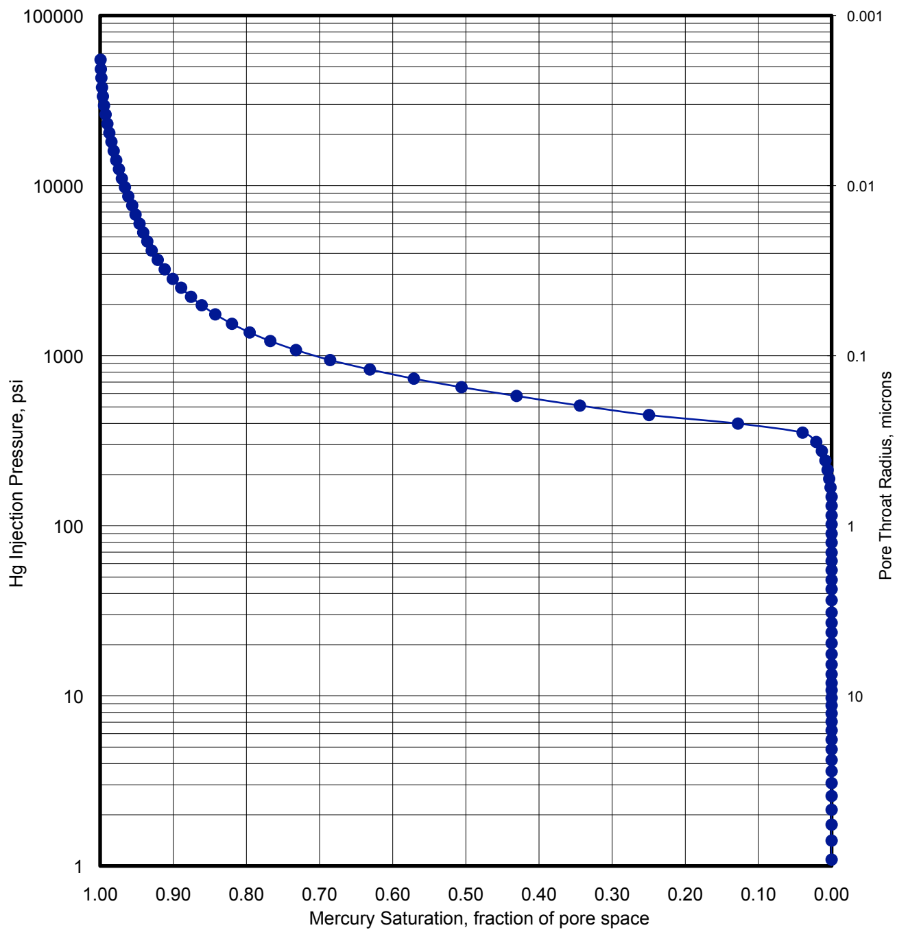
Figure S14. Mercury injection data for Sample 338-C0002L-4X-6
