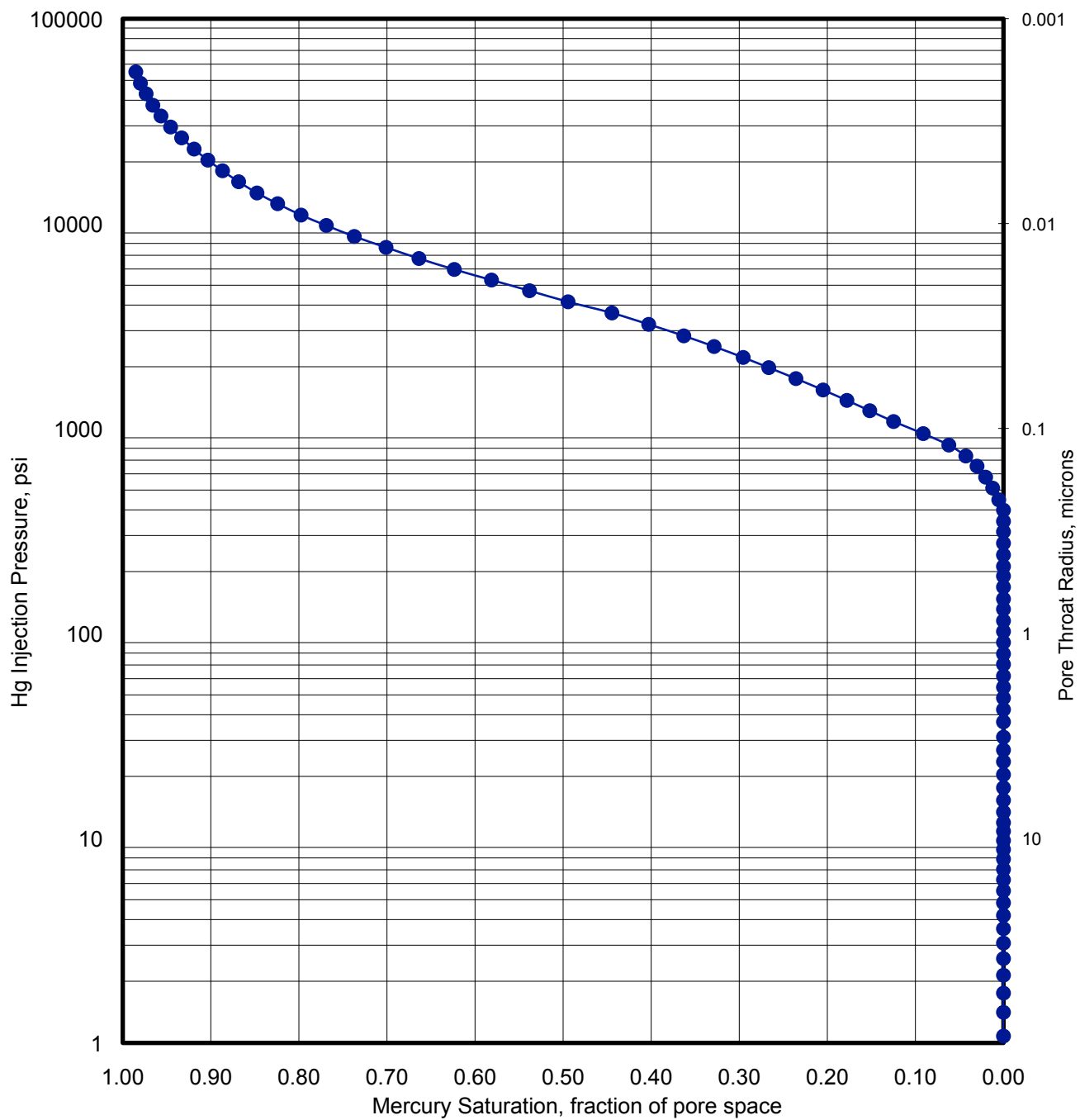
Figure S1. Mercury injection data for Sample 338-C0002F-21SMW
