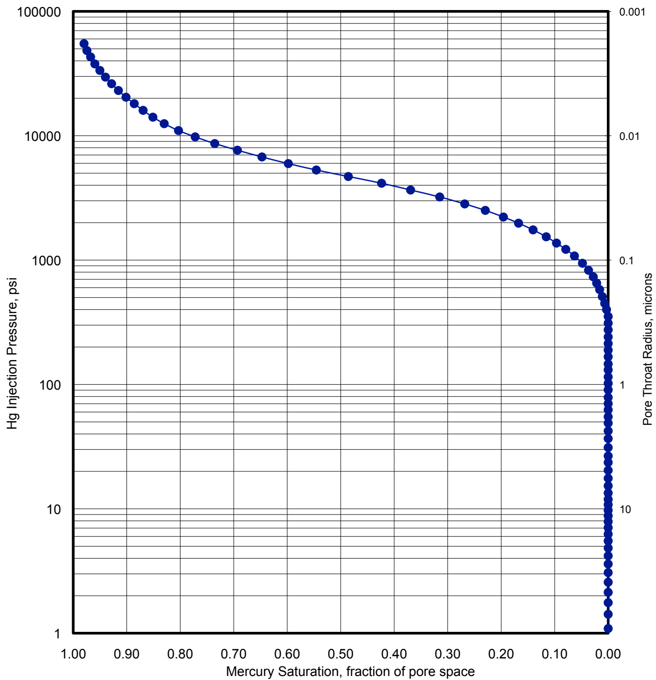
Figure S6. Mercury injection data for Sample 338-C0002F-312SMW
