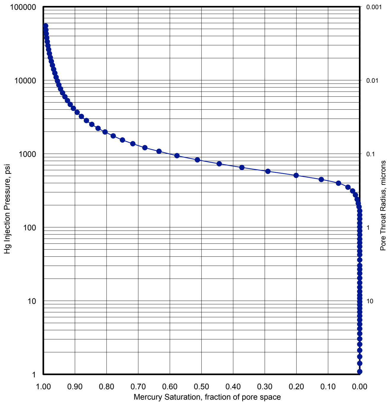
Figure S11. Mercury injection data for Sample 338-C0002K-5T-2
