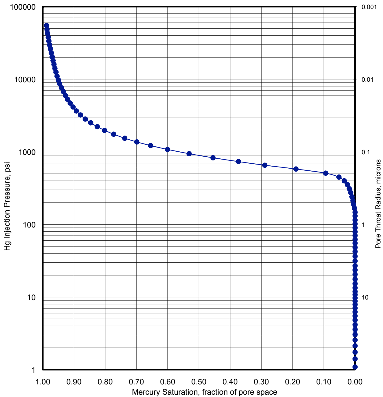
Figure S17. Mercury injection data for Sample 338-C0002L-14X-5
