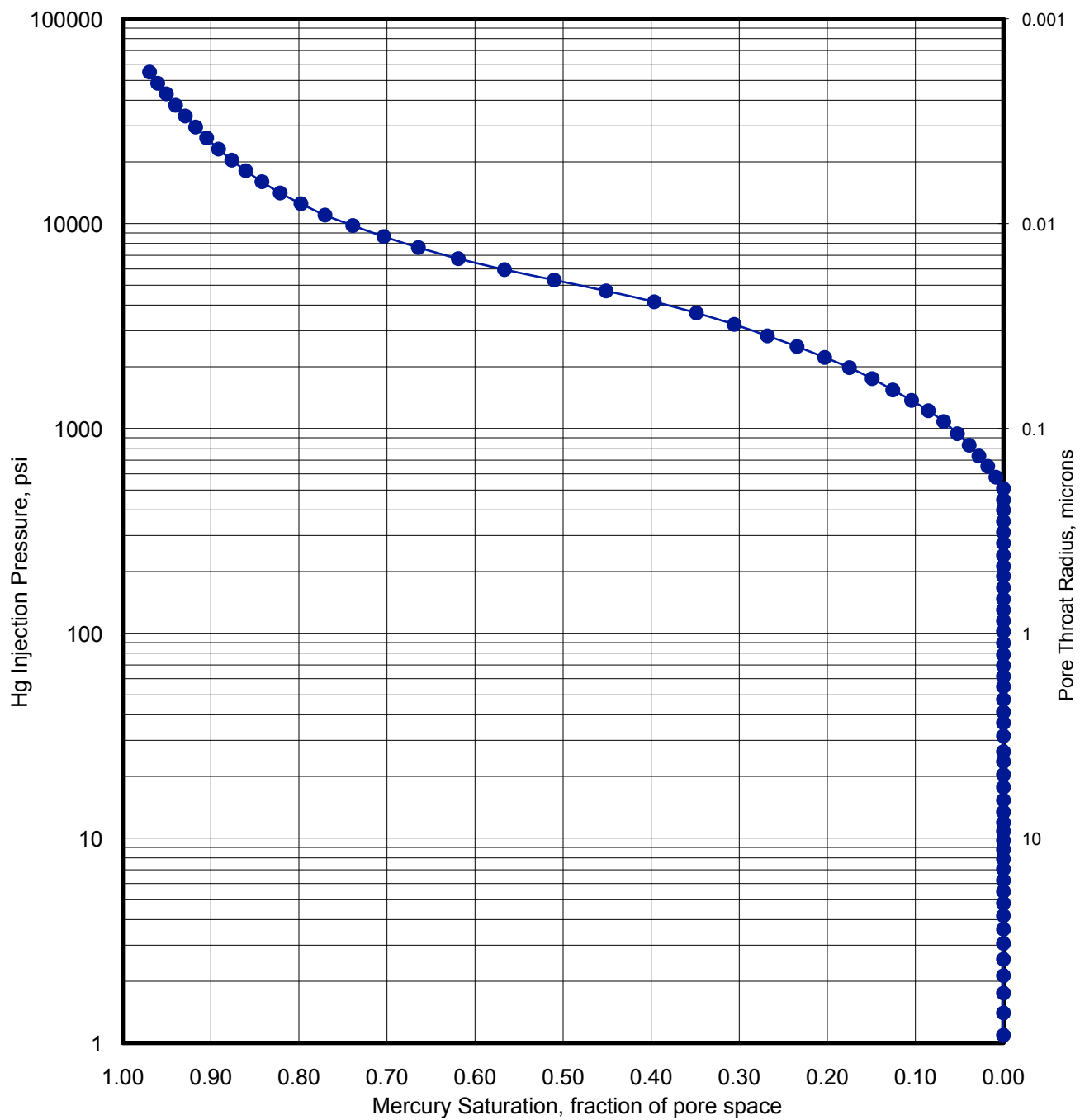
Figure S5. Mercury injection data for Sample 338-C0002F-267SMW
