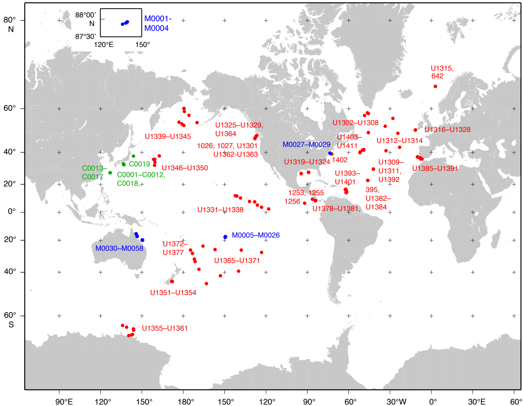
IODP Expeditions 301–336, 339–340, 342–343, Sites C0001–C0019 (●), M0001–M0058 (●), U1301–U1411 (●)
