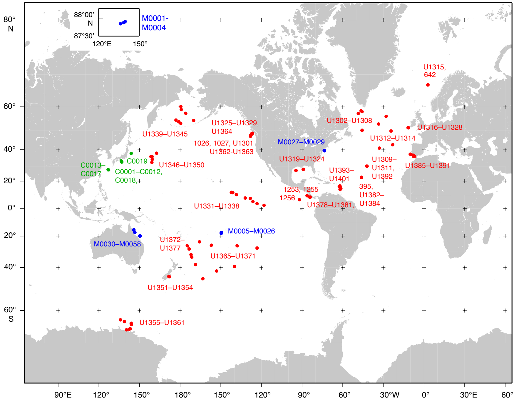
IODP Expeditions 301–336, 339–340, 343, Sites C0001–C0019 (●), M0001–M0058 (●), U1301–U1401 (●)
