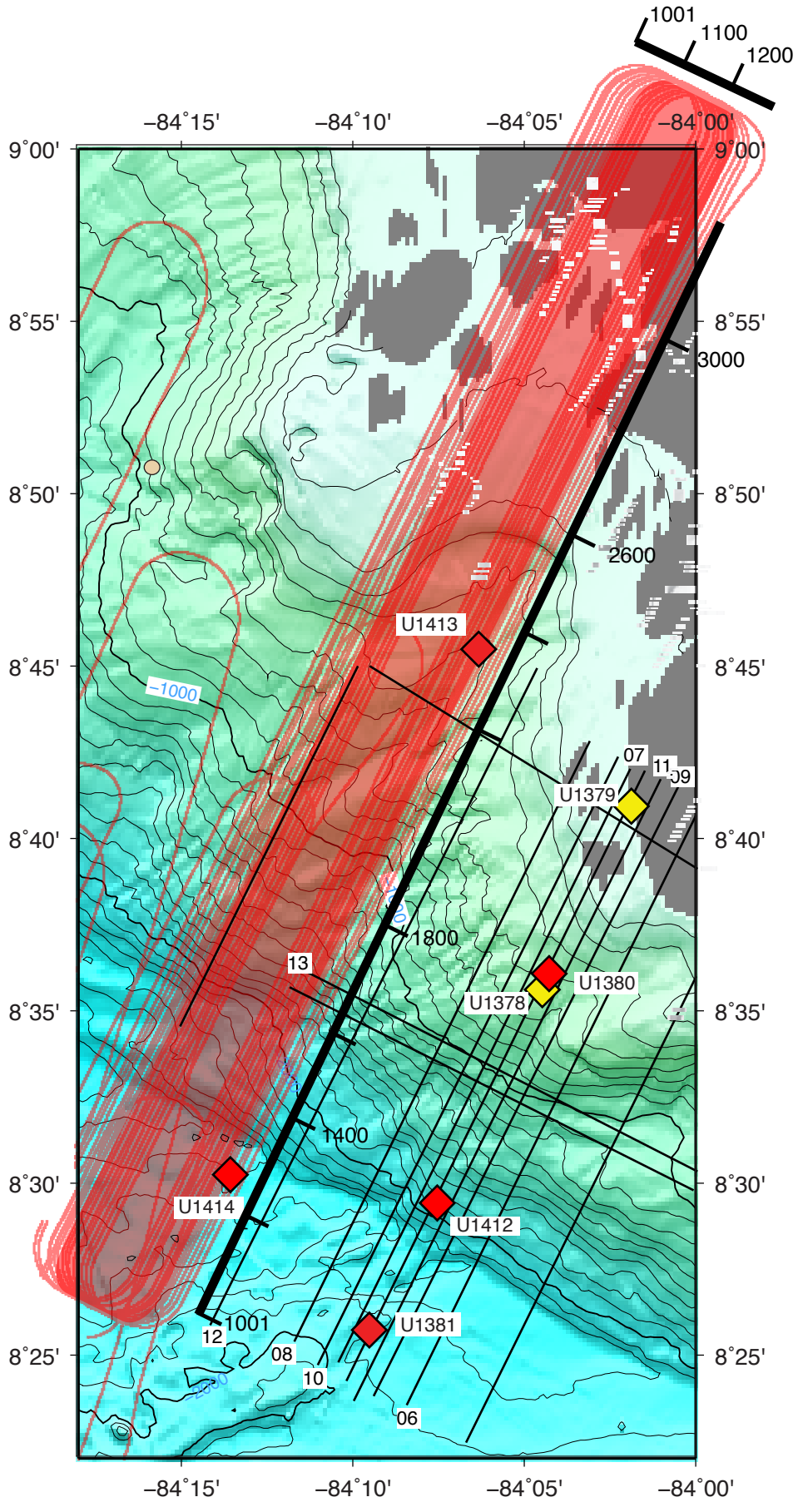
IODP Expedition 344 Site Map
