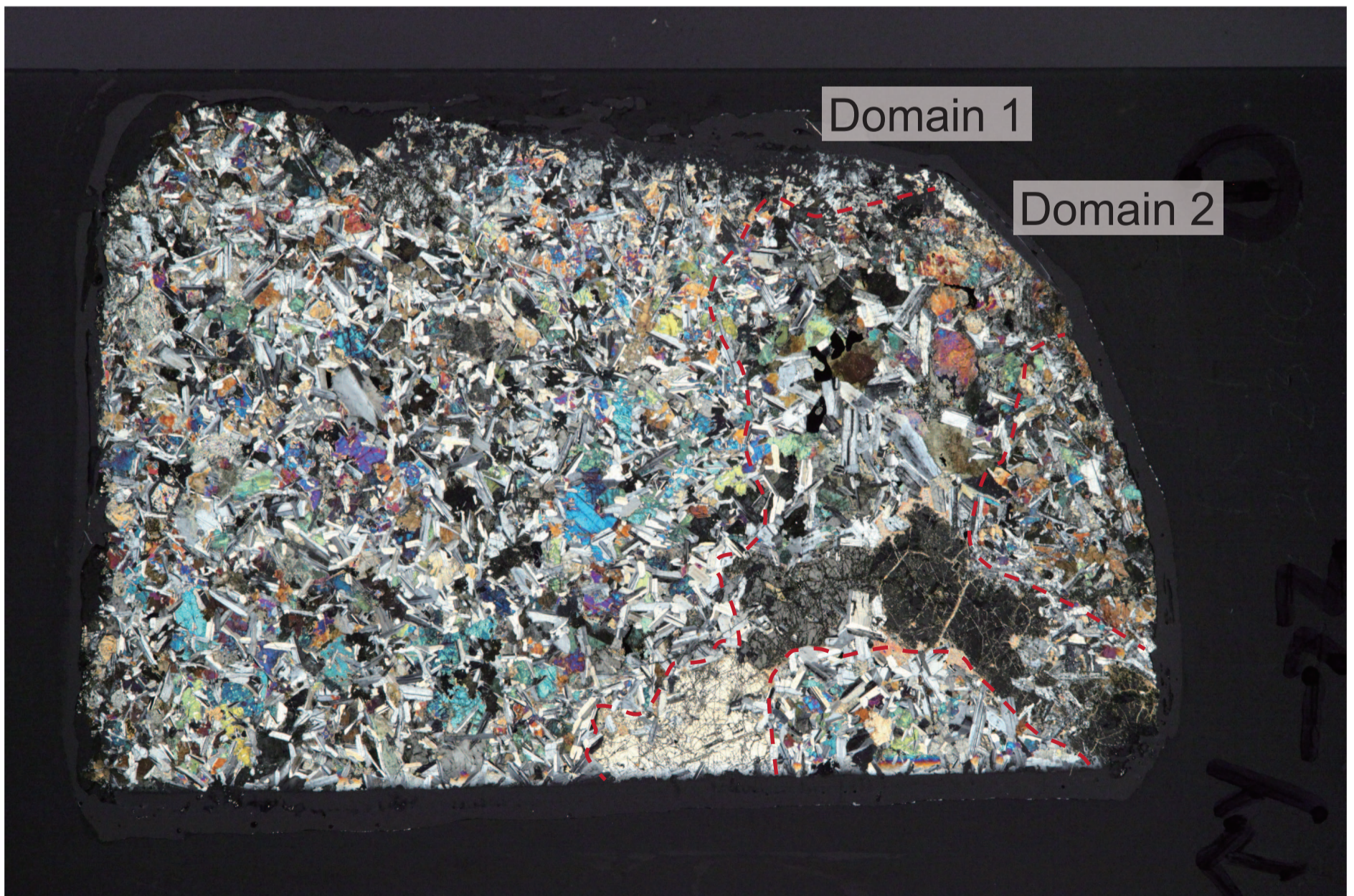
Thin section 1, Sample U1415E-1R-1, 21-23 cm, piece3
