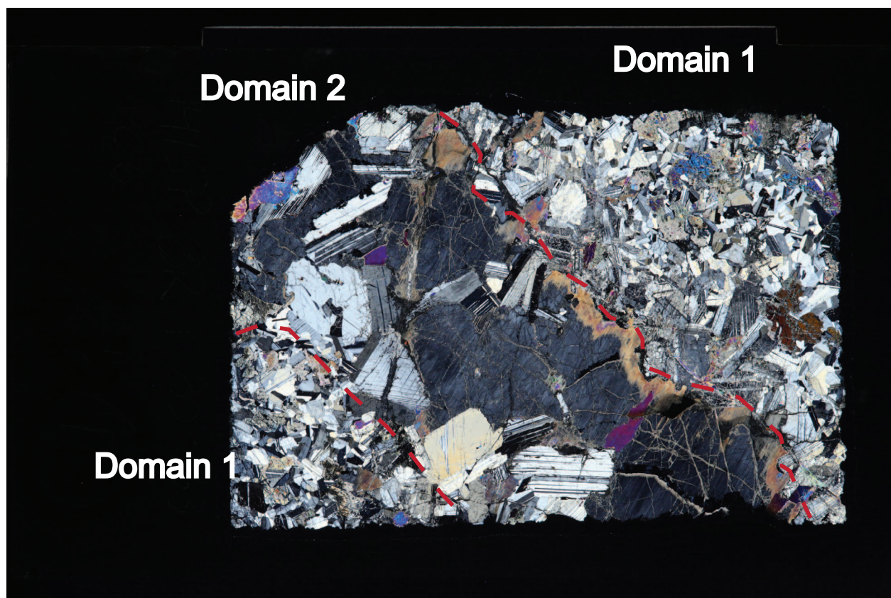
Thin section 116, Sample U1415P-8R-1, 80-83 cm, piece 6
