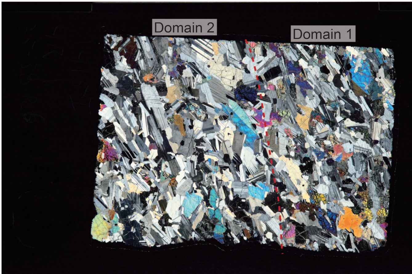
Thin section 21, Sample U14151-4R-1, 35-38 cm, piece6
