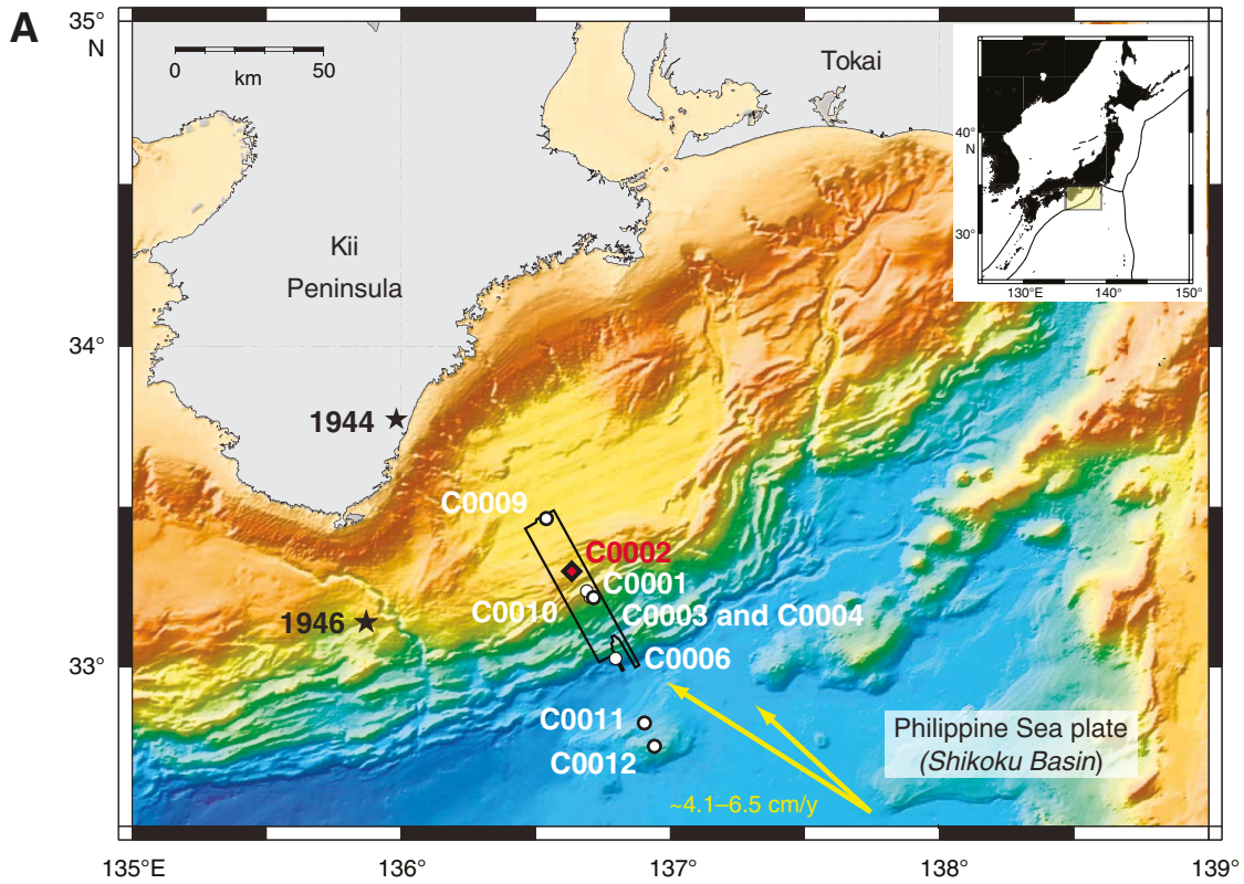
Figure F1. A. Map of the NanTroSEIZE region showing all Stage 1, 2, and 3 drill sites. Red = Expedition 348 Site C0002, white = other NanTroSEIZE sites. Black outline = region with 3-D seismic data, yellow arrows = estimated far-field vectors between Philippine Sea plate and Japan (Seno et al., 1993; Heki, 2007). Stars = epicenter locations of 1944 and 1946 tsunamogenic earthquakes. (Continued on next page.)
