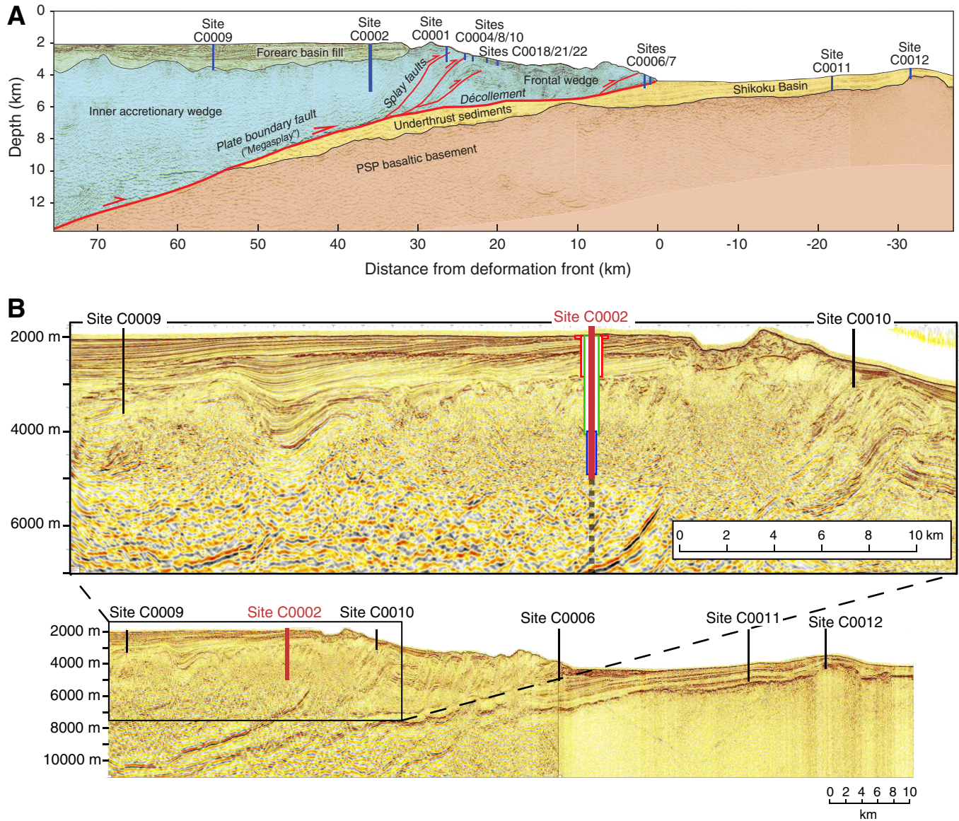
Figure F2. Seismic reflection depth sections with tectonic interpretation and selected NanTroSEIZE drill sites. A. Deep penetration depth section Line 5 (Park et al., 2002), reinterpreted in light of more recent geophysical imaging. B. Upper panel: expanded scale image of the region around Holes C0002F, C0002N, and C0002P. The heavy solid red line represents the currently drilled borehole, and the dashed line shows the projected extension to the plate boundary fault target. The boxes represent cased sections of Holes C0002F, C0002N, and C0002P (red shows the 36 and 20 inch casing, green represents the 13¾ inch casing, and blue indicates the 11¾ inch casing liner section). Lower panel: composite seismic depth section of the NanTroSEIZE site and related drilling sites from the Kumano Basin (Site C0009) to the input sites (C0011 and C0012).
