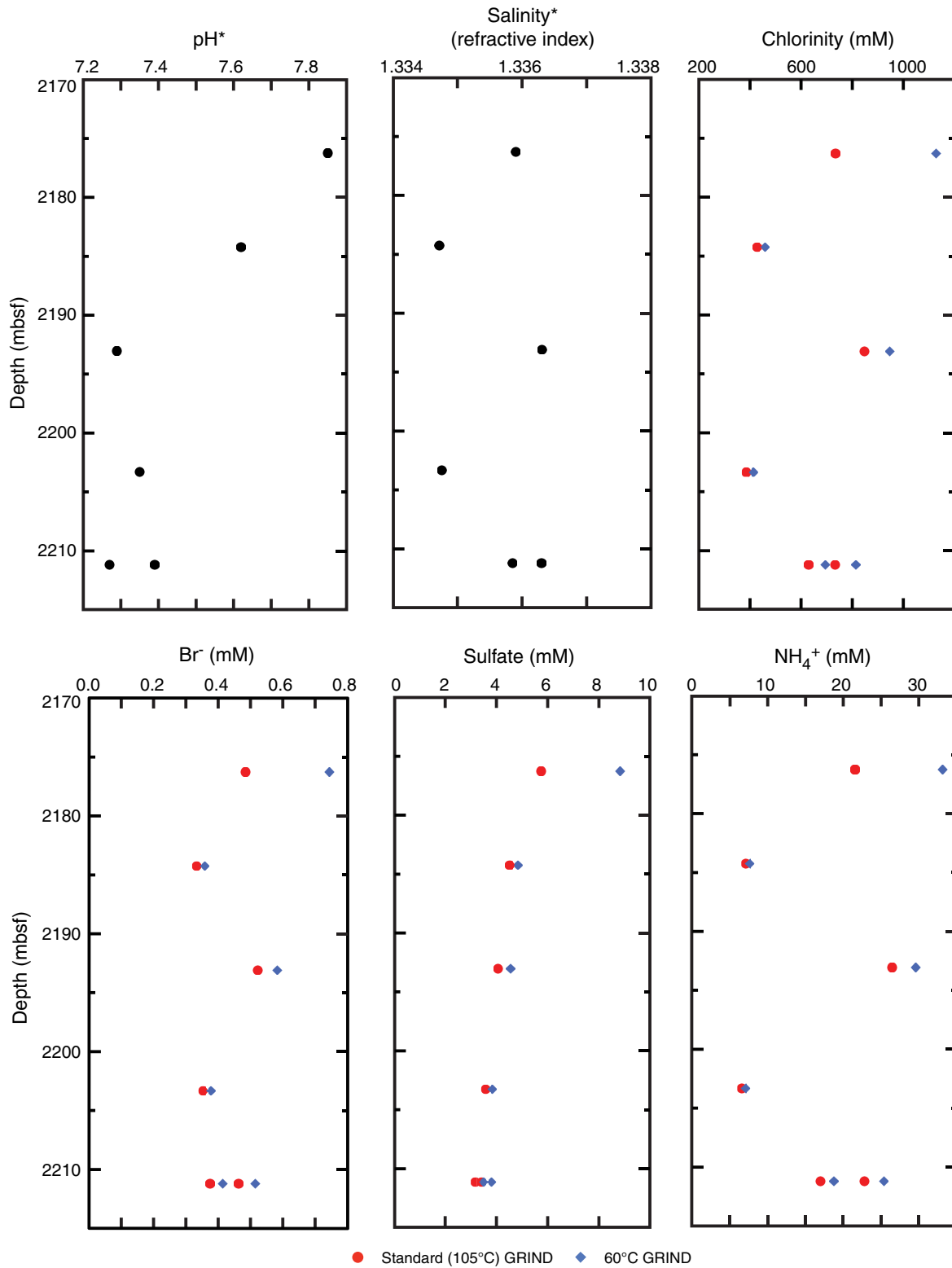
Figure F14. Salinity, pH, and downhole concentrations of chlorinity, bromide, sulfate, and ammonium determined by the ground rock interstitial normative determination (GRIND) method, Hole C0002P.
