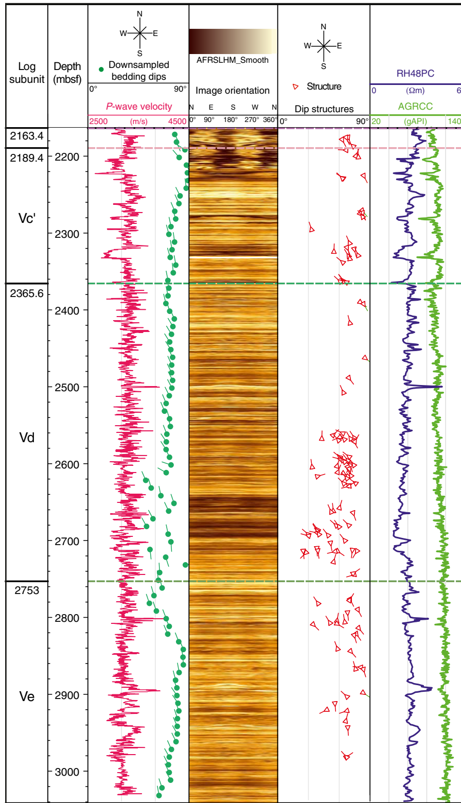
Figure F21. Summary of the preliminary interpretation of azimuthal focused resistivity (AFR) images displayed with velocity, resistivity (RH48PC), and gamma radioactivity (AGRCC). Tadpole plot of downsampled bedding dips (interval = 30 m, step = 15) and shipboard P -wave velocity, high-resolution AFR image (static processing), tadpole plot of structures, resistivity, and gamma ray logs.
