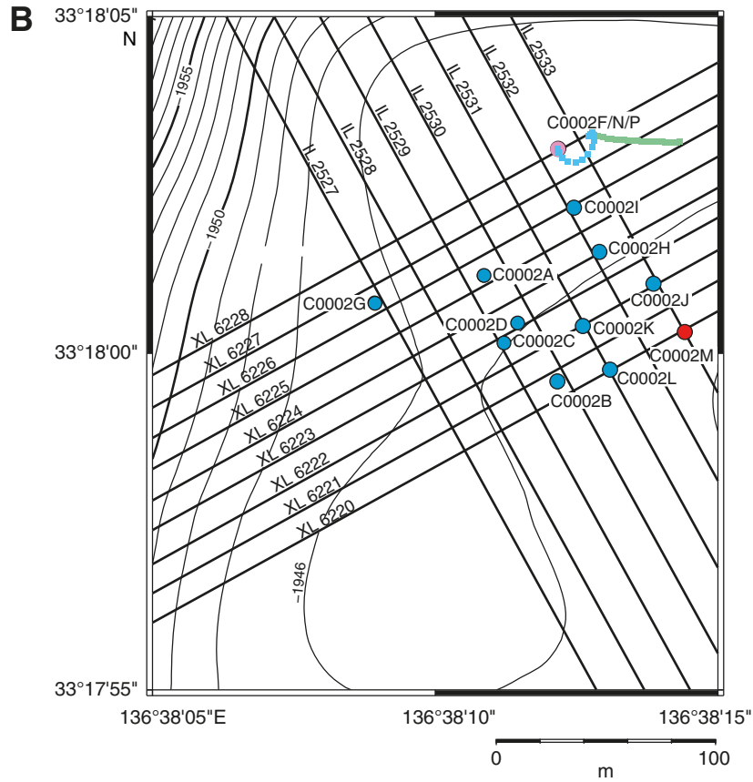
Figure F1 (continued). B. Bathymetric map showing all Site C0002 holes. The long-term borehole monitoring system is installed in Hole C0002G, and the riser hole is Hole C0002F/C0002N/C0002P. The lines from Hole C0002F show the azimuth and deflection of Holes C0002N (blue dashed line) and C0002P (green line) from the original Hole C0002F borehole.
