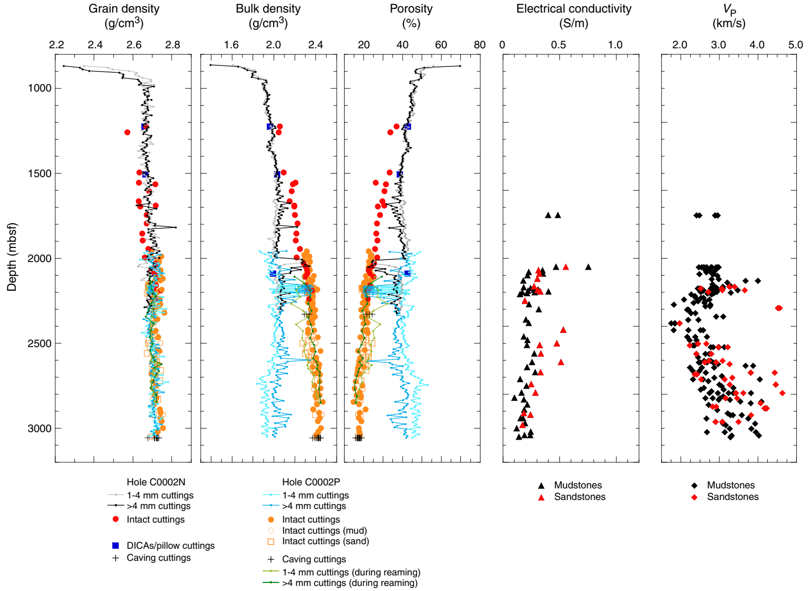
Figure F16. Physical properties measurements on 1–4 and >4 mm cuttings, Holes C0002N and C0002P. DICA = drilling-induced cohesive aggregate.
