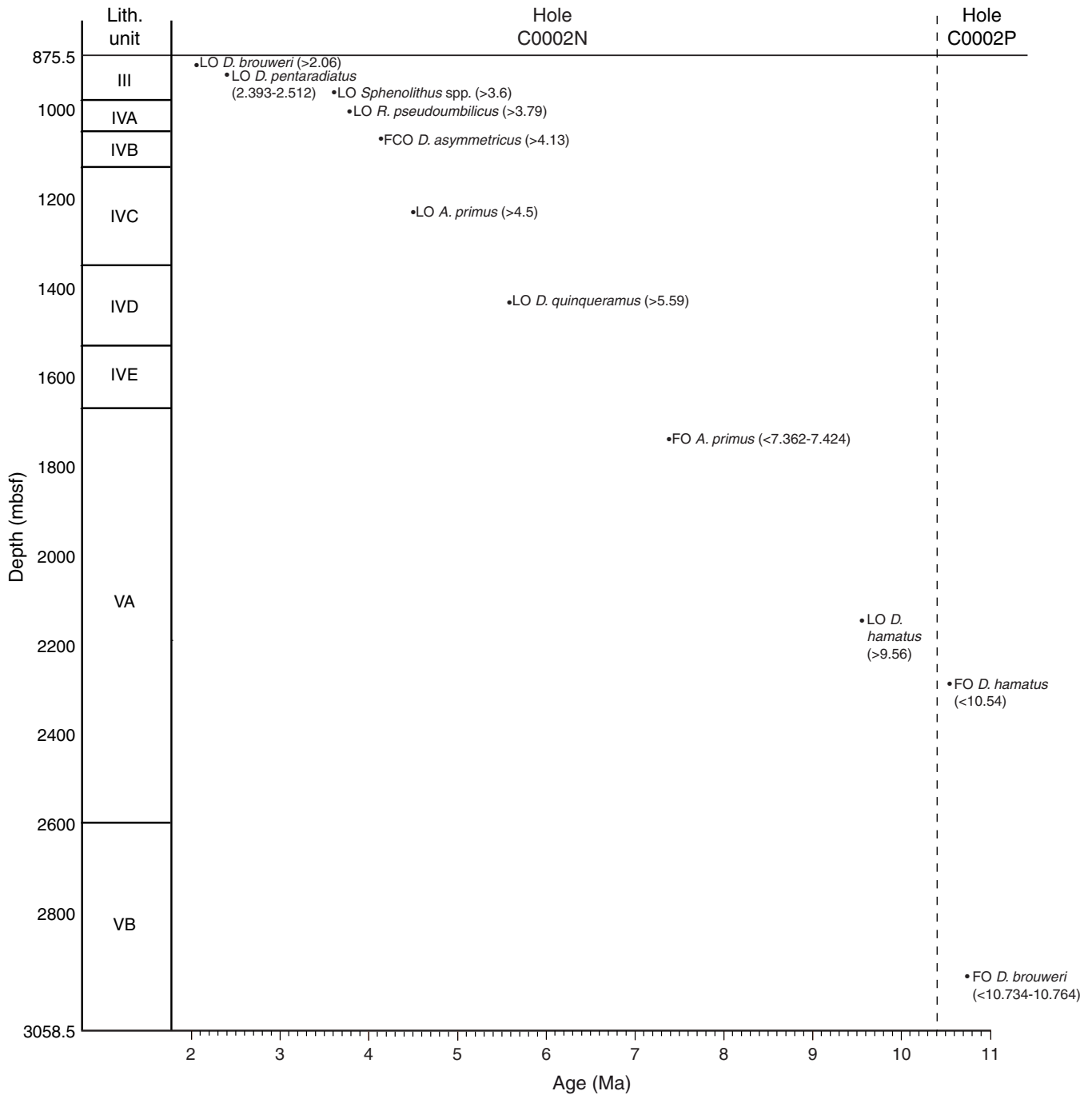
Figure F10. Nannofossil ranges presented as age-depth chart. Bedding dips vary between 60° and 90° and sediment is strongly deformed, so this information does not imply a mass accumulation rate. In Hole C0002P, diagnostic information is very limited, with poor preservation of calcareous fossils, perhaps because steep dips mean little stratigraphy was traversed; however, this data is broadly consistent with depositional ages between 9.56 and 10.73 Ma. LO = last occurrence, FCO = first common occurrence, FO = first occurrence.
