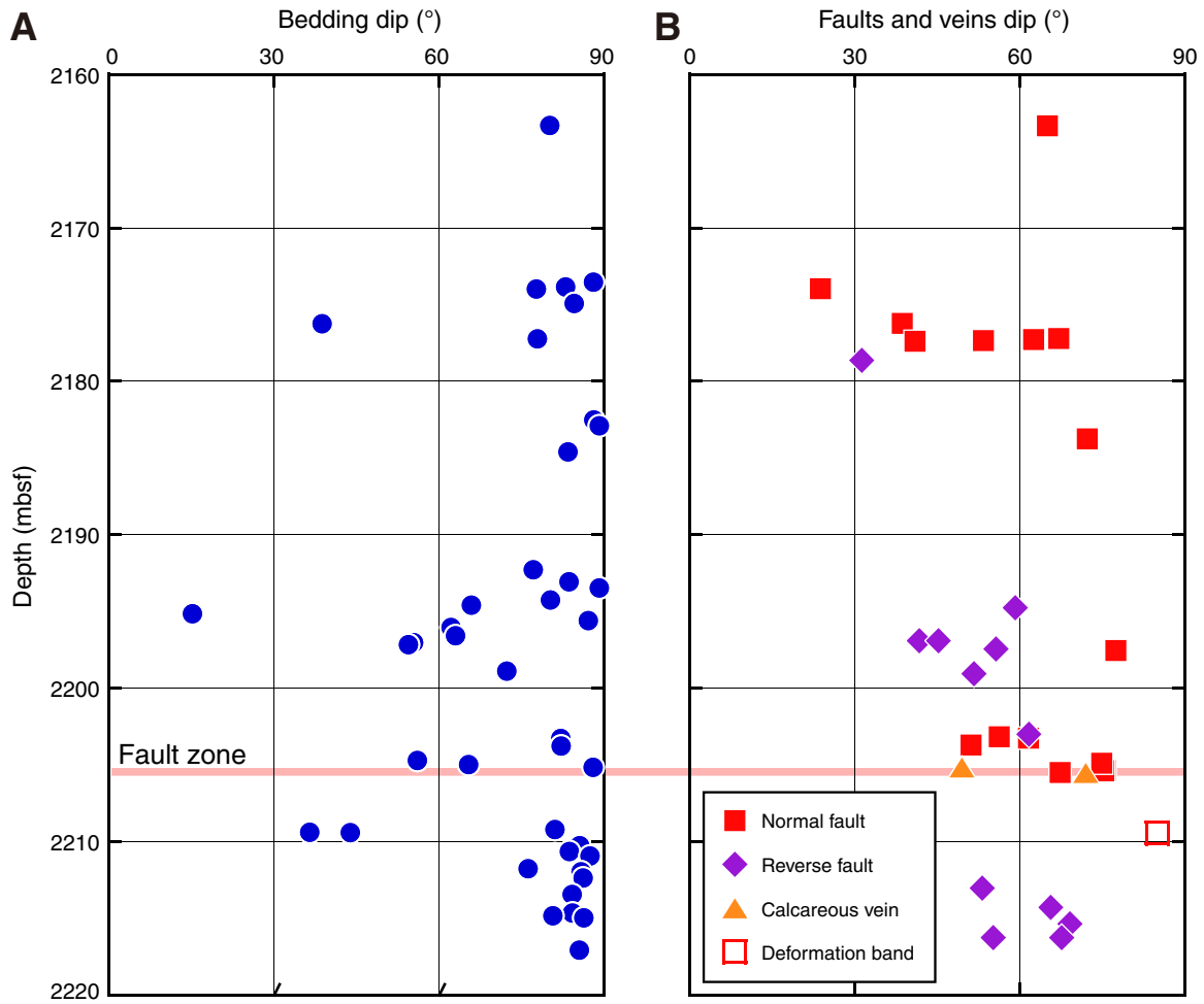
Figure F8. Depth distribution of dip angle variation measured in cores, Hole C0002P. A. Bedding. B. Minor faults, veins, and deformation band.
