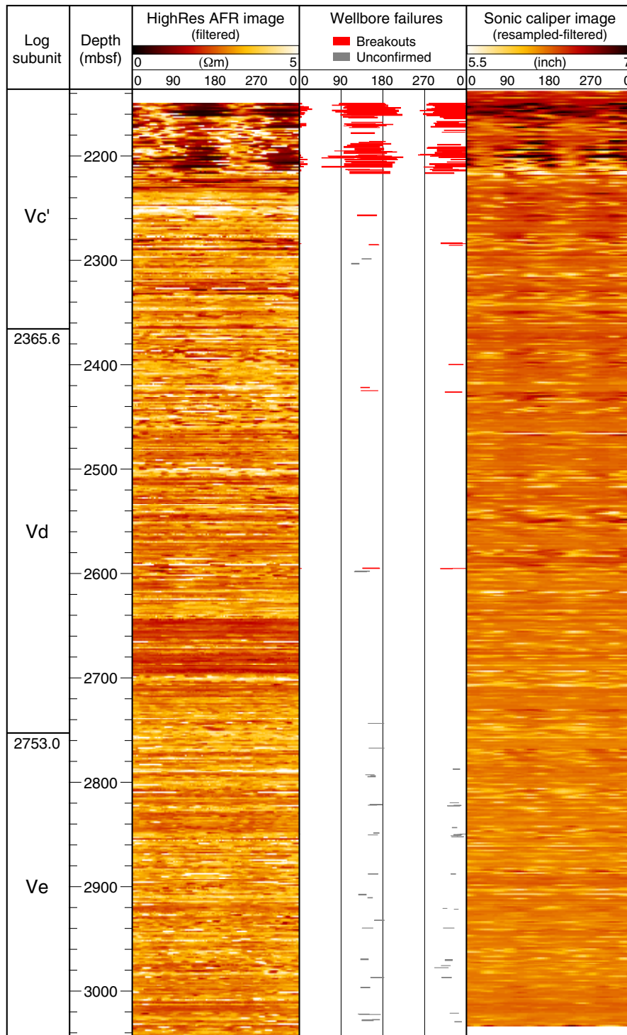
Figure F22. Summary of wellbore failures observed in the resistivity image log shown with the sonic caliper image. AFR = azimuthal focused resistivity.
