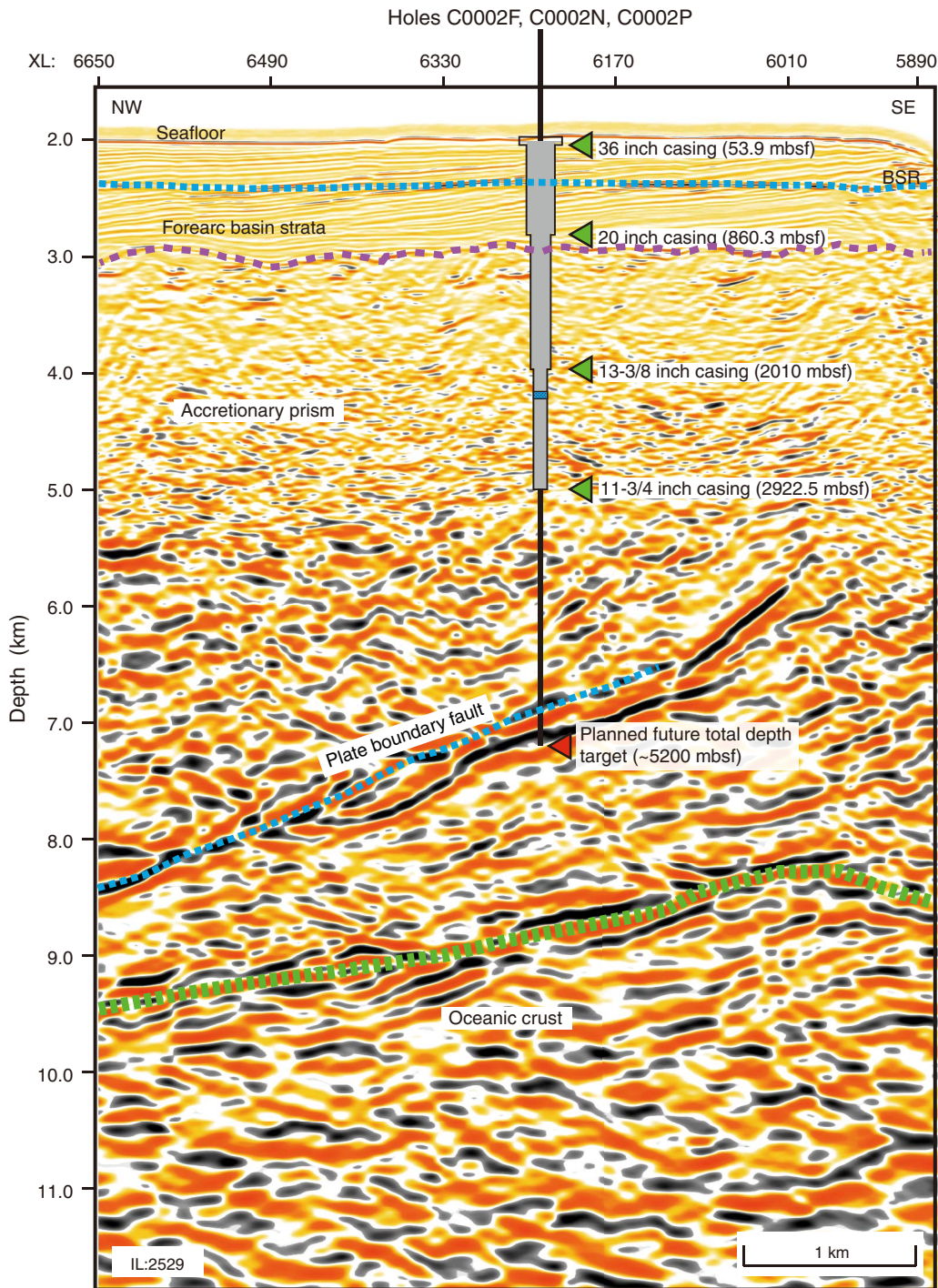
Figure F5. Hole C0002F, C0002N, and C0002P casing and depth schematic overlain on in-line seismic Section 2529 from the prestack depth migrated 3-D seismic volume. The horizontal scale does not allow display of the small (<10 m) Hole C0002N and C0002P sidetrack offsets. The black line represents the borehole, with the final target (red arrowhead) intersecting the plate boundary fault (blue dashed lines). The bottom simulating reflector (BSR) is shown by the opaque blue dashed line. The boundary between forearc basin sediment and accretionary prism is represented by the dashed purple line. The black outlined gray box indicates the current borehole, with casing depths indicated by the green arrowheads. The blue stippled box indicates the cored section of Hole C0002P.
