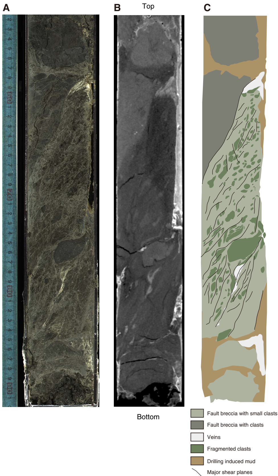
Figure F9. Part of the fault zone in cores retrieved from Hole C0002P (2205.22–2205.56 mbsf). A. Core sample (working half). B. X-ray computed tomography imaging of core sample. C. Sketch of the fault zone.
