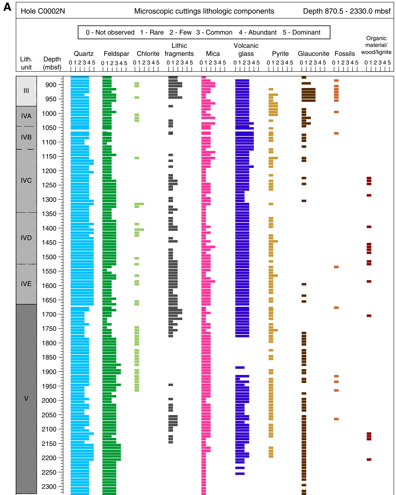
Figure F6. Visual estimation of lithologic composition of cuttings, sampled every 5 m, with associated lithologic unit designations. A. Hole C0002N. (Continued on next two pages.)
