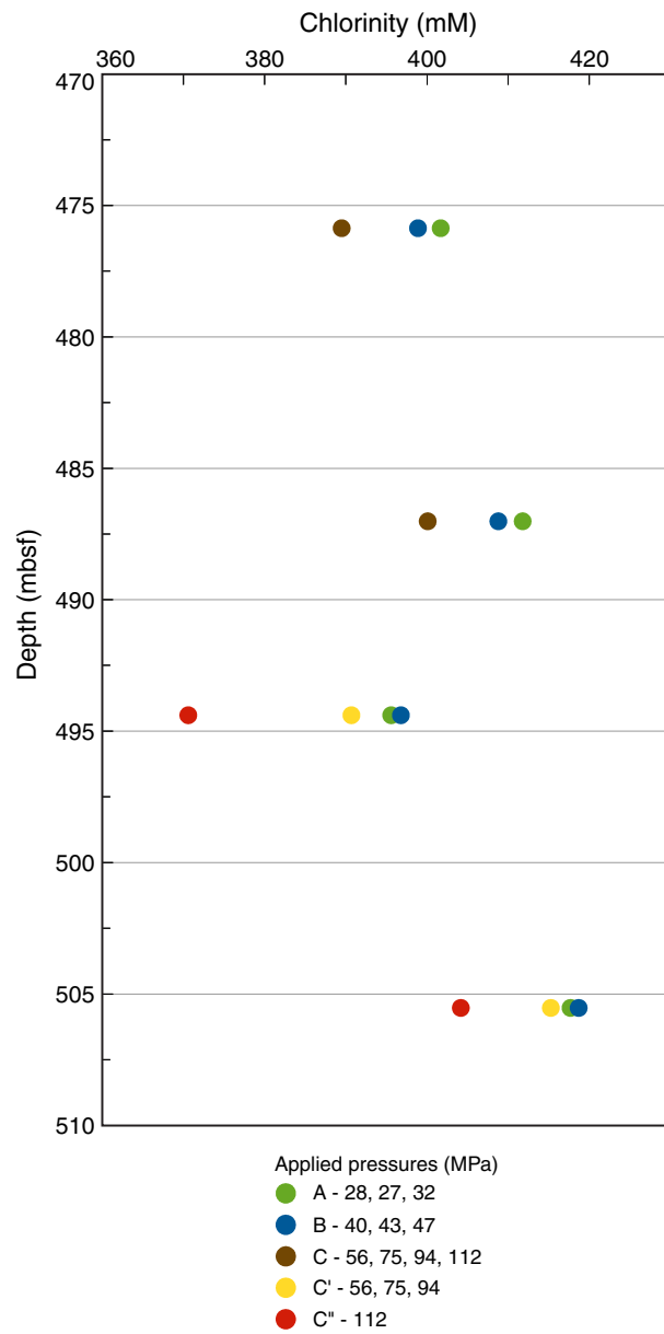
Figure F13. Chlorinity, Hole C0002M. Measured chlorinity values for different squeezing pressure steps are shown. Data represent separate water aliquots from sequential squeeze steps.
