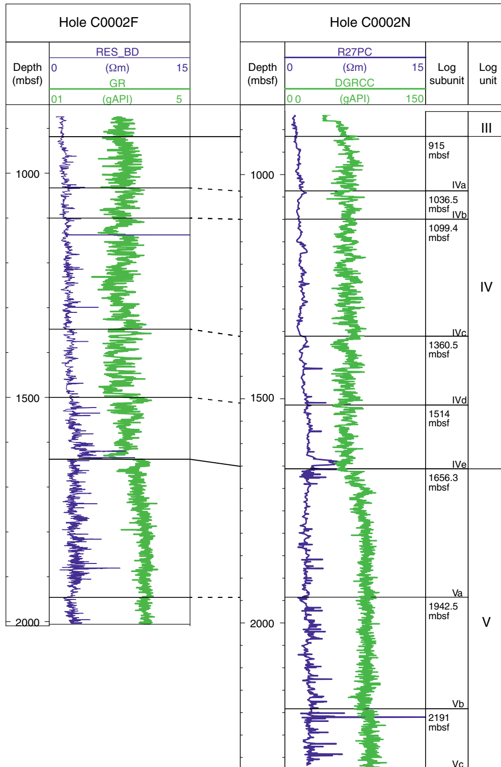
Figure F19. Correlation of log units and subunits between Holes C0002F and C0002N. Log units and subunits defined in Hole C0002F were correlated to Hole C0002N based on the gamma ray and resistivity log response in Hole C0002N. The definition and characterization of units and subunits in Hole C0002F is based on a more complete data set including resistivity images and acoustic logs. Major boundaries and changes in trend or character were identified and correlated. Gamma ray values in Hole C0002N are higher throughout, which may be an artifact (see text for discussion of data quality). RES_BD = resistivity, GR = gamma radiation, R27PC = deep resistivity, DGRCC = dual gamma ray.
