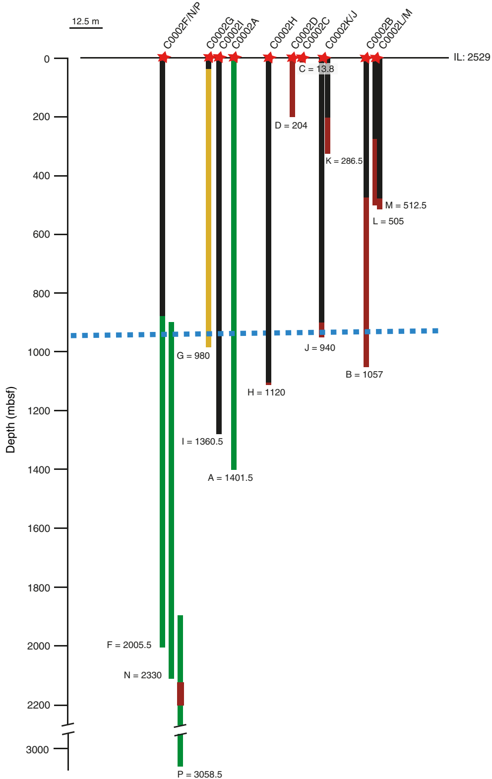
Figure F3. Summary diagram of all drilling and coring at Site C0002. Cored sections are indicated by the brown lines, yellow indicates the observatory, green indicates logging-while-drilling sections, and black indicates sections that were drilled without any sampling. The transect for these holes follows in-line seismic Section 2529. The blue dashed line schematically indicates the approximate upper limit of the accretionary prism.
