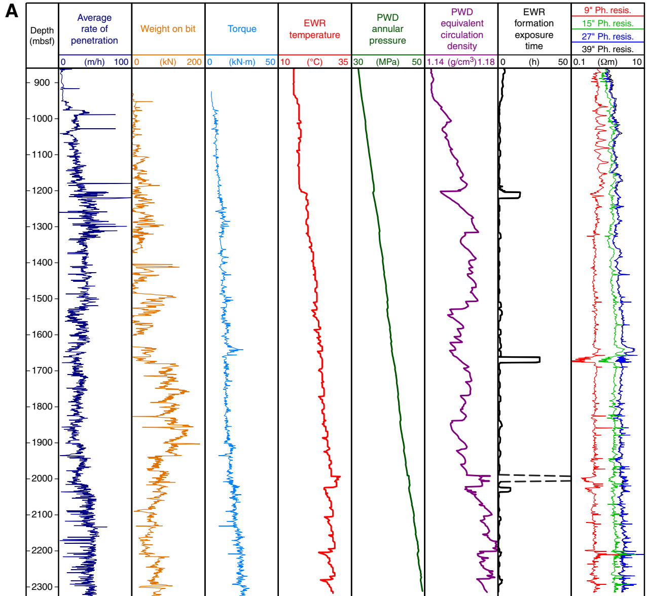
Figure F17. Drilling parameters and selected logs, Holes C0002N and C0002P. EWR = electromagnetic wave resistivity tool, PWD = pressure while drilling, Ph. Resis. = phase resistivity. A. Hole C0002N. Exposure time data drawn with dashed lines at ~2000 mbsf was reconstructed because data were not recorded during the changeover from Run 1 to Run 2. (Continued on next page.)
