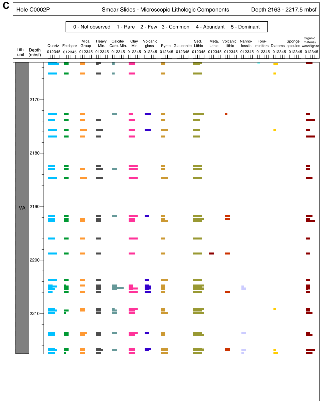
Figure F6 (continued). C. Hole C0002P coring interval smear slides.
