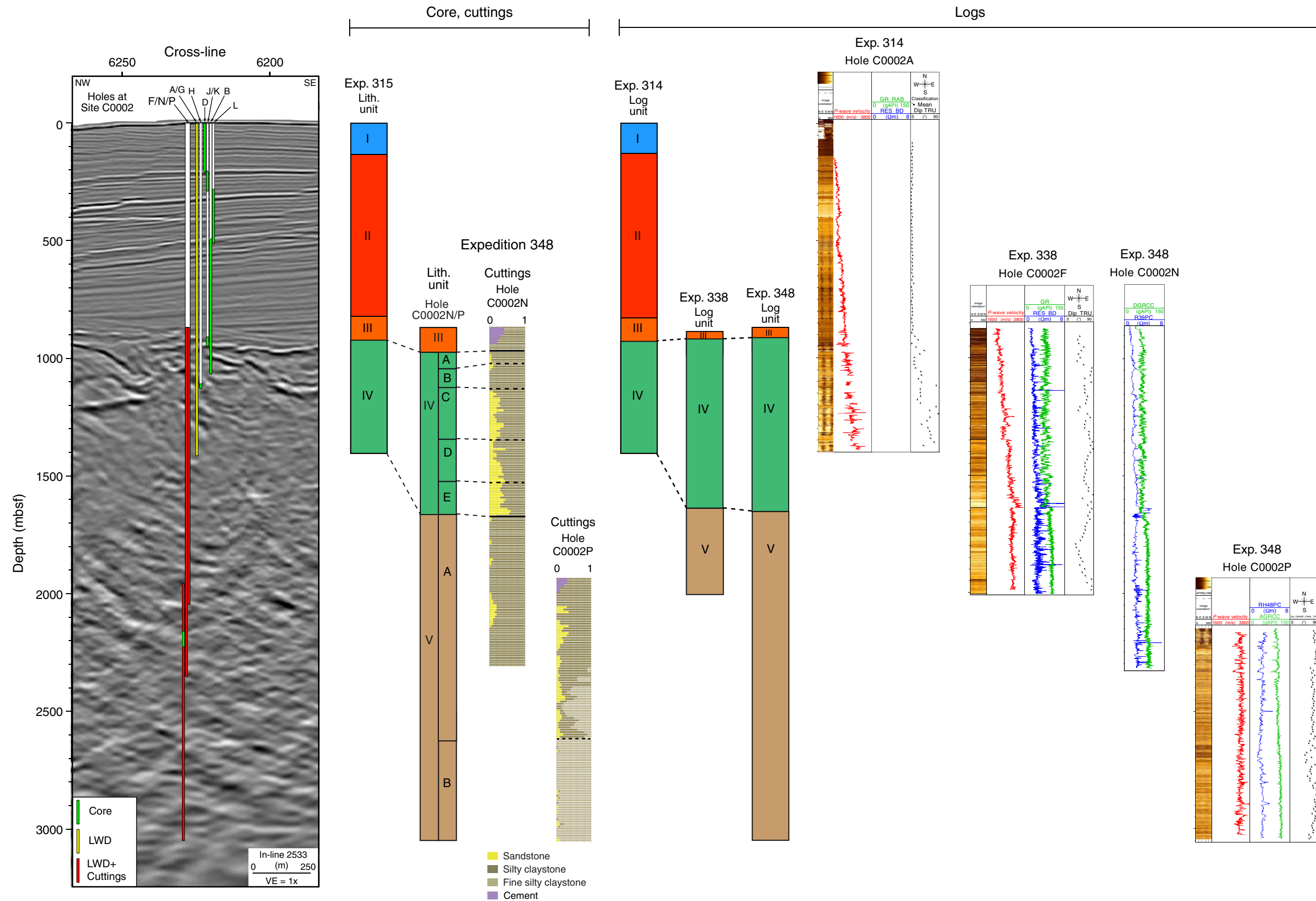
Figure F4. Composite summary plot of data from multiple expeditions and phases of drilling at Site C0002. Resistivity image and logging-while-drilling logs are from Holes C0002F, C0002N, and C0002P. Logging and lithologic unit boundaries are from Expeditions 315, 338, and 348. Percent ratios of cuttings samples from Holes C0002N and C0002P are also shown.
