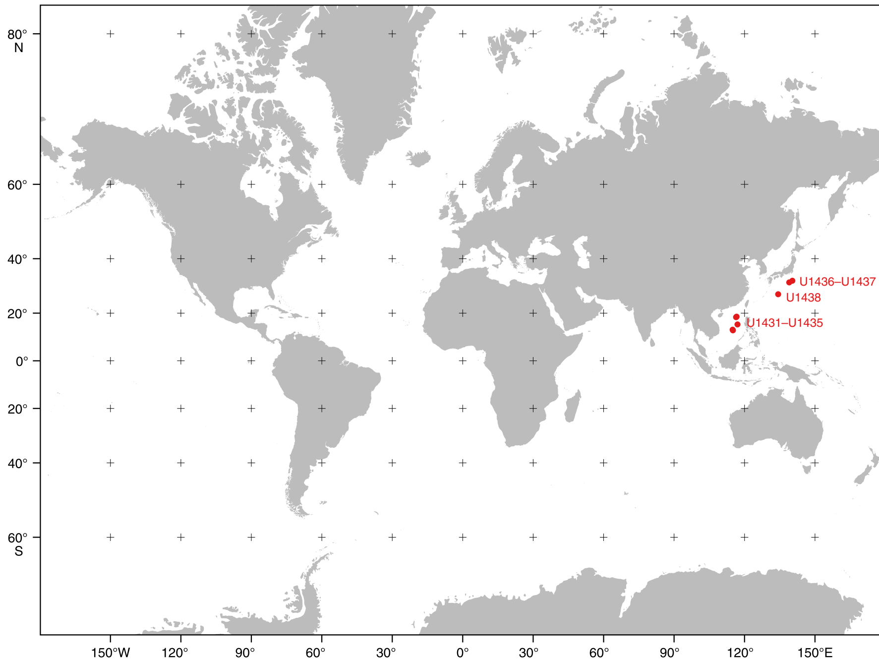
IODP Expedition 349-351, Sites U1431-U1438 (●)
