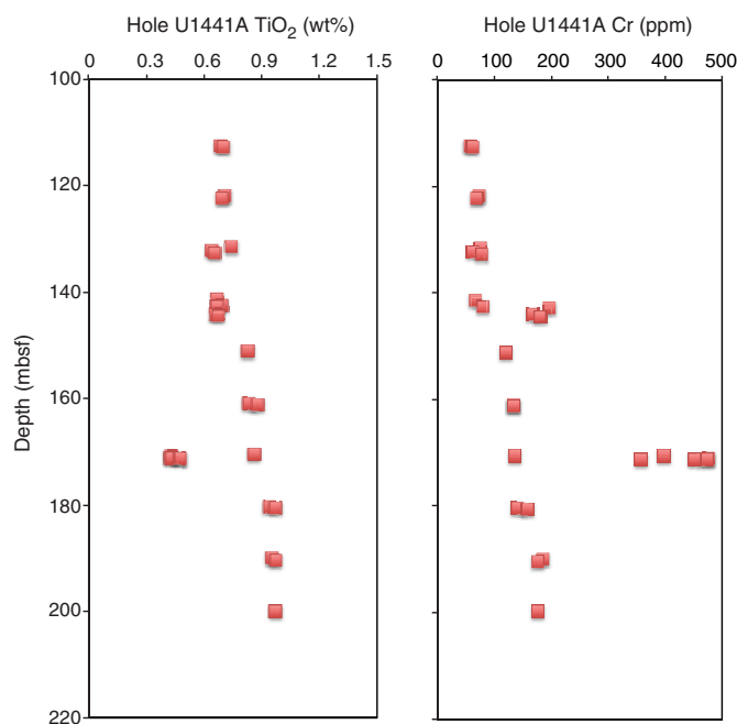
Figure F23. Concentrations of TiO 2 and Cr with depth, Hole U1441A.
