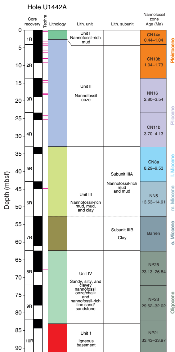
Figure F18. Lithostratigraphic sediment units and ages based on biostratigraphy.
