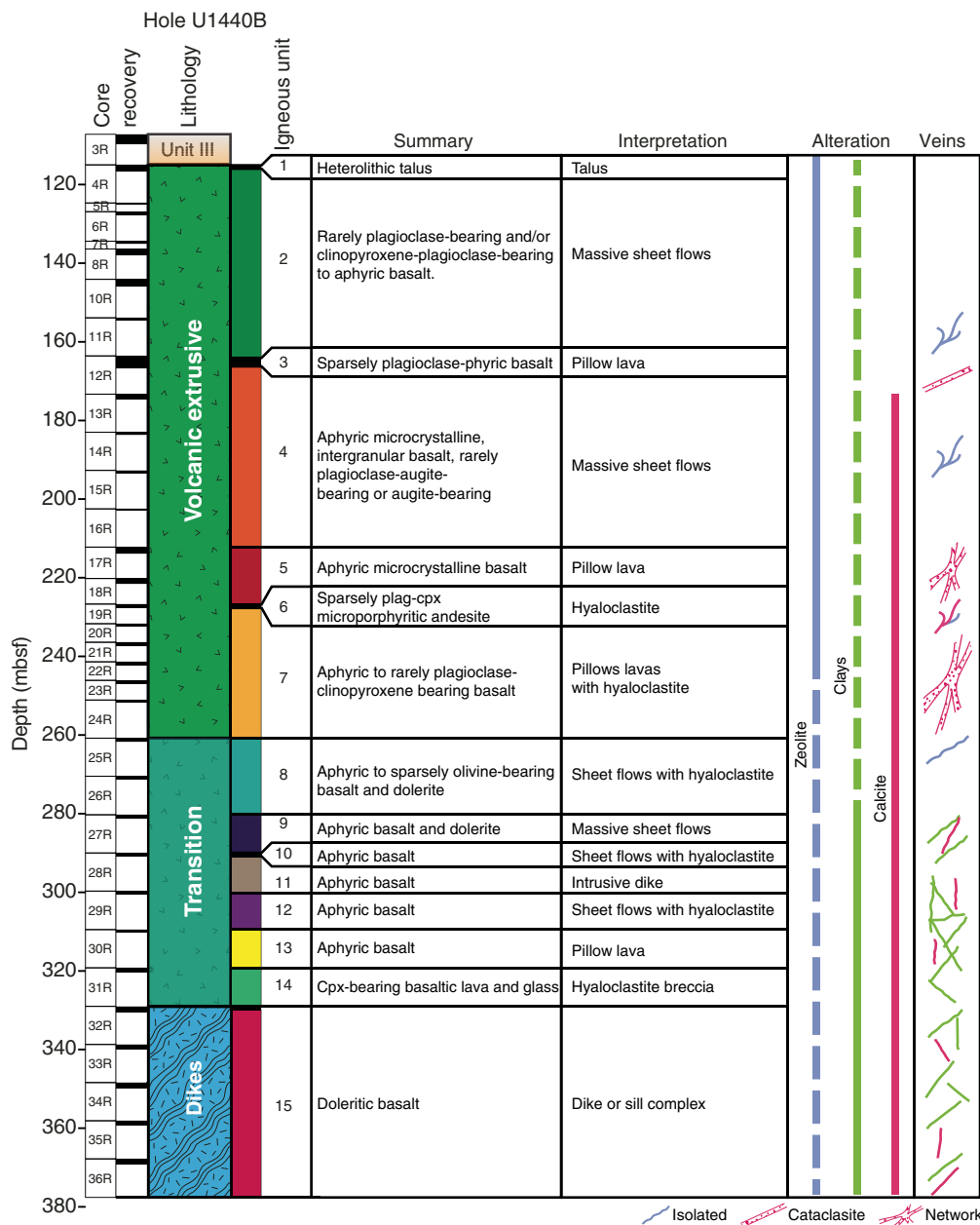
Figure F14. Lithostratigraphic igneous units.
