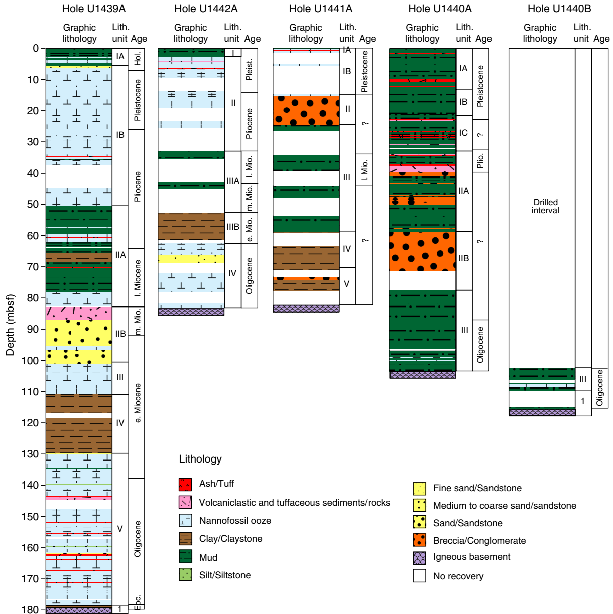
Figure F25. Summary of sedimentary sections. Eocene to Holocene sediment shows typical pelagic carbonates. They are variably influenced by local and regional volcanism, leading to the alternating sequences of volcanoclastic-rich and nannofossil-pure lithologic units.
