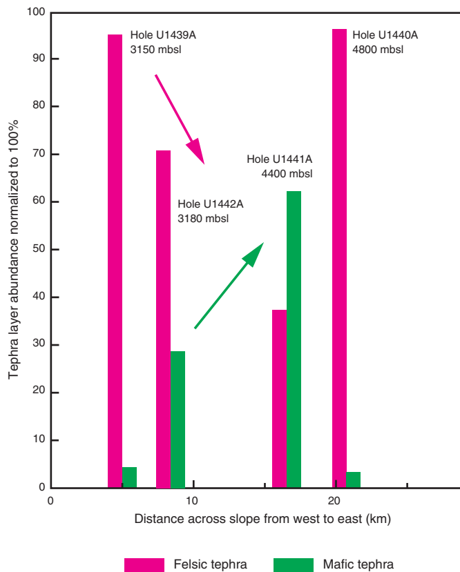
Figure F26. Normalized ash abundance, Sites U1439–U1442. Note different amounts of felsic and mafic ash layers across the slope. Arrows mark the decrease and increase of felsic and mafic tephra, respectively.
