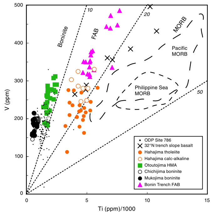
Figure F4. V-Ti systematics (Shervais, 1982) for the lavas erupted following subduction initiation. Note that the earliest lavas to erupt following subduction initiation are distinct from MORB and from later boninites. These are, however, isolated outcrops. Plot taken from Ishizuka et al. (2006, 2011).
