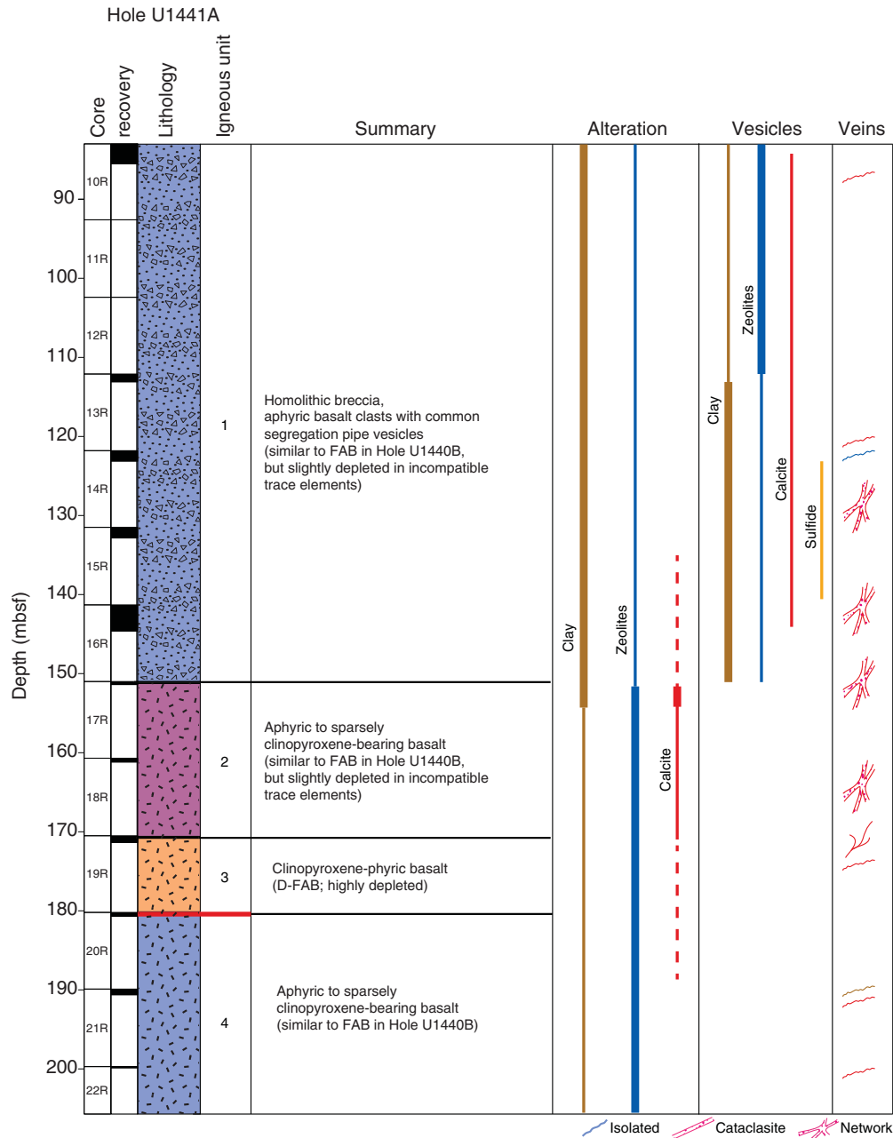
Figure F16. Lithostratigraphic igneous units.
