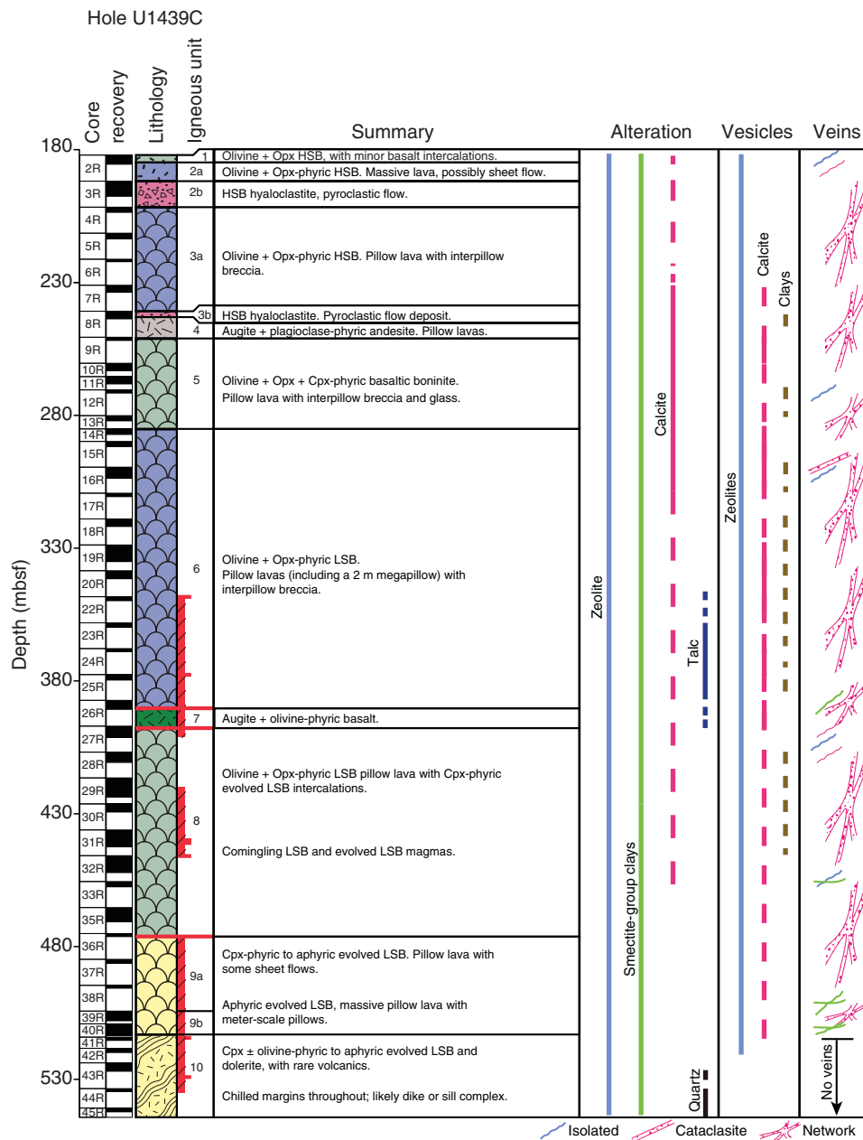
Figure F12. Lithostratigraphic igneous units. Red hatched bars adjacent to lithology column represent fault zones. HSB = high-silica boninite, LSB = low-silica boninite.
