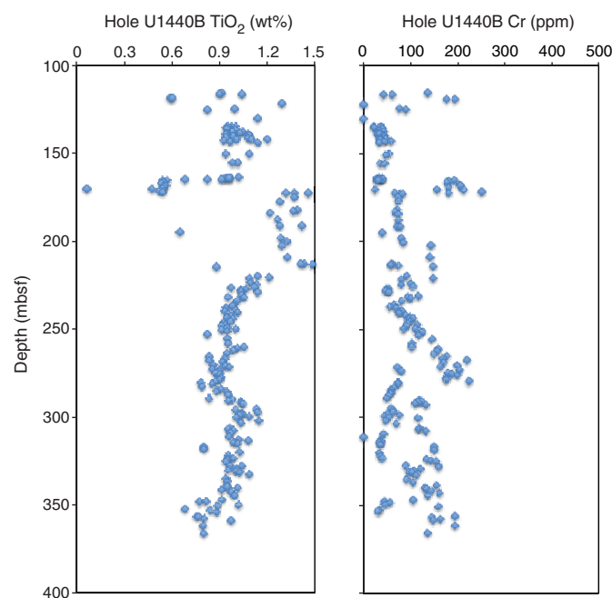
Figure F22. Concentrations of TiO 2 and Cr with depth, Hole U1440B.
