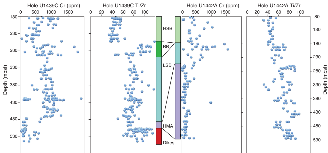
Figure F24. Cr concentrations and Ti/Zr ratios with depth. The central colored bars represent our stratigraphic correlation between these two holes (see text for further explanation). BB = basaltic boninite.
