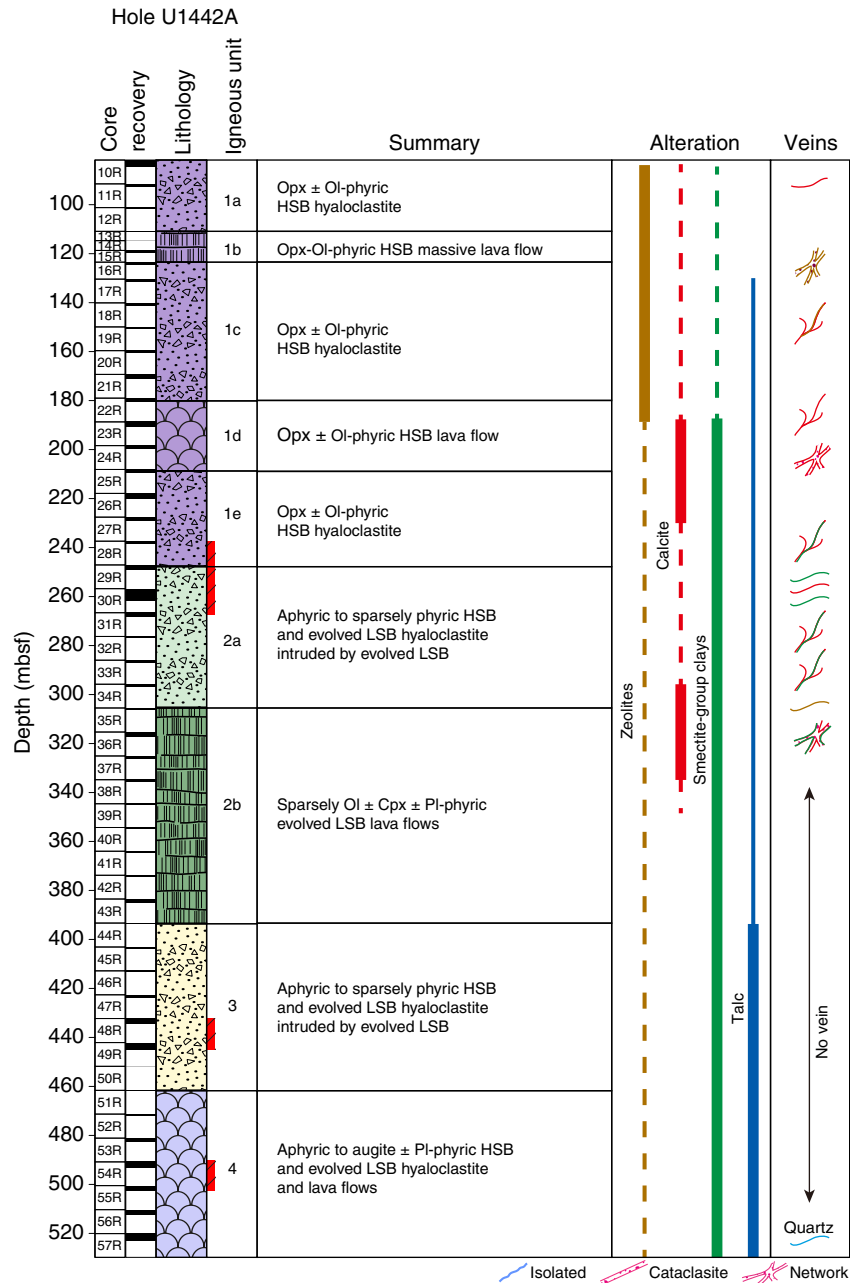
Figure F17. Lithostratigraphic igneous units. Red hatched bars adjacent to lithology column represent fault zones. Opx = orthopyroxene, Ol = olivine, Cpx = clinopyroxene, Pl = plagioclase.
