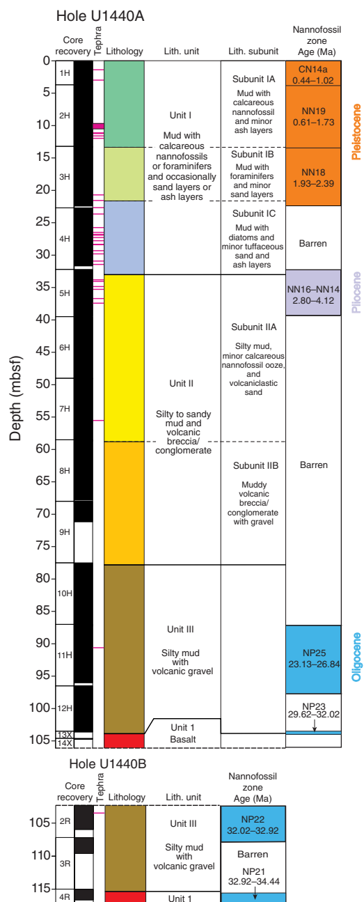
Figure F13. Lithostratigraphic sediment units and ages based on biostratigraphy.
