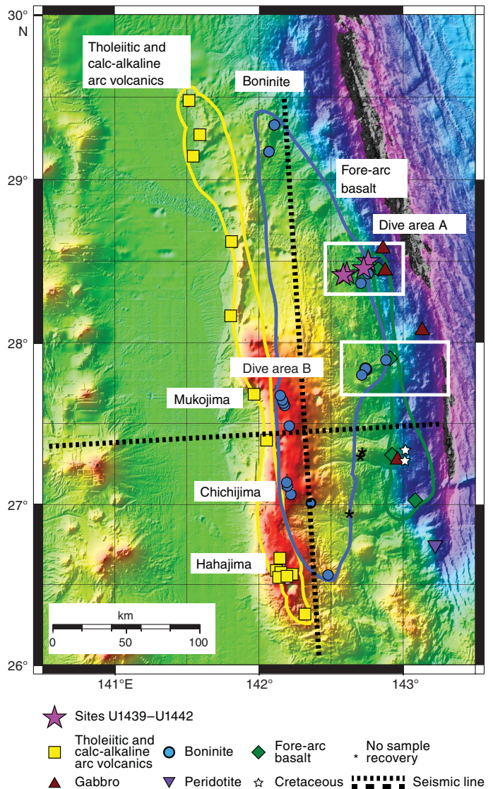
Figure F9. Rock types recovered from dredging and diving expeditions to the Bonin fore arc, showing its ophiolitic structure (after Ishizuka et al., 2011). Stars = Sites U1439–U1442, boxes = areas chosen for more detailed site survey dives.
