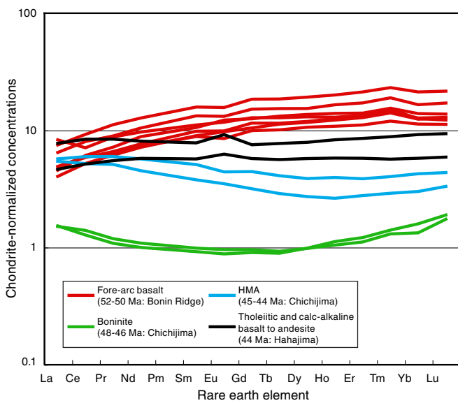
Figure F3. Variations in REE patterns in the Bonin fore arc following subduction initiation. Note the recently discovered MORB-like patterns of the first volcanic products, the fore-arc basalt, and the contrast with the later U-shaped boninite patterns. Expedition 352 research will obtain complete information on gradations within and between these units. Plot taken from Ishizuka et al. (2006, 2011).
