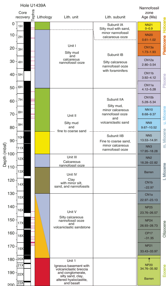
Figure F11. Lithostratigraphic sediment units and ages based on biostratigraphy.
