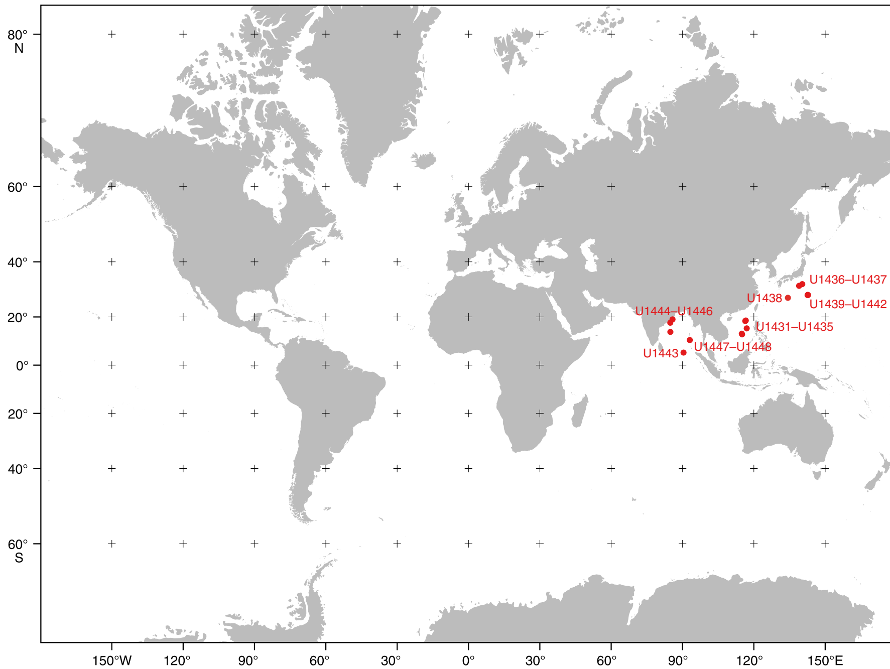
IODP Expedition 349-353, Sites U1431-U1448 (●)
