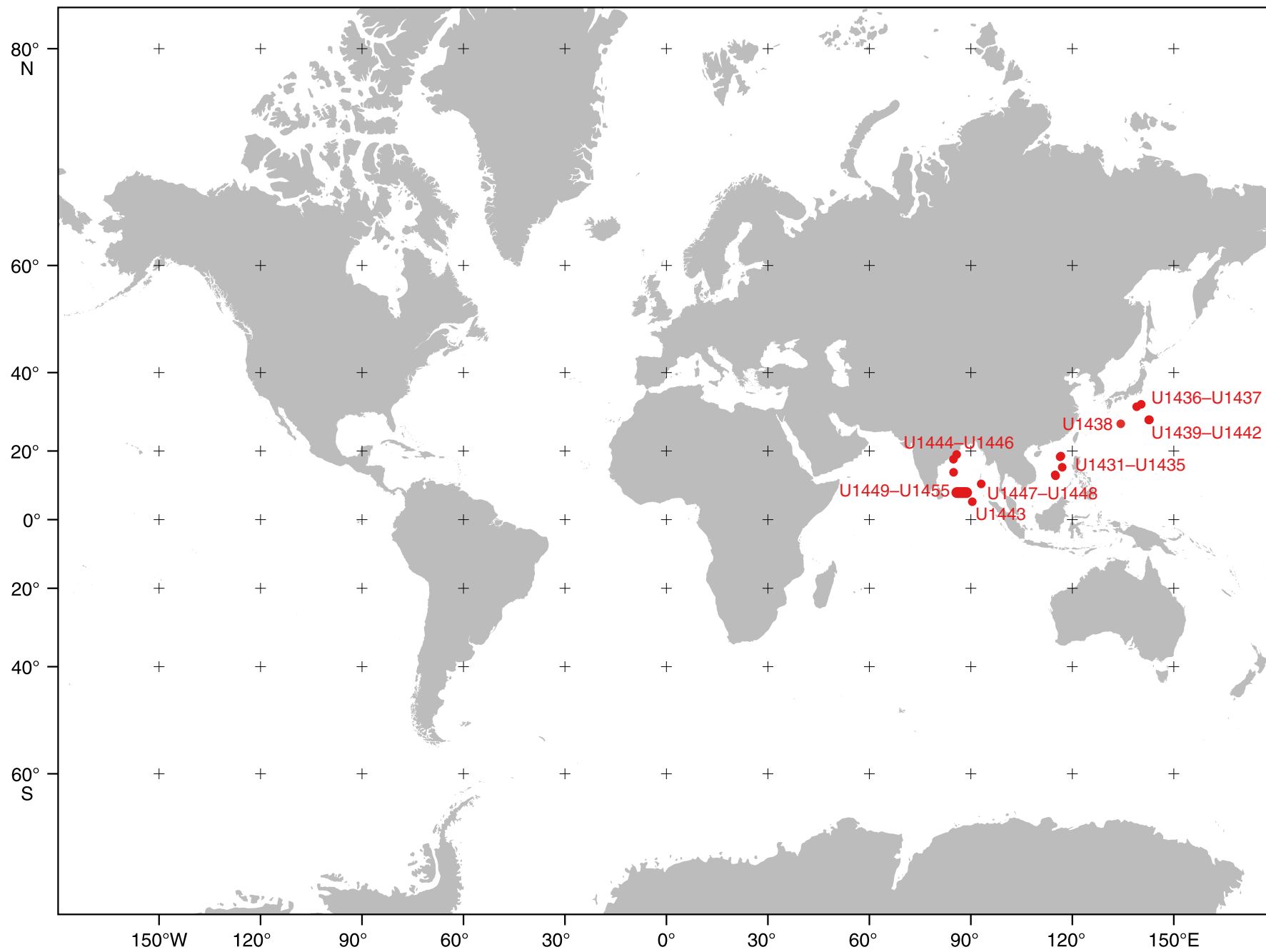
IODP Expeditions 349-354, Sites U1431-U1455 (●)
