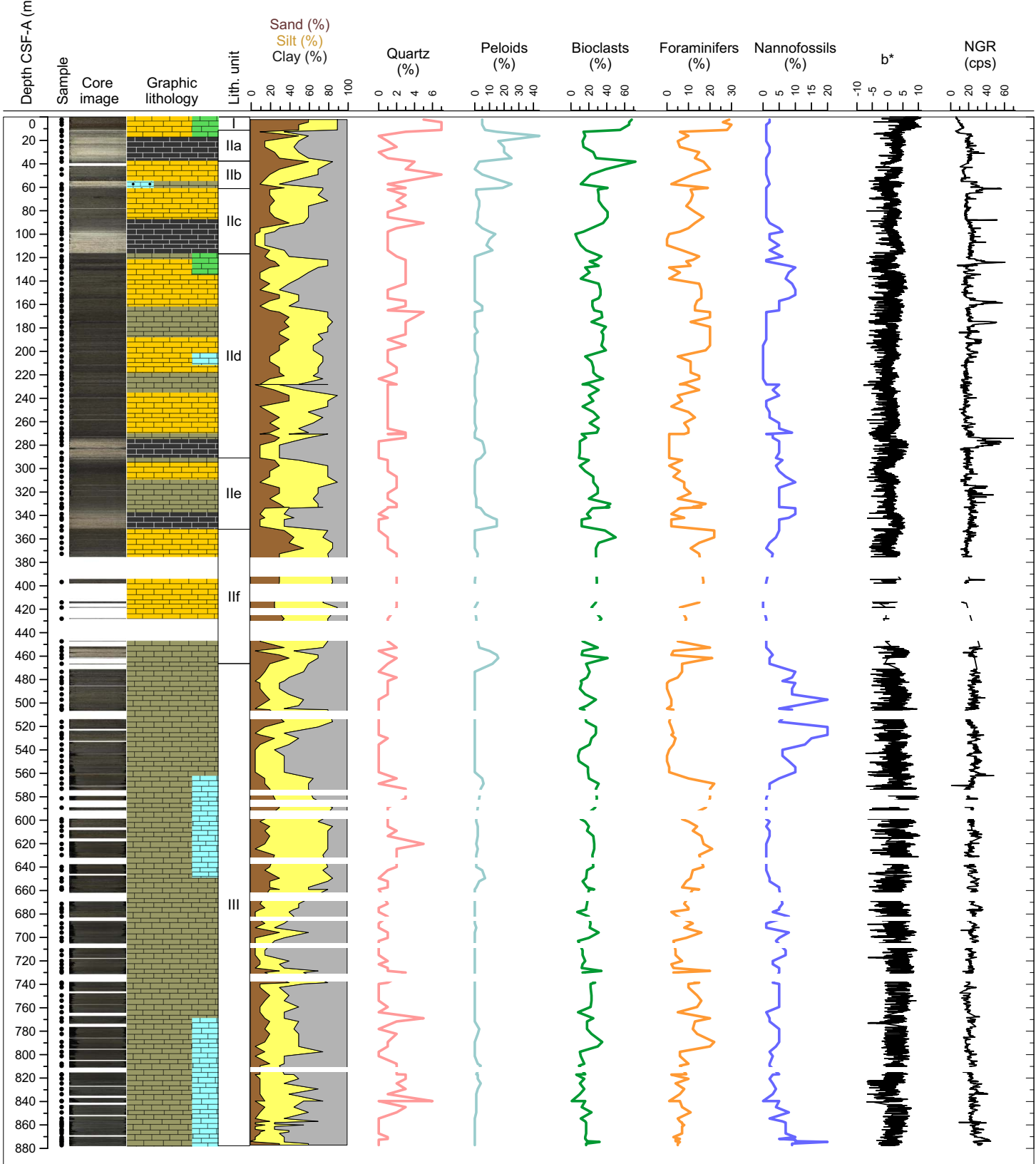
U1461_C_litho_Supplement2_SmearData_U1461B
