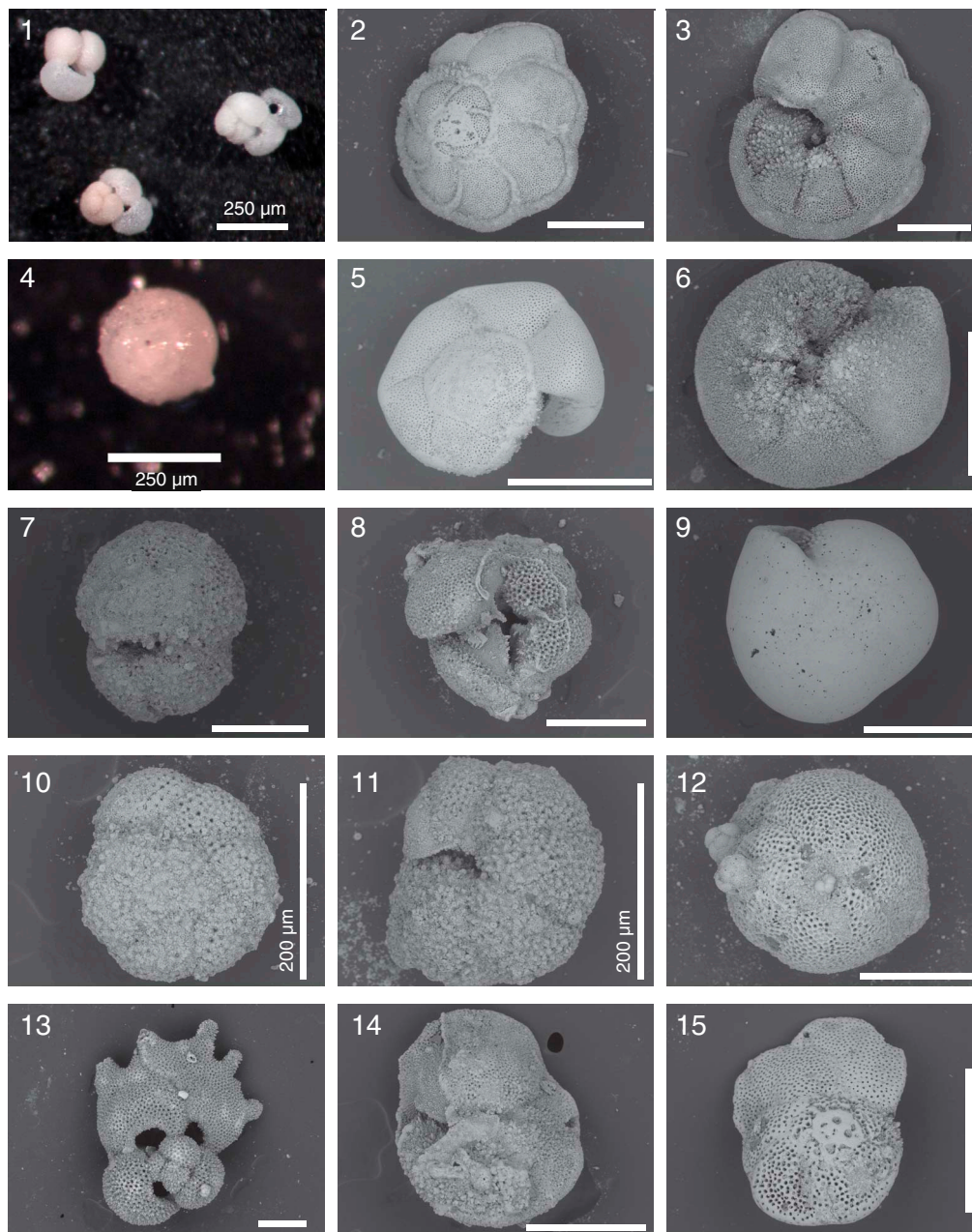
Figure F26. Plate of selected planktonic foraminifers, Site U1466. 1. Globigerinoides ruber pink (two specimens on the left) and white (one specimen on the right). 2, 3. Globorotalia limbata . 4. Orbulina suturalis . 5, 6. Globorotalia truncatulinoides . 7. Praeorbulina sicana . 8. Dentoglobigerina altispira . 9. Pulleniatina obliquiloculata . 10, 11. Paragloborotalia kugleri . 12. Globigerinatella insueta . 13. Globigerinoides fistulosus . 14, 15. Fohsella fohsi . Scale bars = 250 \mu\text{m} , except where otherwise indicated.
