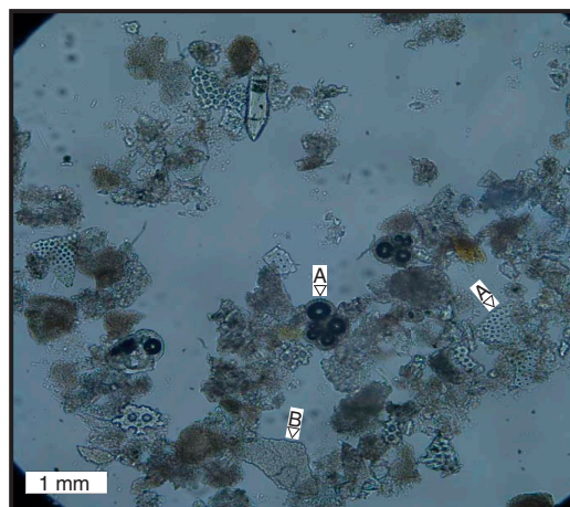
Figure F5. A = planktonic foraminiferal debris, B = pteropod fragments (359-U1466A-6H-CC; 52.25 mbsf).
