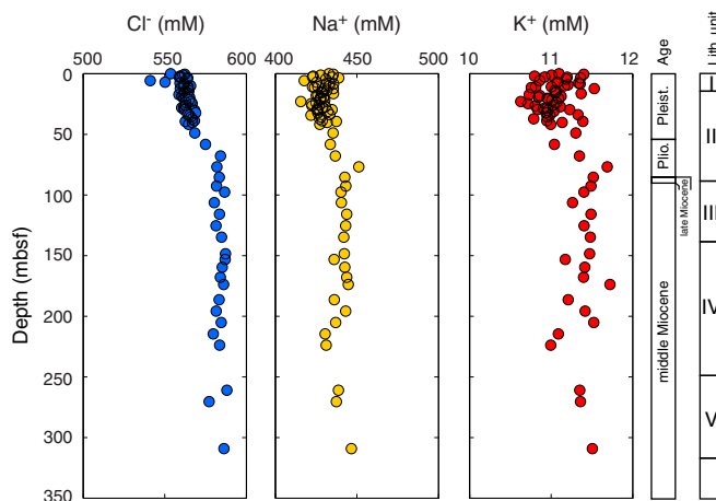
Figure F31. IW Cl - , Na + , and K + concentrations, Holes U1466A and U1466B.
