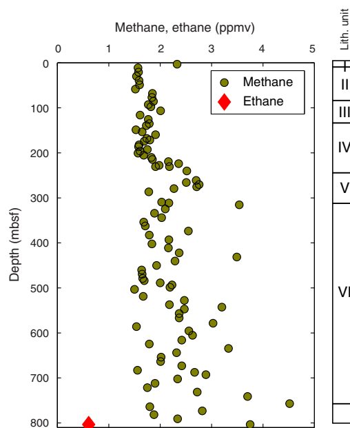
Figure F39. Headspace methane and ethane concentrations, Site U1466.
