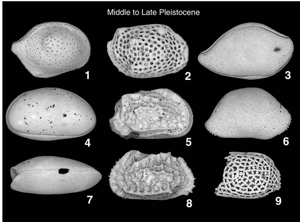
Figure F27. Plate of Middle to Late Pleistocene ostracods, Site U1466. 1. Loxococoncha cf. pulchra McKenzie, 1967. 2. Loxocorniculum sp. 3. Neonesidea sp. A. 4. Xestoleberis sp. 5. Bosasella elongata (Hu, 1979). 6. Paranesidea sp. B. 7. Krithe sp. 8. Bradleya sp. 9. Pistocythereis sp.
