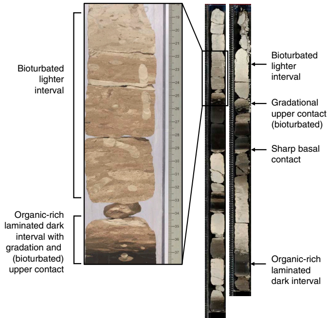
Figure F20. Alternation of black organic-rich and white chalk alternation in Subunit VIIB (359-U1446B-56R-1 [top = 789.60 mbsf] and 56R-2).
