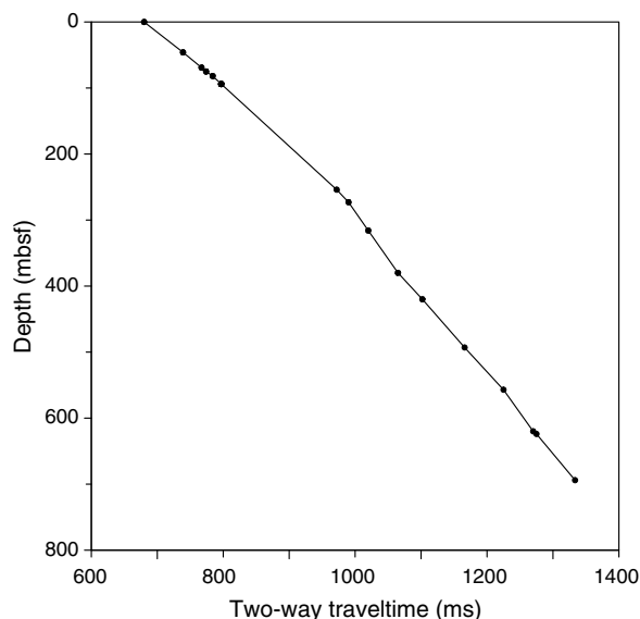
Figure F57. Time-depth conversion, Site U1466.
