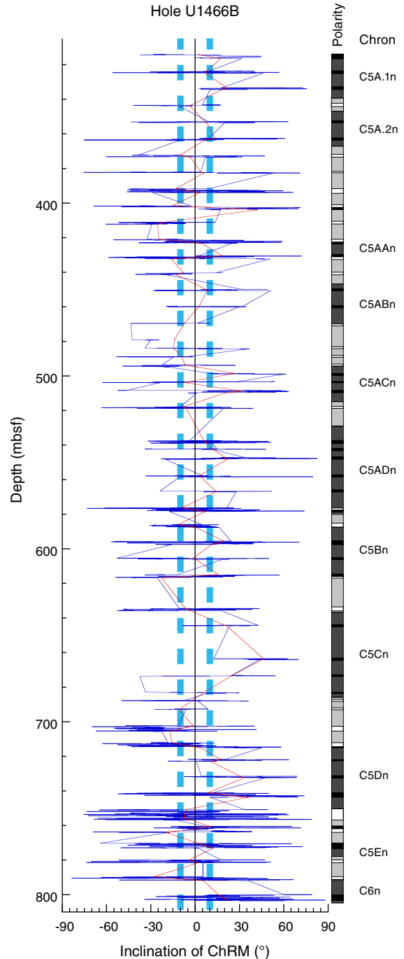
Figure F47. Inclination of ChRM and magnetostratigraphy, Hole U1466B. Polarity: black = normal, white = reversed, dark gray boxes = possible normal chrons, light gray = possible reversal chrons. The chron boundary could not be defined precisely due to the absence of sample continuity.
