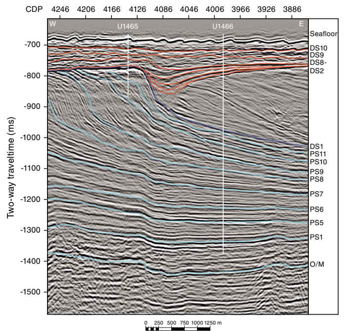
Figure F55. Seismic section of drowned Kardiva platform and onlap and burial by drift sequences, Site U1466. Dark blue line = horizon between platform and drift sequences.
