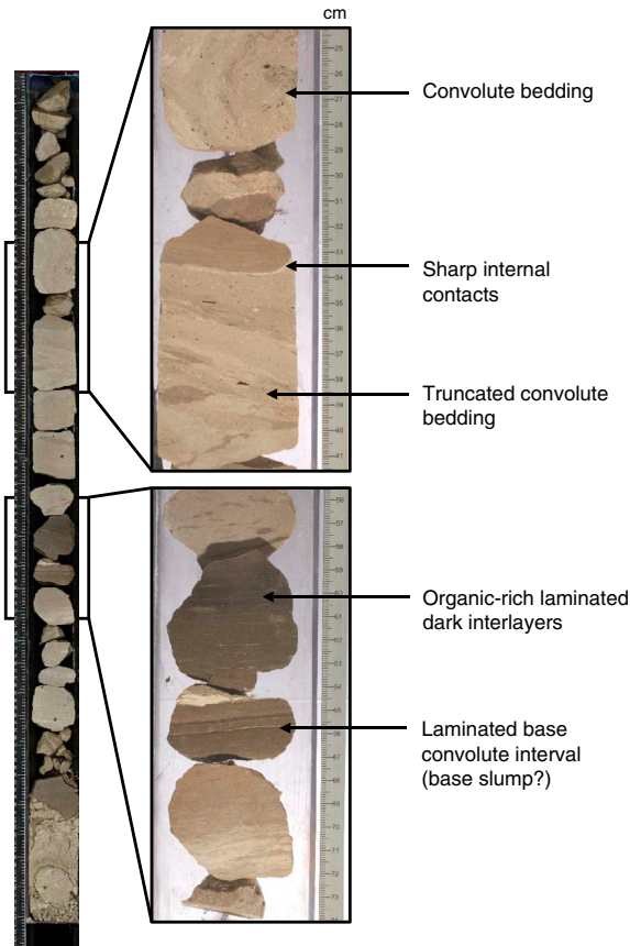
Figure F20. Alternation of black organic-rich and white chalk alternation in Subunit VIIB (359-U1446B-56R-1 [top = 789.60 mbsf] and 56R-2).
