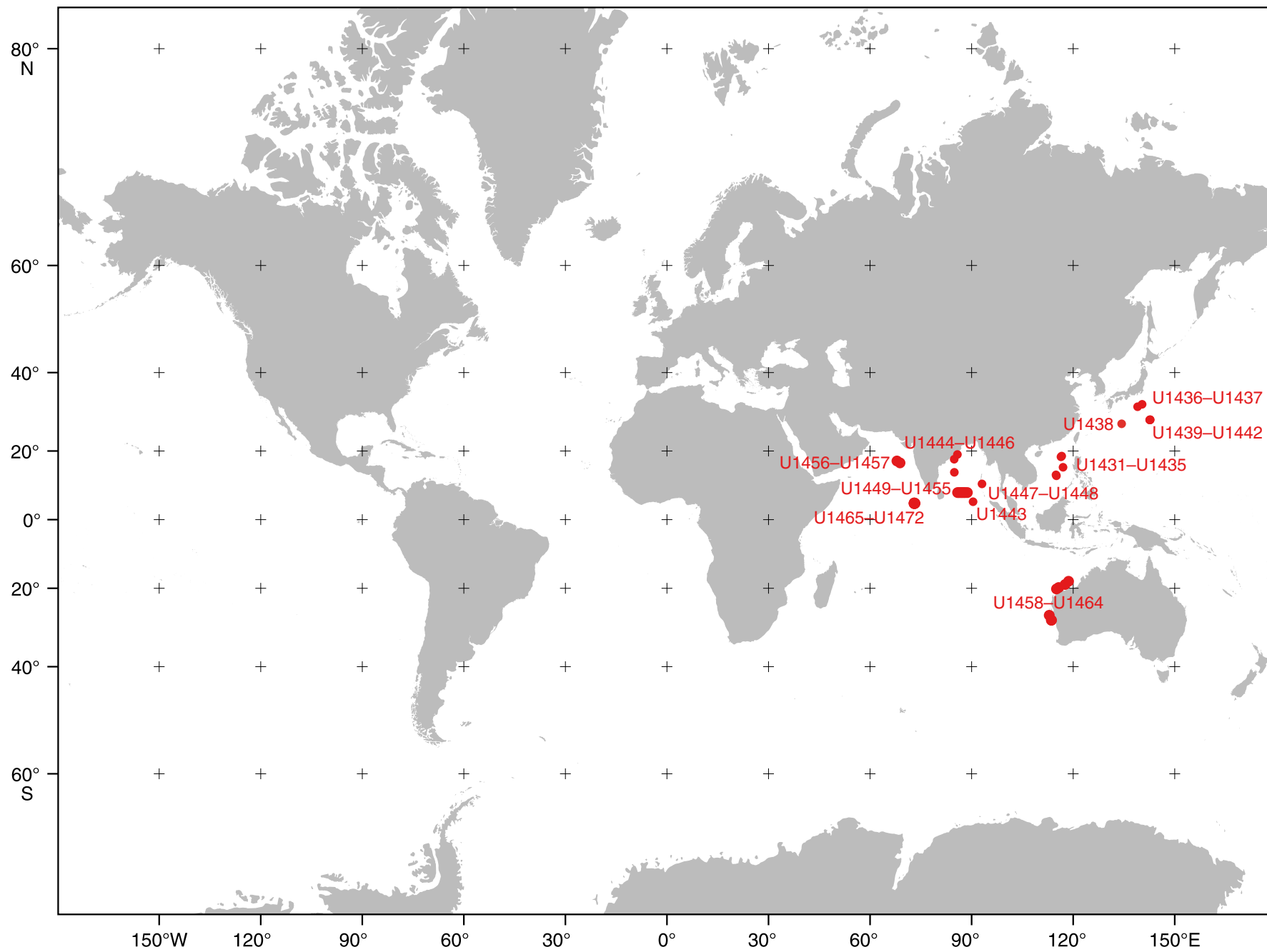
IODP Expeditions 349–356, 359, Sites U1431–U1472 (•)
