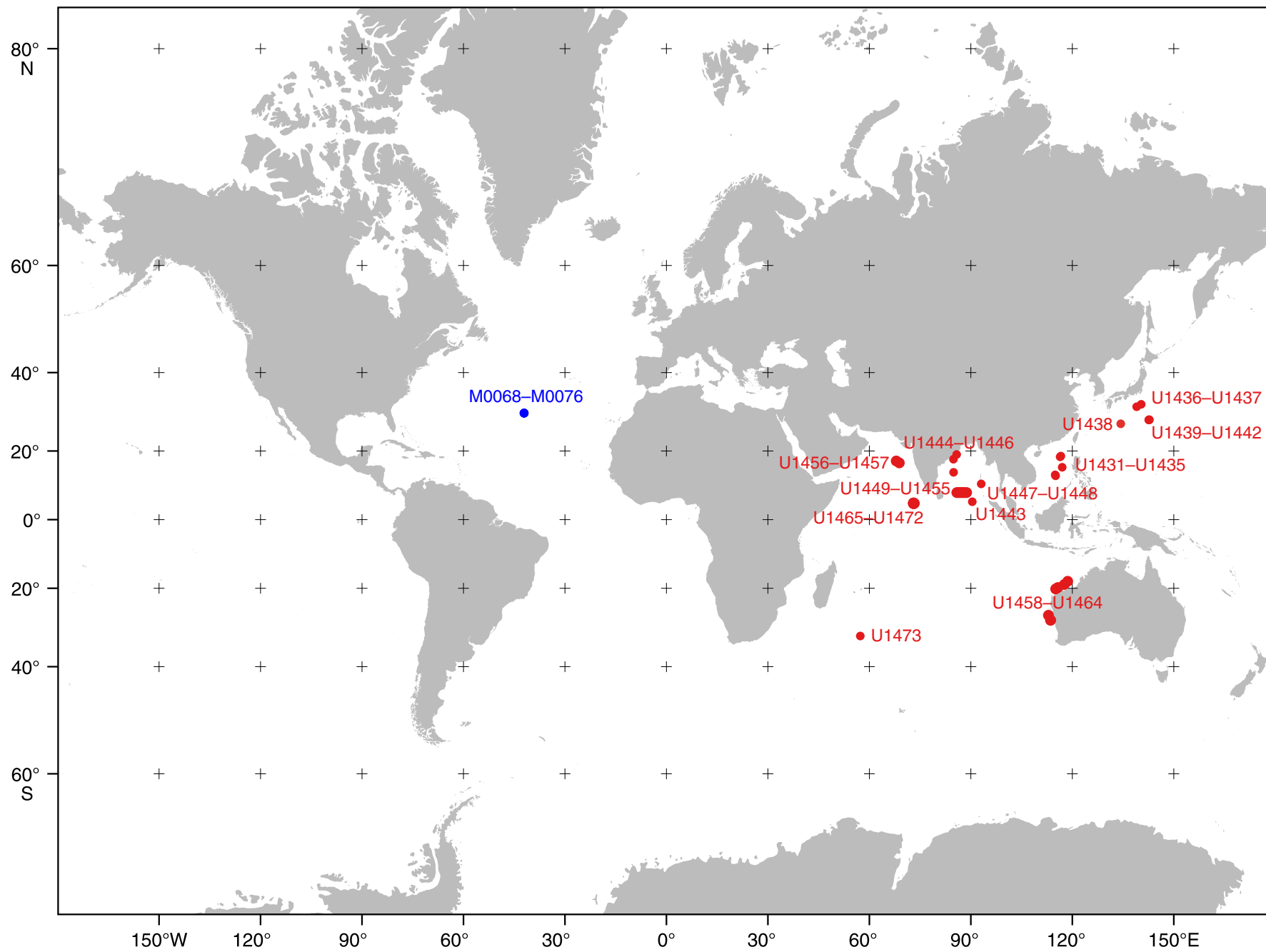
IODP Expeditions 349-357, 359-360, Sites M0068-M0076 (●), U1431-U1473 (●)
