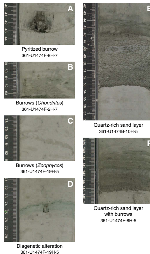
Figure F10. A–F. Representative sedimentary structures and lithologic accessories, Site U1474.
