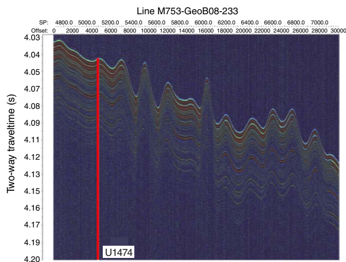
Figure F6. Parasound Line M753-GeoB08-233 showing parallel reflectors at Site U1474. Labels on the vertical axis are chosen to represent \sim 10 m (13.3 ms two-way traveltime).
