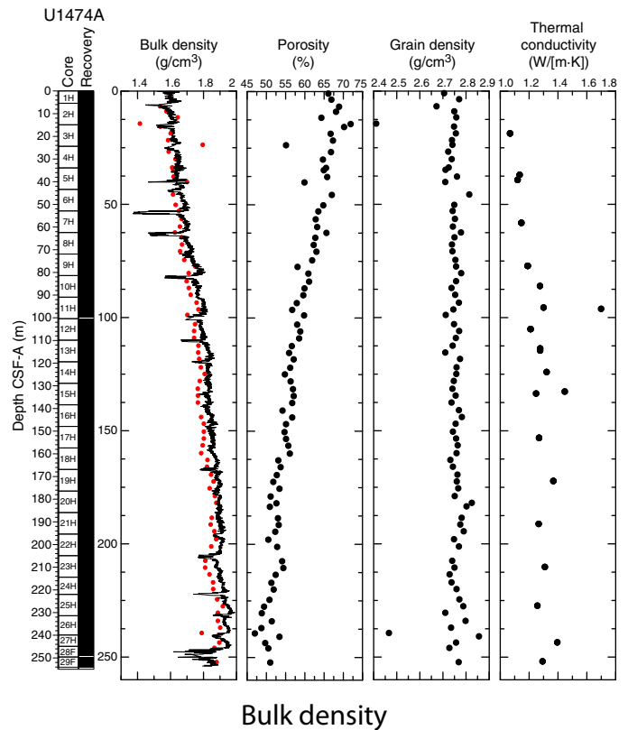
Figure F16. Bulk density (black line = WRMSL measurements, red circles = MAD measurements), porosity, grain density, and thermal conductivity, Hole U1474A.
