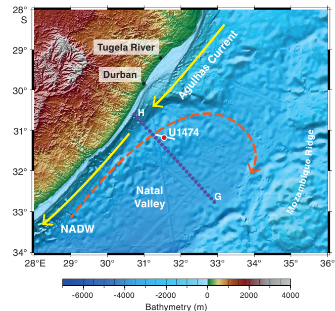
Figure F2. Geomorphologic and oceanographic features near Site U1474. Seismic Line H–G (blue dotted line) of Niemi et al. (2000) is shown in Figure F4. Seismic and parasound lines are shown in Figures F5 and F6, respectively. Seismic line M753–GeoB08–233 is shown as a solid white line. Dashed arrow = bottom water current, solid arrows = main surface currents.
