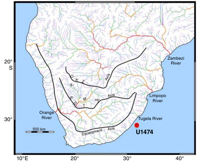
Figure F3. Drainage system of southern Africa adapted from Moore et al. (2009). Colors denote stream rank from 1 (purple) to 5 (red). For reference, Rank 5 streams are considered medium streams in the terminology of Strahler (1952). The major river divides are interpreted by Moore et al. (2009) to reflect epeirogenic uplift axes, progressively younger from inland toward the margin. OKZ = Ovambo-Kalahari-Zimbabwe, EGT = Etosha-Griqualand-Transvaal. M = Molopo River, N = Nossob River, MM = Mahura Muhtla.
