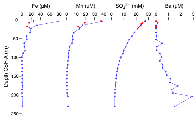
Figure F35. Dissolved iron, manganese, sulfate, and barium profiles, Holes U1474A (blue) and U1474B (red).
