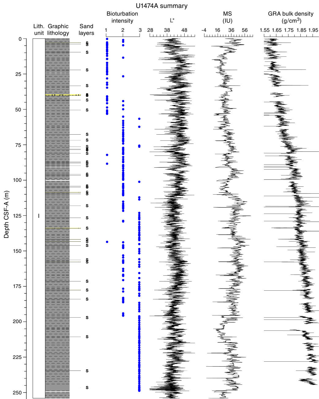
Figure F8. Lithostratigraphic summary with selected physical property and geochemical data. Holes U1474C and U1474H are composed of only one core each and are presented in the visual core descriptions (see Core descriptions ). Bioturbation intensity: 1 = slight, 2 = moderate, 3 = strong. A. Hole U1474A. (Continued on next four pages.)
