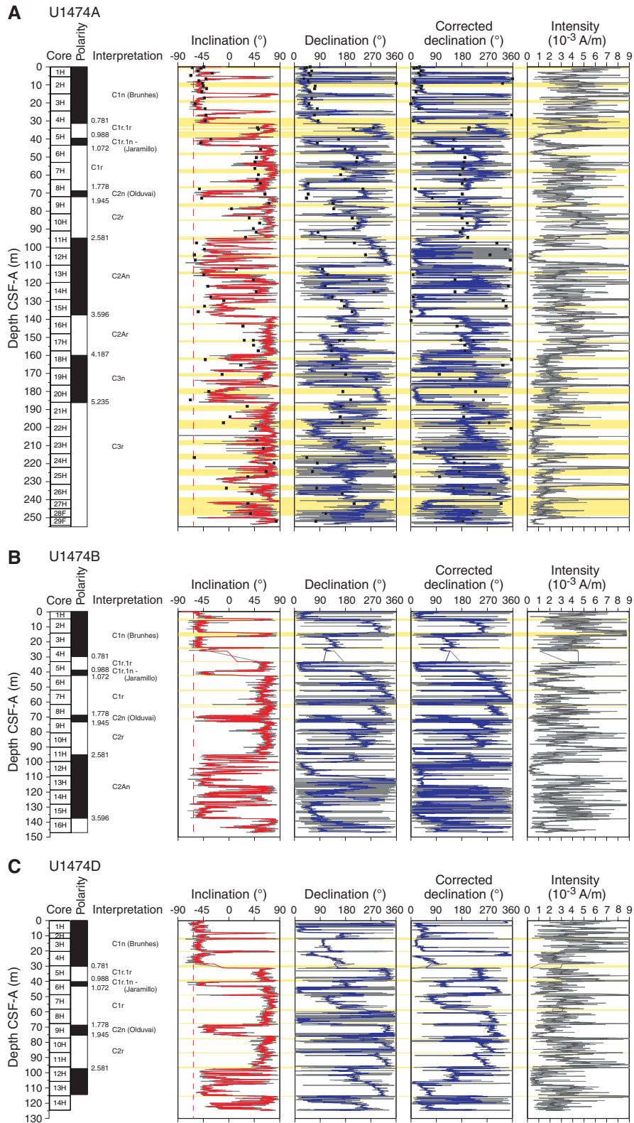
Figure F28. Downhole paleomagnetic results, Site U1474. Inclination, declination, corrected declination, and intensity after 25 mT AF demagnetization are plotted according to their individual CSF-A depth scales. Inclination: gray line = continuous SRM data, red line = 10-point smoothed record, vertical dashed line = present-day inclination. Declination: gray line = data, blue line = 10-point smoothed record, yellow shaded horizontal bars = core disturbance intervals. Polarity chron ages after Gradstein et al. (2012). A. Hole U1474A. Black squares = ChRM obtained by PCA of discrete sample demagnetization data. B. Hole U1474B. C. Hole U1474D. (Continued on next page.)
