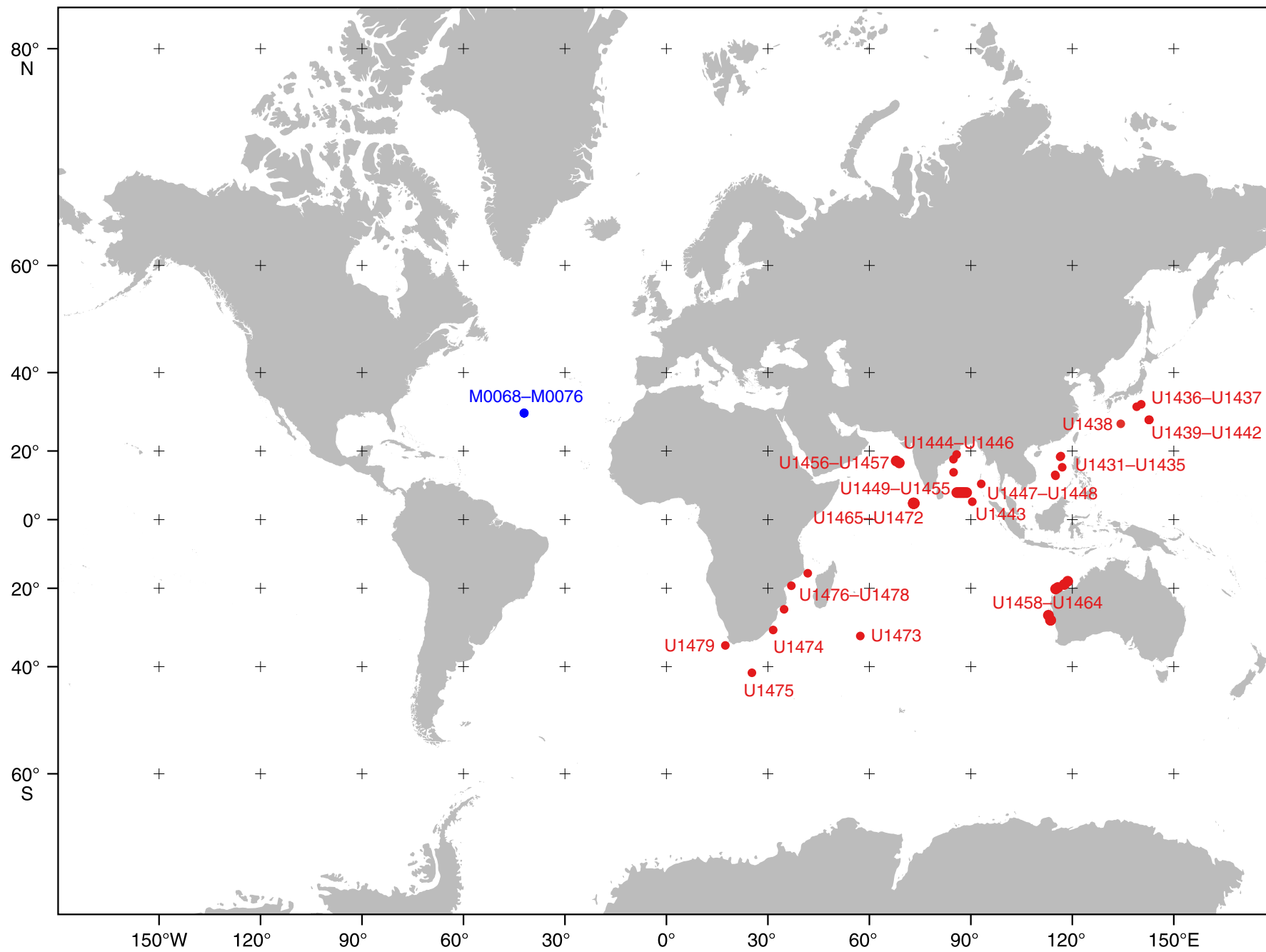
IODP Expeditions 349–357, 359–361, Sites M0068–M0076 (●), U1431–U1479 (●)
