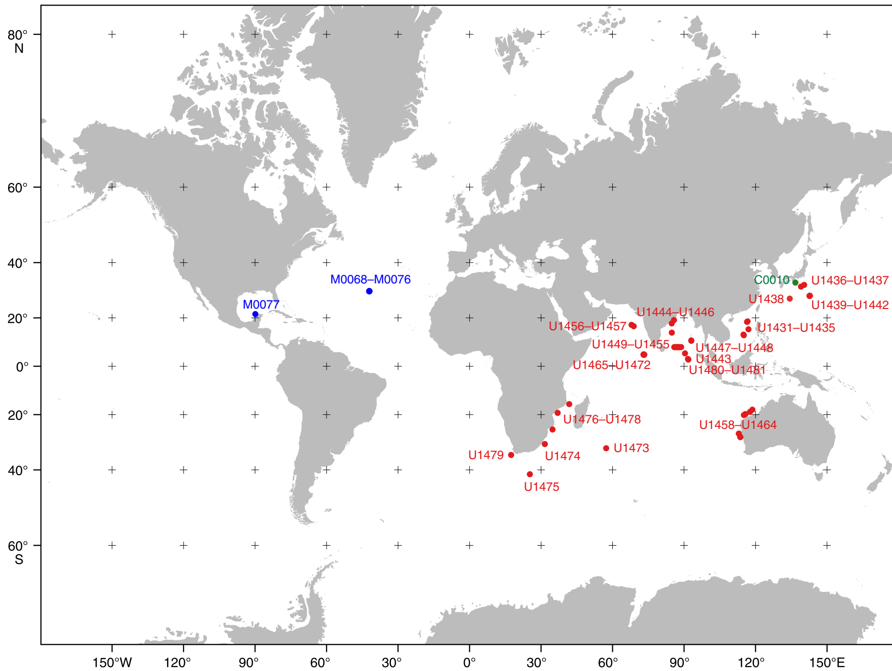
IODP Expeditions 349–357, 359–362, 364–365, Sites C0010 (●), M0068–M0077 (●), U1431–U1481 (●)
