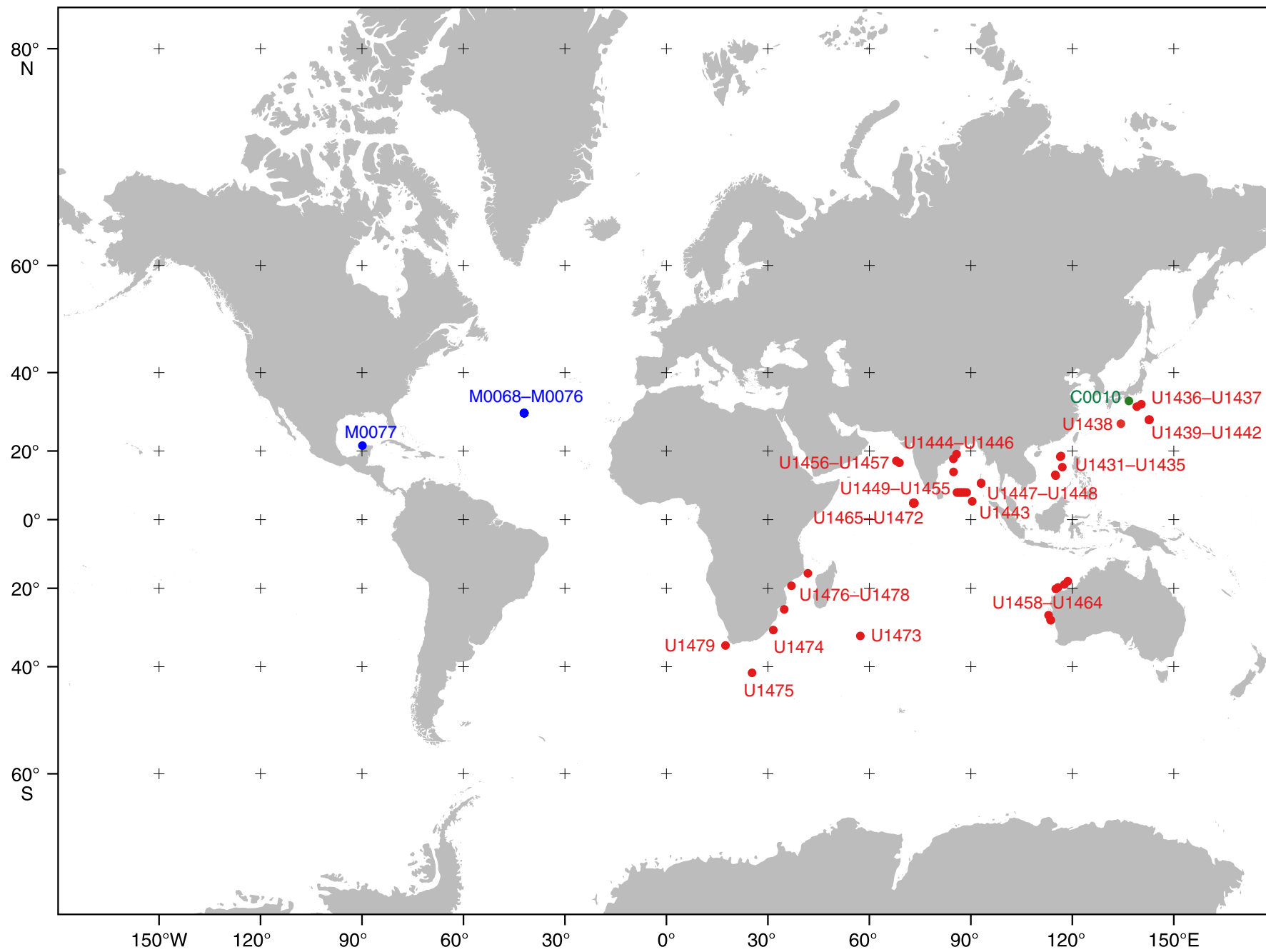
IODP Expeditions 349–357, 359–361, 364–365, Sites C0010 (●), M0068–M0077 (●), U1431–U1479 (●)
