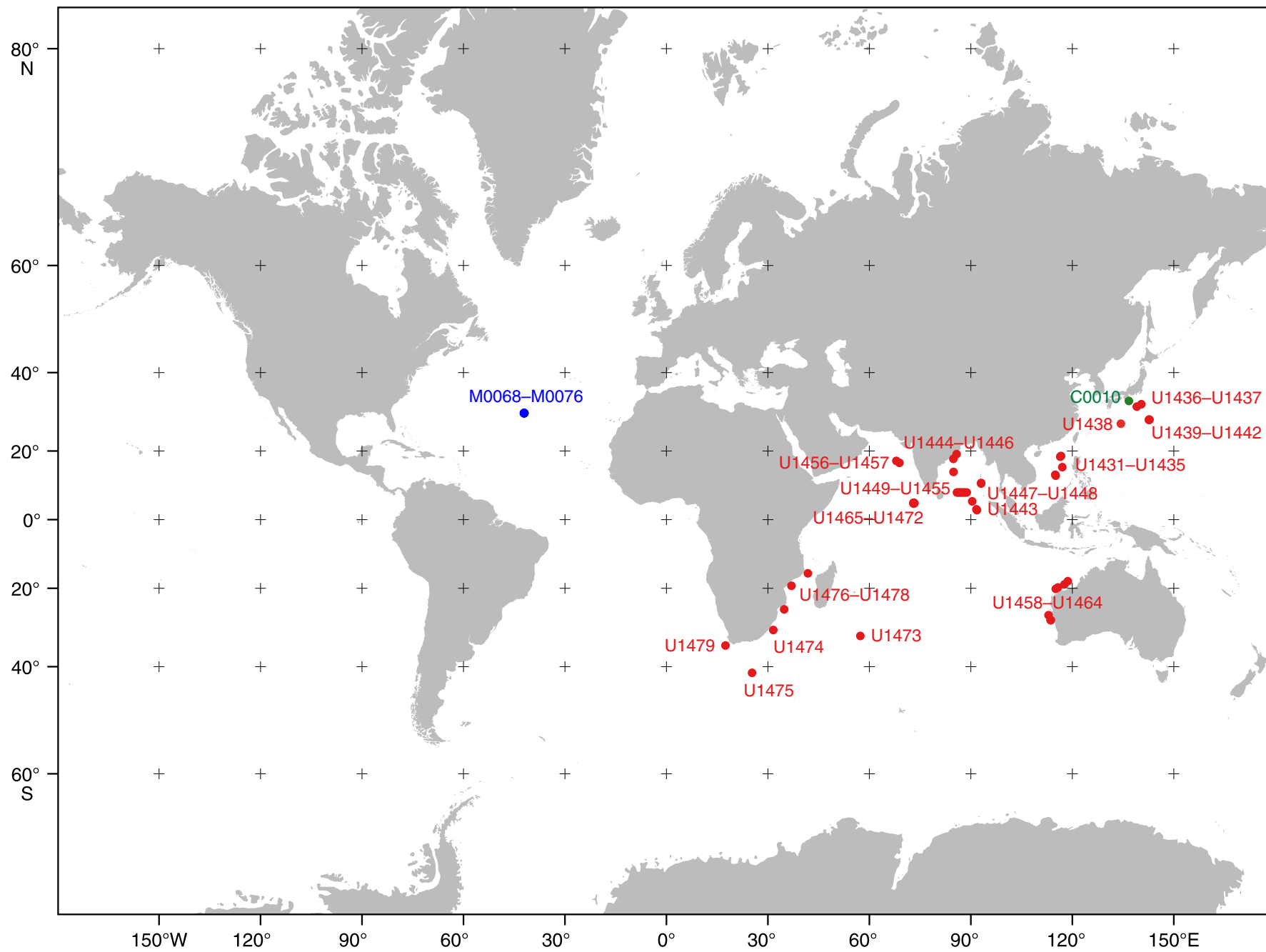
IODP Expeditions 349-357, 359-361, 365 Sites C0010 (●), M0068-M0076 (●), U1431-U1479 (●)
