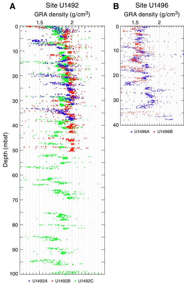
Figure F13. GRA density. A. Holes U1492A–U1492C. Data obtained below 100 mbsf are not plotted. B. Holes U1496A and U1496B.
