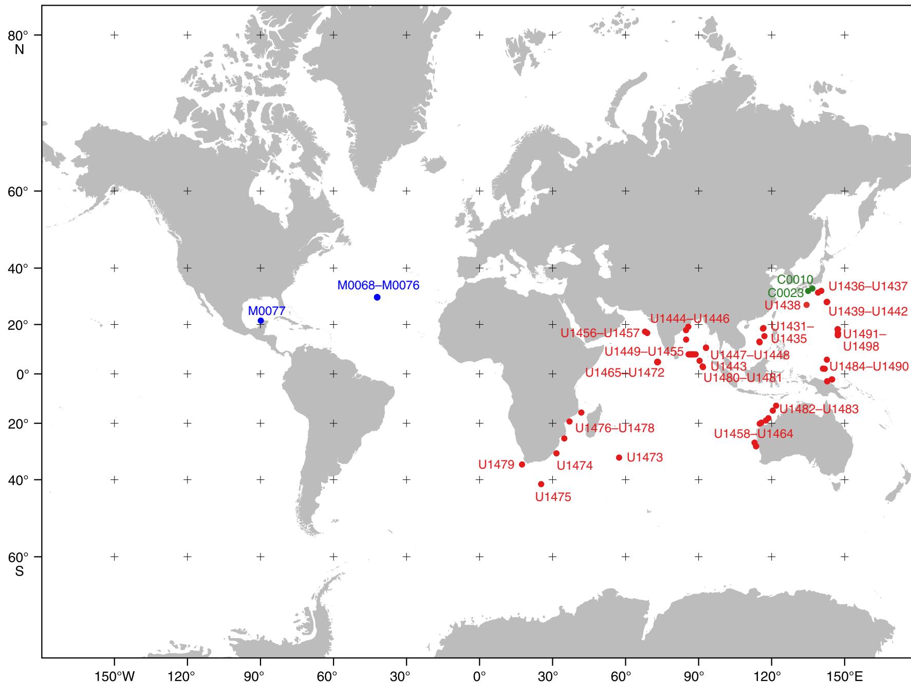
IODP Expeditions 349–357, 359–366, 370, Sites C0010, C0023 (●), M0068–M0077 (●), U1431–U1498 (●)
