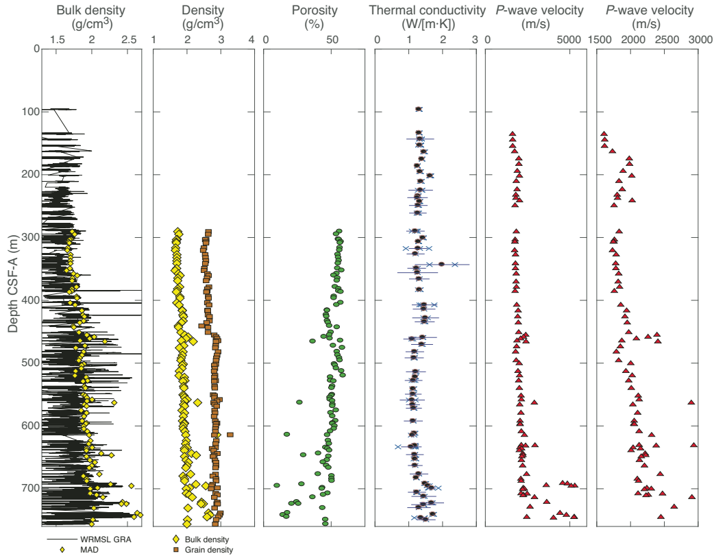
Figure F37. Density, thermal conductivity (bars = 1σ standard deviation), and caliper P-wave velocity, Hole U1513E.
