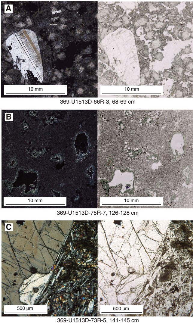
Figure F11. Textural features in Unit VI (see Figure F9), Hole U1513D (left = XPL, right = PPL). A. Plagioclase-phyric basalt with altered microcrystalline groundmass. White pseudophenocrysts are islands of fresh intergranular plagioclase and clinopyroxene groundmass. B. Green highly vesicular basalt. Vesicles are lined with chlorite, and the groundmass has been replaced by chlorite and sericite. C. Dolerite dike containing a xenocryst of plagioclase feldspar with alteration pits and veins. Groundmass consists of plagioclase feldspar, chlorite, clinopyroxene (fresh and altered), and hematite.
