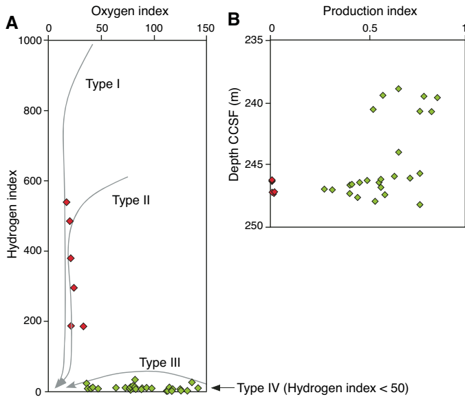
Figure F46. A. Source rock analysis (pyrolysis) results, Site U1513. Data from samples with lower TOC_{SRA} ( <0.8 wt%) are not plotted. B. Production index across the potential OAE 2 interval. Red = samples from a black layer, green = other lithologies.
