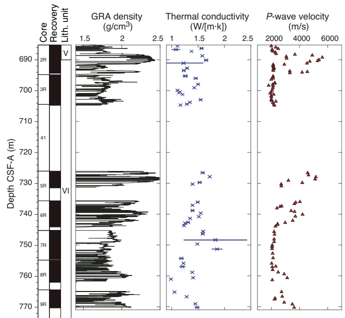
Figure F37. Density, thermal conductivity (bars = 1σ standard deviation), and caliper P-wave velocity, Hole U1513E.
