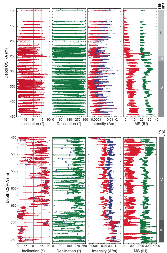
Figure F20. Paleomagnetic results, Hole U1513D. Blue squares = discrete samples. Intensity: blue = 0 mT AF demagnetization, red = 30 mT AF demagnetization. MS: green = whole-round (20 IU offset for 95–450 m CSF-A and 2000 IU offset for 450–760 m CSF-A), red = point source.
