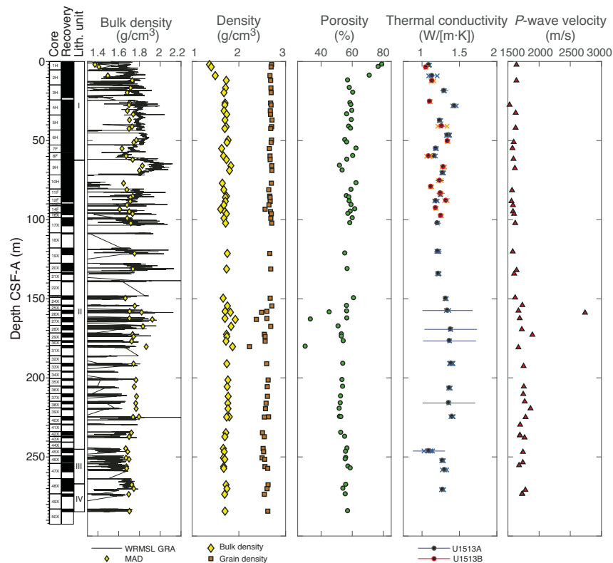
Figure F35. Density, porosity, thermal conductivity (bars = 1σ standard deviation; with additional data from Hole U1513B), and caliper P-wave velocity, Hole U1513A.
