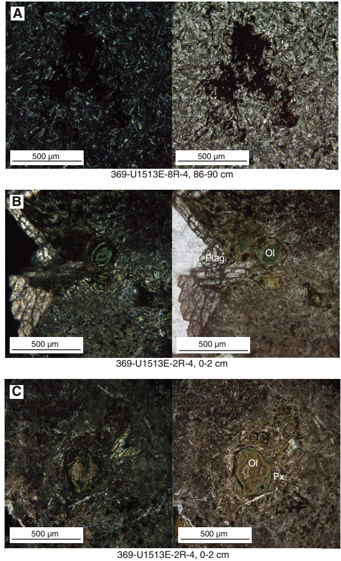
Figure F12. Original igneous textures of volcanics (see Figure F10) in Unit VI, Hole U1513E (left = XPL, right = PPL). A. Green fine-grained basalt with criss-crossing lineation pattern of oxide minerals and showing felty and spherulitic textures of feldspar. B. Olivine-plagioclase-phyric basalt with spherulitic plagioclase (Plag) in groundmass. Plagioclase is replaced by calcite and olivine is pseudomorphed by glauconite and oxide (outline). C. Same section in B showing olivine (Ol) with overgrowth of pyroxene (Px) in spherulitic plagioclase groundmass. Both are altered to palagonite and glauconite.
