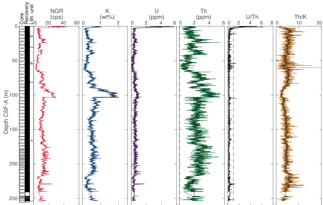
Figure F18. Whole-core NGR data, Hole U1514A. Black data curves = 101-point moving average. U/Th ratio: vertical dashed line = 1:1.
