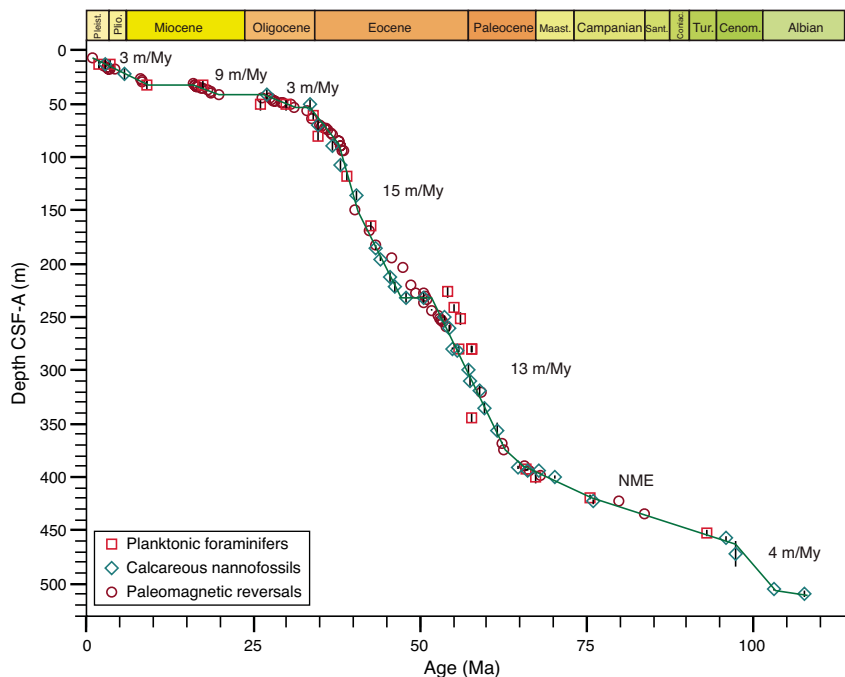
Figure F8. Age-depth plot, Site U1514. The interval corresponding to ~400–460 m CSF-A is structurally disturbed and yields no meaningful estimate (NME) for the sediment accumulation history.
