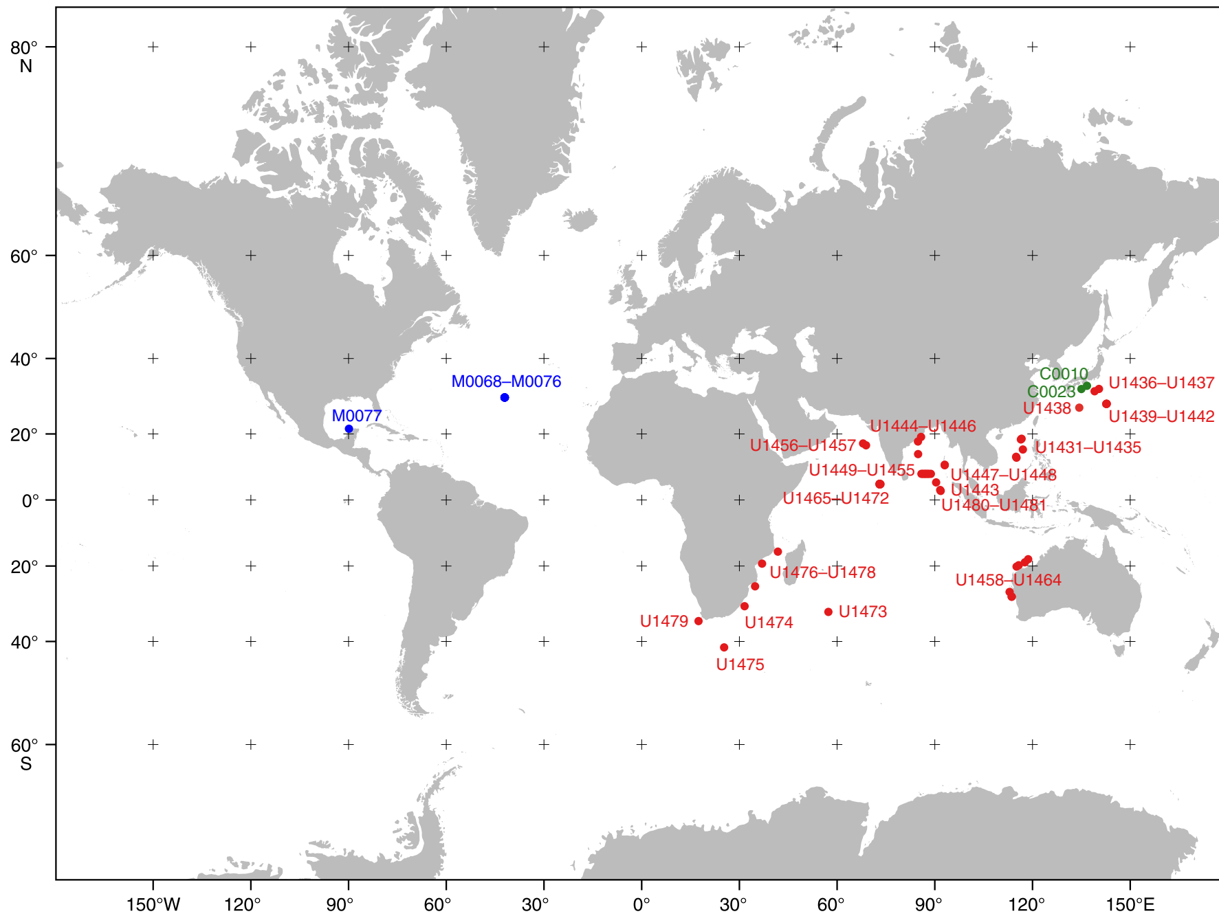
IODP Expeditions 349–357, 359–362, 364–365, 370, Sites C0010, C0023 (●), M0068–M0077 (●), U1431–U1481 (●)
