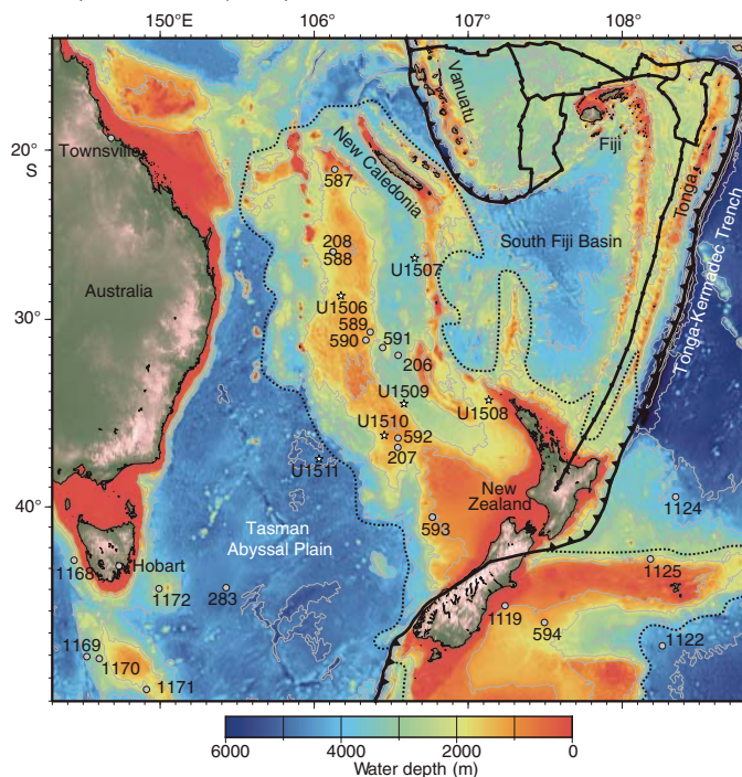
Figure F2. Location of Sites U1506–U1511 (stars) in the southwest Pacific. Dots = relevant DSDP and ODP sites. The expedition departed from Townsville and returned to Hobart. Dashed line = approximate location of Zealandia (Mortimer et al., 2017).
