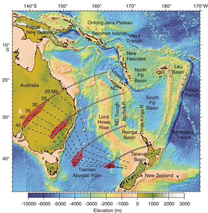
Figure F8. Australia-Pacific relative plate motion history plotted on Tasman Frontier bathymetric features (NC = New Caledonia, R = ridge) (after Bache et al., 2012). Australian plate points are reconstructed relative to a fixed Pacific plate at 1 My intervals. Dashed lines = relocated positions of Norfolk Ridge at 5 My intervals, revealing that plate motion rates were low in New Zealand during the interval 45–25 Ma.
