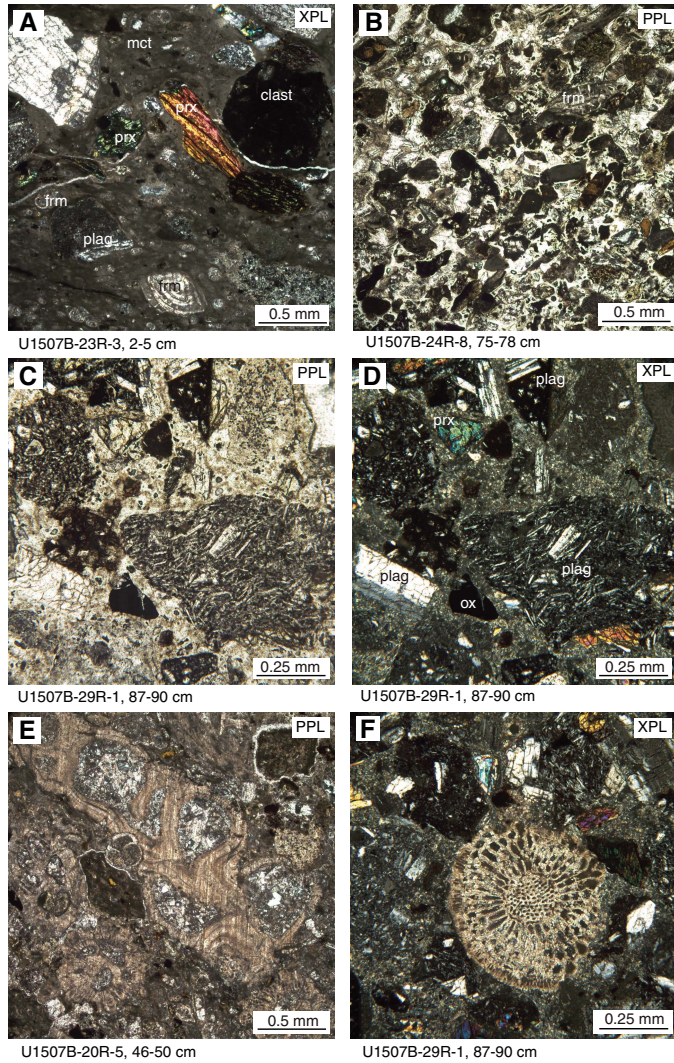
Figure F13. Common Subunit Ic sedimentary lithologies, Site U1507. A. Lower Oligocene clayey foraminiferal (frm) chalk with volcanic clasts. mct = micrite, prx = pyroxene, plag = plagioclase. B. Lower Oligocene tuffaceous sandstone. C, D. Upper Oligocene tuff. Note the isolated pyroxene grains, microcrystalline basalt clasts with plagioclase, and an altered (reddish brown) vesicular clast. ox = oxide. E. Lower Oligocene clayey foraminiferal (gastropod?). F. Upper Oligocene tuff with a shallow-water coral or bryozoan.
