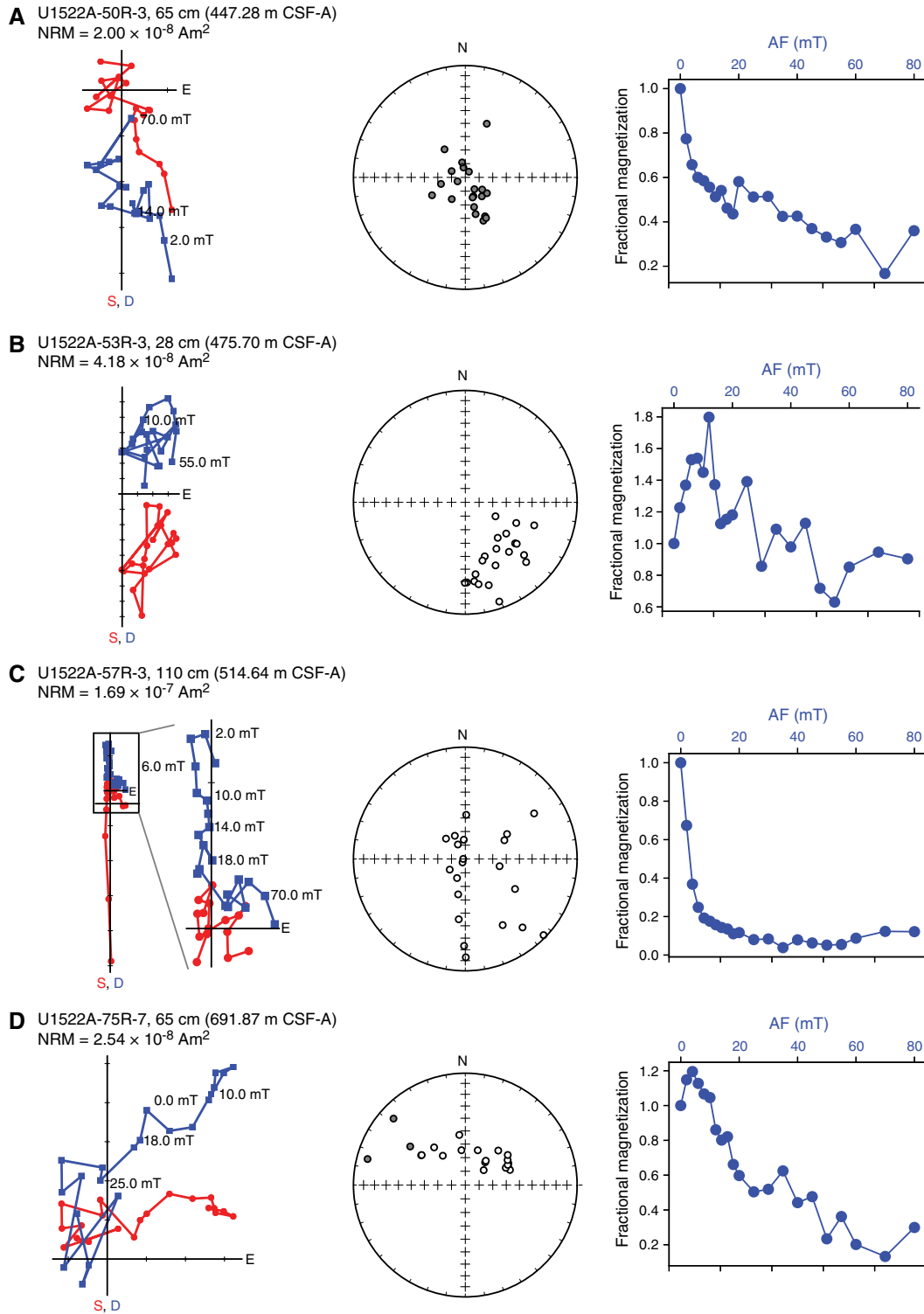
Figure F17. Representative AF demagnetization behavior of oriented discrete samples, Site U1522. From left to right for each sample: Zijdeveld diagram with peak AF fields and initial NRM, equal area projection of directions during demagnetization (solid gray circles = lower hemisphere, open circles = upper hemisphere), and fractional magnetization (normalized to initial NRM) during AF demagnetization. A. Sample from reversed polarity zone. B. Sample without stable remanence from which no ChRM direction is estimated. C, D. Samples from a normal polarity zone.
