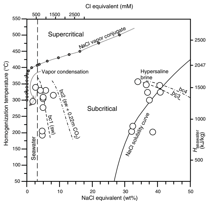
Figure F14. Salinity (NaCl equivalent wt%) vs. homogenization temperature and corresponding enthalpy of NaCl-H 2 O (Bischoff and Rosenbauer, 1985) for fluid inclusions from anhydrite, gypsum, and natroalunite recovered from Site U1528. NaCl saturation curve calculated from Driesner and Heinrich (2007), and NaCl vapor conjugate curve calculated from Bischoff (1991). Phase separation (boiling) curves calculated for seawater (sw) + 0.22 m CO 2 (bc2), 33 wt% NaCl equivalent hypersaline brine (bc3), and 33 wt% NaCl equivalent hypersaline brine + 0.22 m CO 2 . Broken line with arrow = salinities caused by vapor condensation under subcritical conditions.
