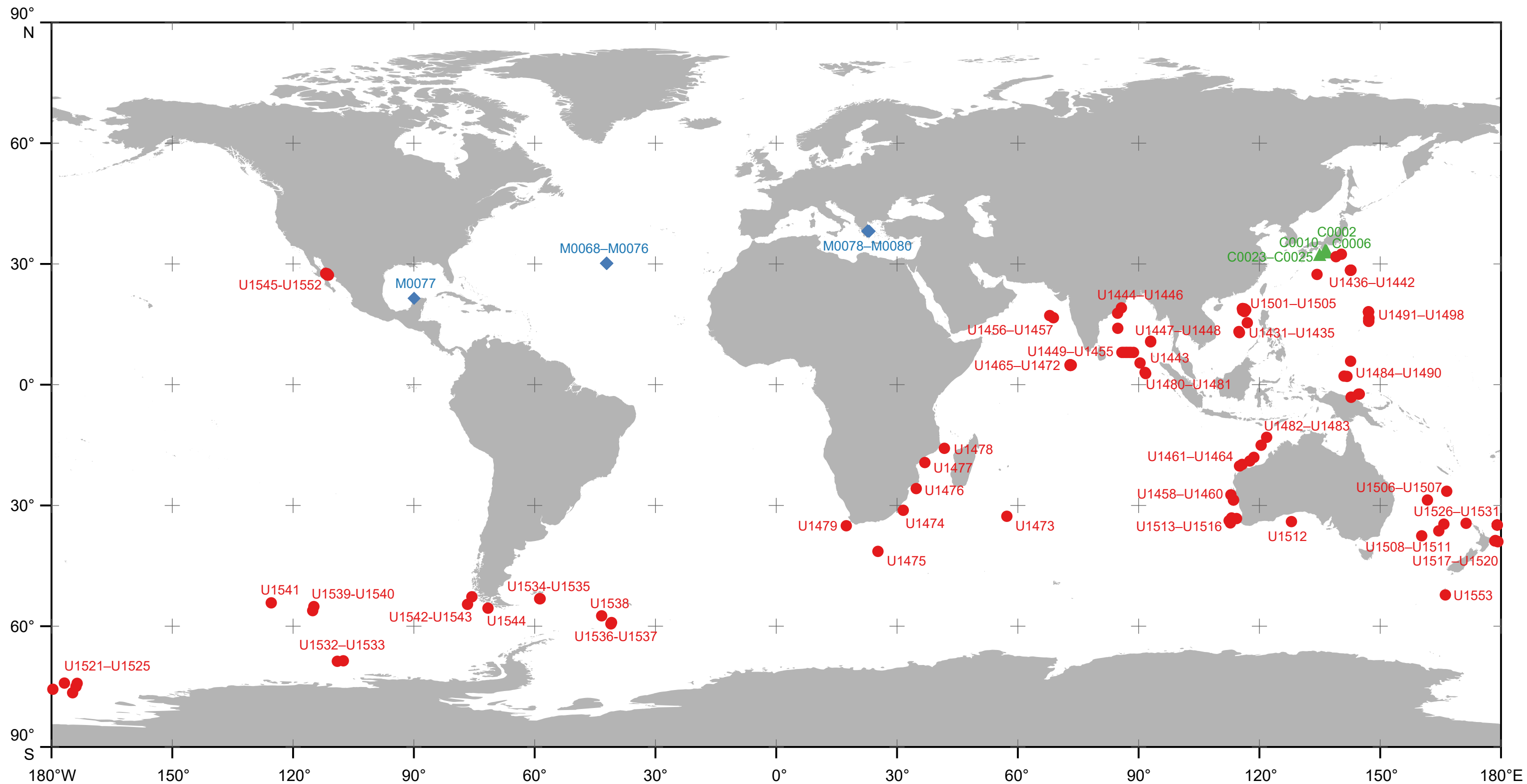
IODP Expeditions 349–372, 374–376, 378–383, 385, Sites C0002, C0006, C0010, C0023–C0025 (▲), M0068–M0080 (◆), U1431–U1553 (●)
