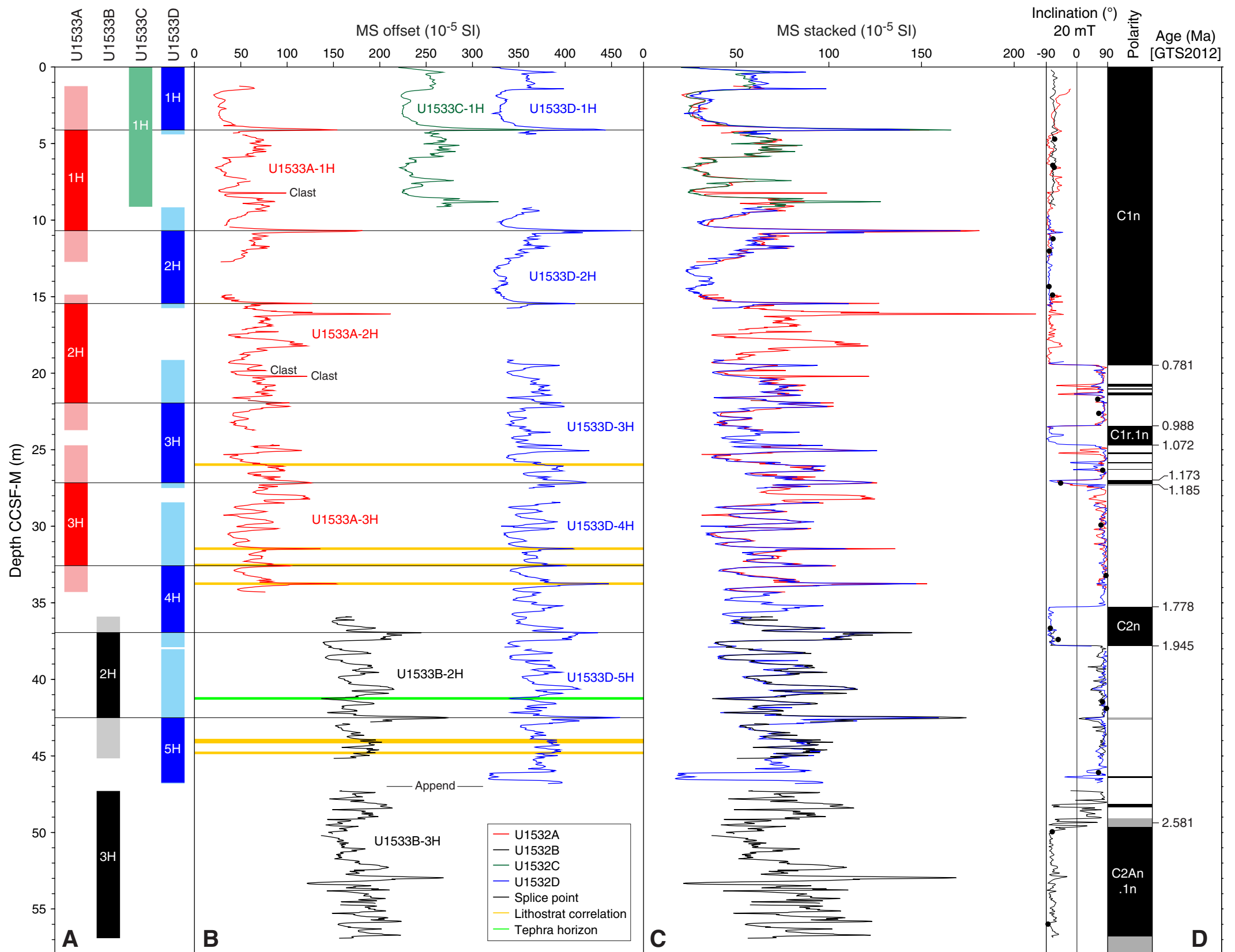
Expedition 379 Site U1533, Figure F40. Composite splice framework for the uppermost sediment sequence recovered at Site U1533. A. Core positions showing in-splice (dark) and out-of-splice (light) intervals. B. Whole-round MS data offset according to hole: Hole U1533A = +0, Hole U1533B = +100, Hole U1533C = +200, Hole U1533D = +300. C. Stacked whole-round MS data. D. Paleomagnetic inclination data and polarity/chron interpretations. Black circles = discrete samples. https://doi.org/10.14379/iodp.proc.379.104.2021
