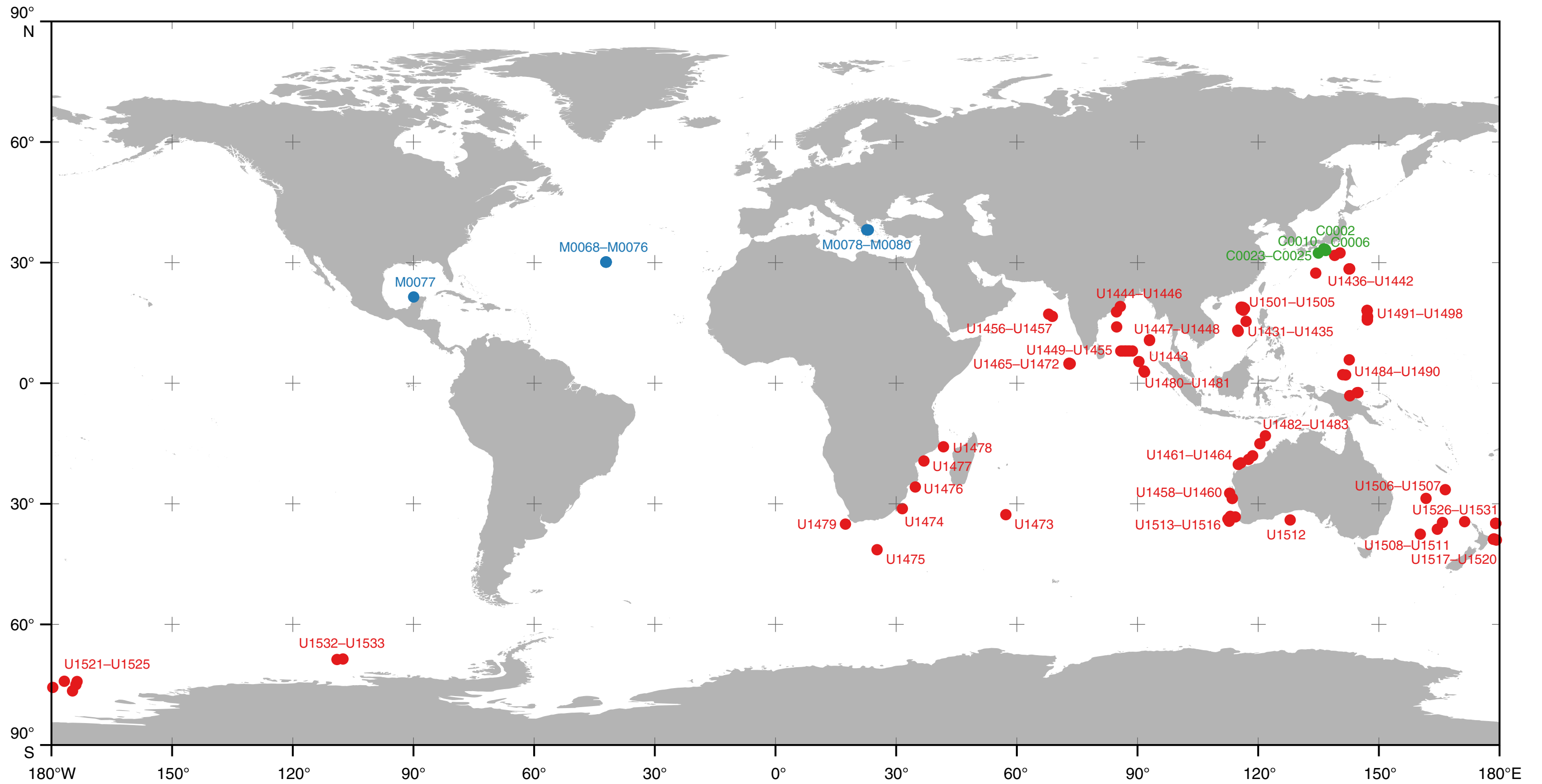
IODP Expeditions 349–372, 374–376, 379–381, Sites C0002, C0006, C0010, C0023–C0025 (●), M0068–M0080 (●), U1431–U1533 (●)
