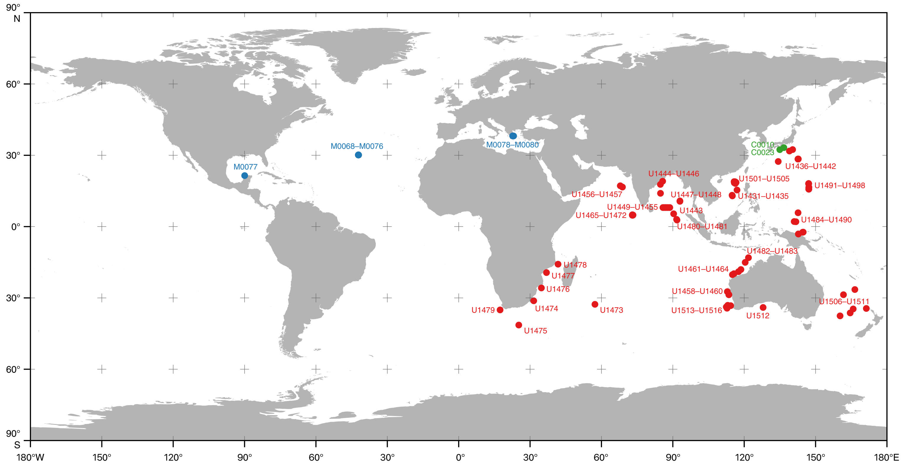
IODP Expeditions 349–357, 359–371, 381, Sites C0010, C0023 (●), M0068–M0080 (●), U1431–U1516 (●)
