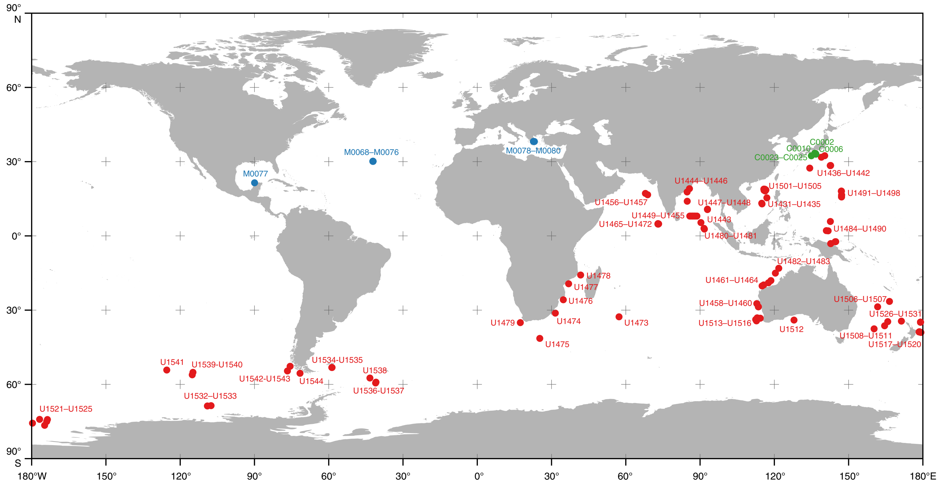
IODP Expeditions 349–372, 374–376, 379–383, Sites C0002, C0006, C0010, C0023–C0025 (●), M0068–M0080 (●), U1431–U1544 (●)
