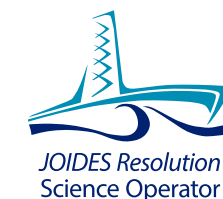
IODP Expeditions 349–372, 374–376, 378–386, 389–393, 395–400, Sites C0002, C0006, C0010, C0023–C0025 (▲), M0068–M0110 (◆), U1431–U1608 (●)
