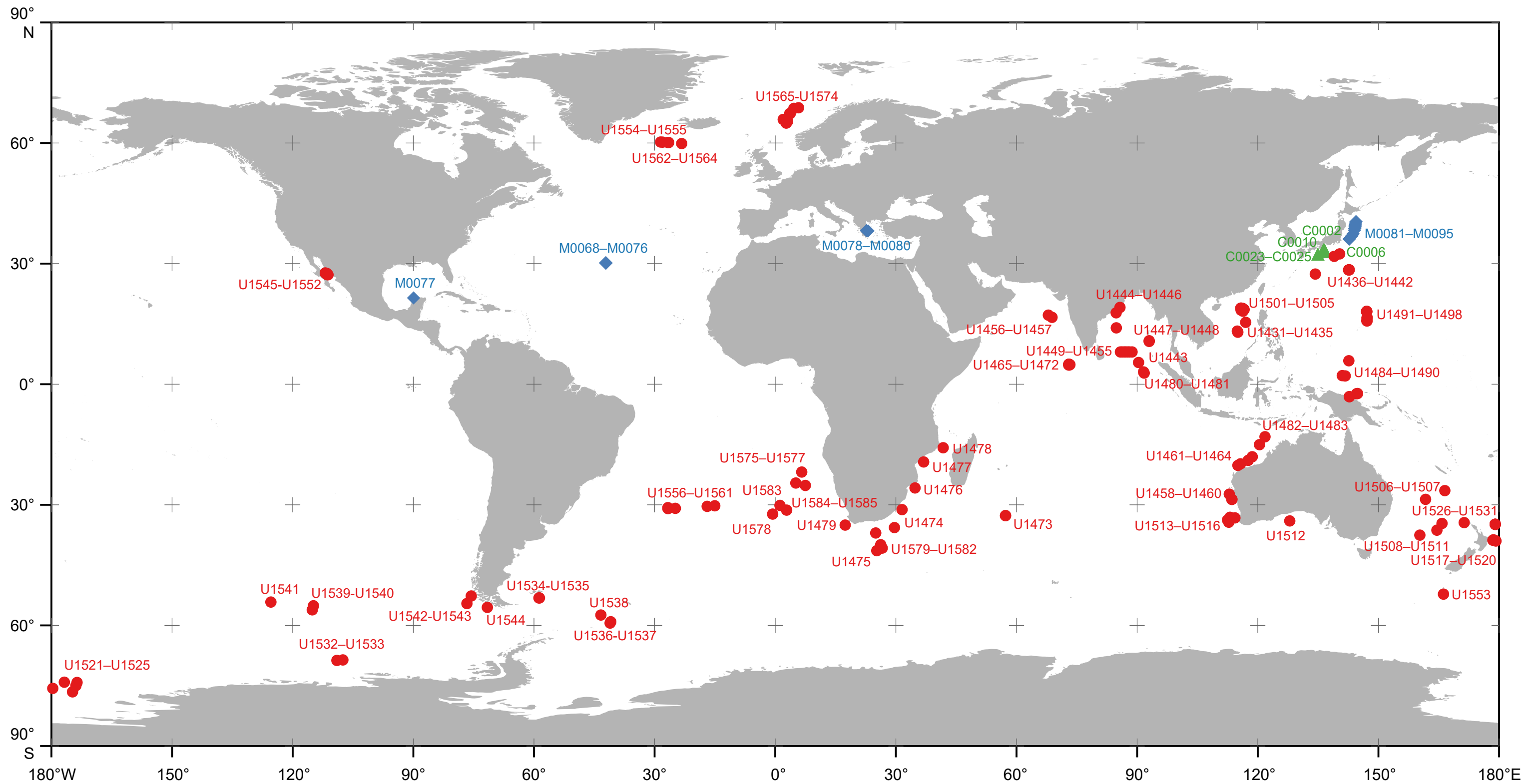
IODP Expeditions 349–372, 374–376, 378–386, 390C, 390–393, 396, Sites C0002, C0006, C0010, C0023–C0025 (▲), M0068–M0095 (◆), U1431–U1585 (●)
