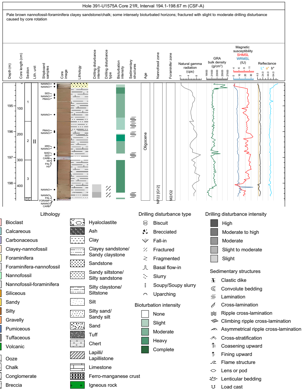
Example VCD and lithology patterns, symbols, and nomenclature used for VCDs, Expedition 391. cps = counts per second.
