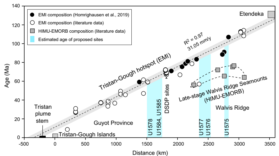
Figure F6. Walvis Ridge age progression from radiometrically dated igneous rocks. Samples with EMI composition follow a tight linear trend. Exceptions are samples with HIMU-type composition that yield ages ~30–40 Myr younger than the underlying basement with an EMI-type geochemical composition. Vertical blue bands = Expedition 391 and 397T cored sites (see Homrighausen et al. [2019] for sources of age data). EMORB = enriched mid-ocean-ridge basalt.
