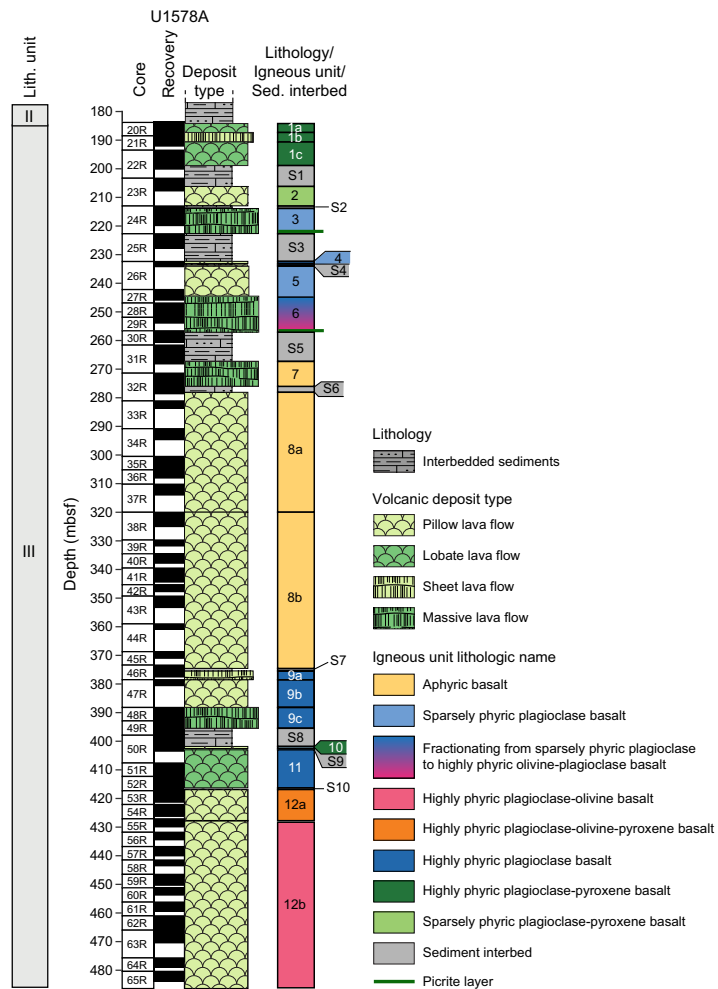
Figure F31. Stratigraphic column for igneous basement, Hole U1578A.
