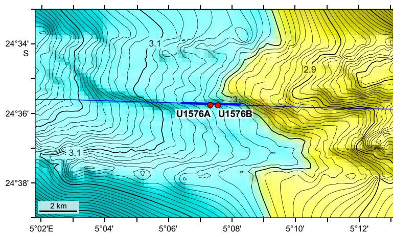
Figure F18. Bathymetry of Site U1576 and environs. Detailed multibeam bathymetry around Seismic Line TN373-VB08 is merged with the SRTM15+ bathymetry grid (Tozer et al., 2019). Contours are plotted at 10 m intervals and labeled in kilometers. Blue line represents Seismic Line TN373-VB08. Heavy blue line shows the portion of the line shown by Figure F19.
