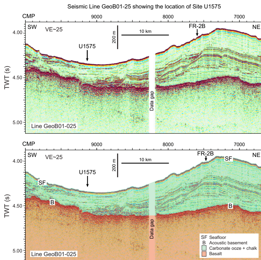
Figure F14. Seismic Line GeoB01-25. Top: seismic profile. Bottom: seismic line interpretation. TWT = two-way travelttime, VE = vertical exaggeration.
