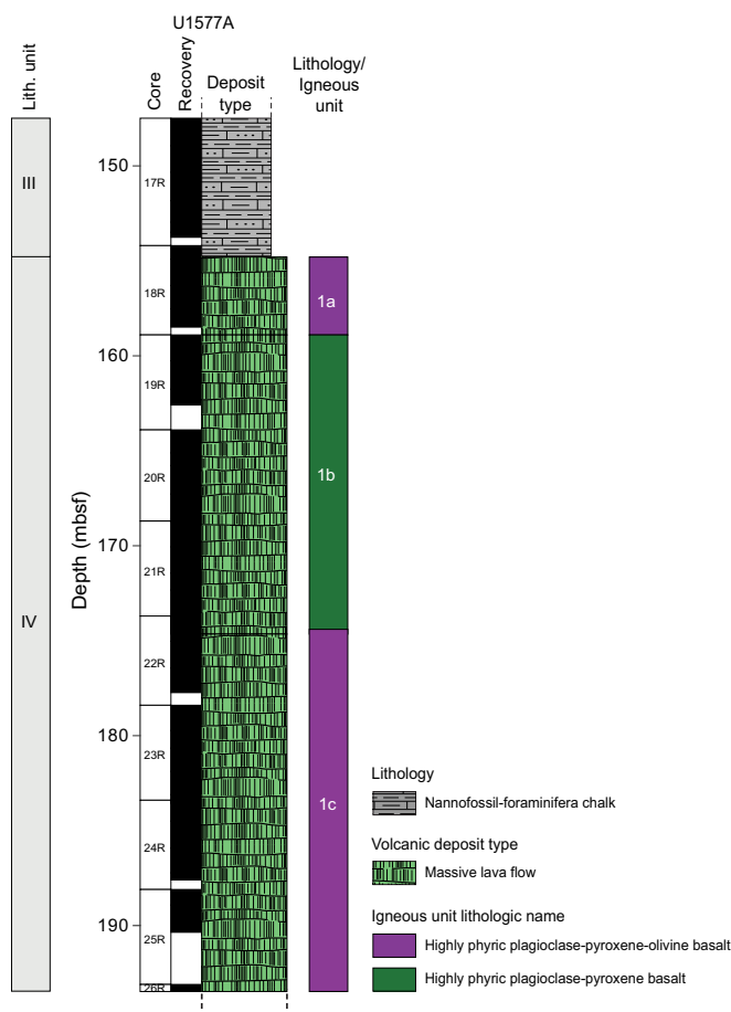
Figure F26. Stratigraphic column for igneous basement, Hole U1577A.
