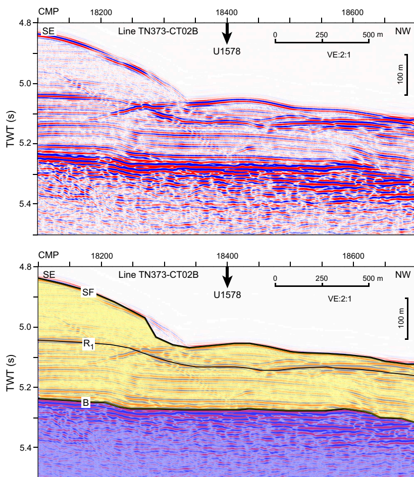
Figure F27. Seismic Line TN373-CT2B over Site U1578. Top: uninterpreted seismic profile. Arrow = location of Site U1578. Bottom: seismic line interpretation. TWT = two-way travelttime, VE = vertical exaggeration.
