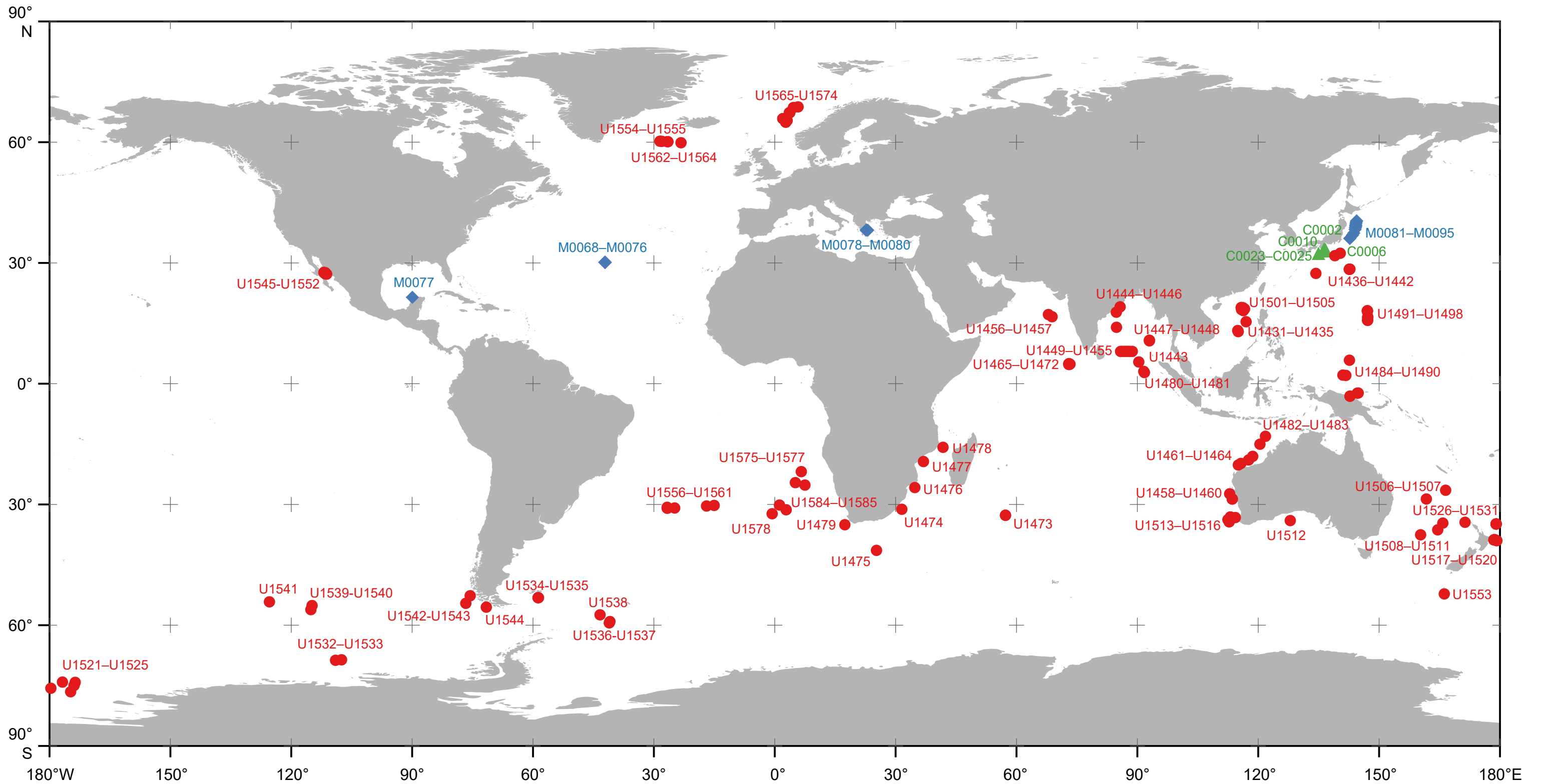
IODP Expeditions 349–372, 374–376, 378–386, 390C, 391, 396, Sites C0002, C0006, C0010, C0023–C0025 (▲), M0068–M0095 (◆), U1431–U1578, U1584–U1585 (●)
