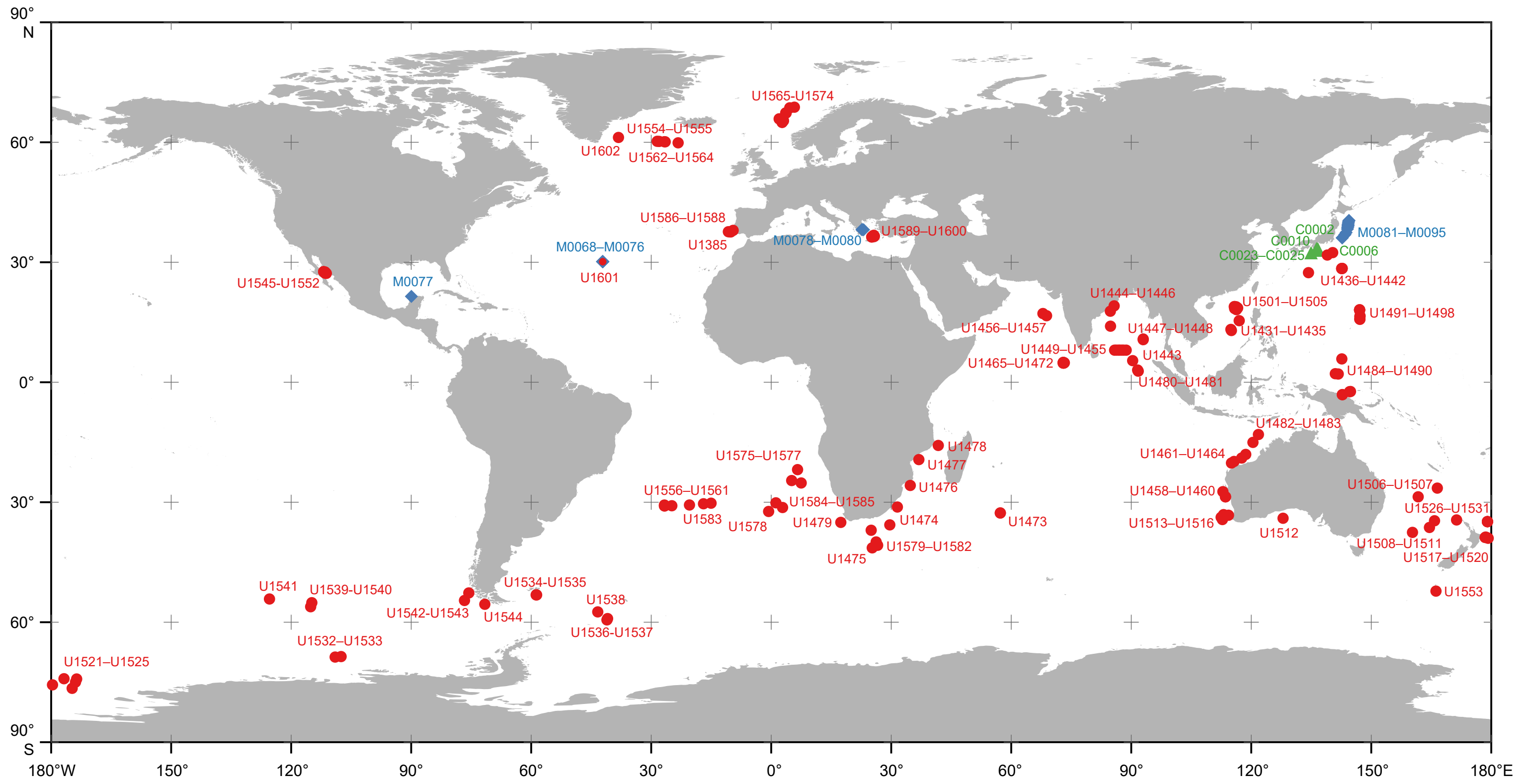
IODP Expeditions 349–372, 374–376, 378–386, 390–393, 395–399, Sites C0002, C0006, C0010, C0023–C0025 (▲), M0068–M0095 (◆), U1431–U1555, U1562–U1602 (●)
