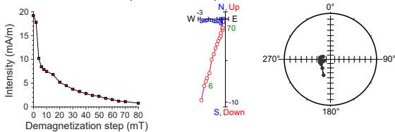
397-U1586A-17H-2, 74 cm | 151.14 m CSF-A | JR6 data
