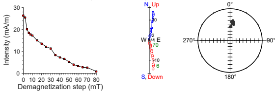
397-U1586A-15H-2, 74 cm | 132.14 m CSF-A | SRM data
