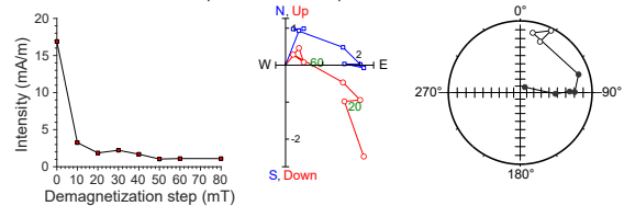
397-U1586A-18H-3, 71 cm | 162.08 m CSF-A | JR6 data
