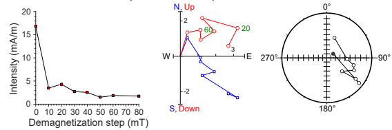
397-U1586A-18H-5, 74 cm | 165.11 m CSF-A | SRM data
