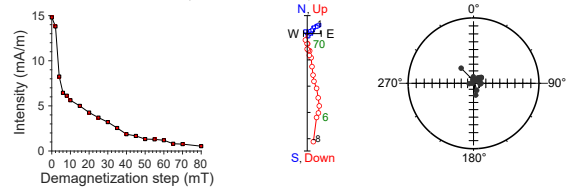
397-U1586A-16H-4, 74 cm | 144.68 m CSF-A | SRM data
