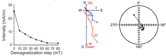
397-U1586A-17H-4, 74 cm | 154.11 m CSF-A | JR6 data
