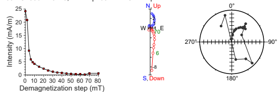
397-U1586A-19H-2, 72 cm | 170.14 m CSF-A | SRM data
