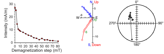
397-U1586A-15H-6, 74 cm | 138.07 m CSF-A | SRM data
