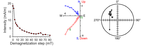
397-U1586A-16H-2, 74 cm | 141.64 m CSF-A | SRM data
