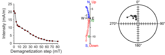
397-U1586A-14H-4, 74 cm | 125.62 m CSF-A | SRM data
