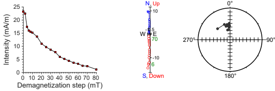
397-U1586A-14H-6, 74 cm | 128.6 m CSF-A | SRM data
