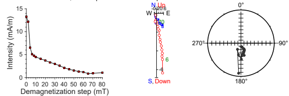
397-U1586A-18H-1, 71 cm | 159.12 m CSF-A | JR6 data
