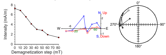
397-U1586A-32X-1, 83 cm | 248.05 m CSF-A | SRM data
