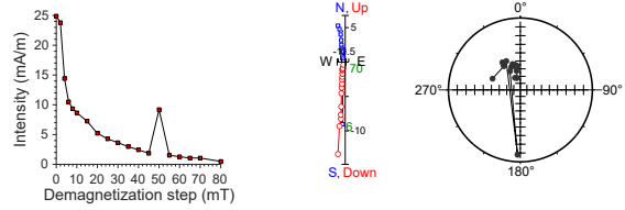
397-U1586A-23F-2, 74 cm | 193.77 m CSF-A | SRM data
