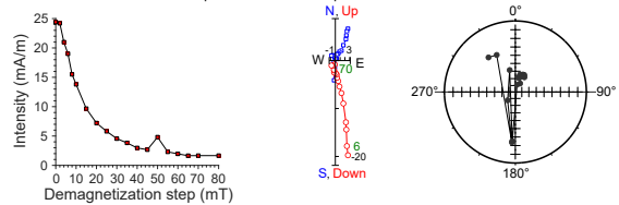
397-U1586A-32X-5, 27 cm | 253.43 m CSF-A | SRM data
