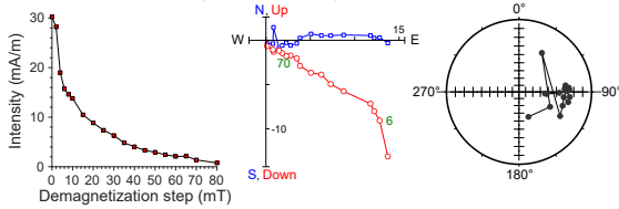
397-U1586A-21F-2, 99 cm | 184.6 m CSF-A | SRM data
