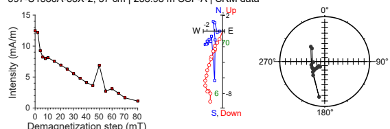
397-U1586A-33X-2, 57 cm | 258.98 m CSF-A | SRM data
