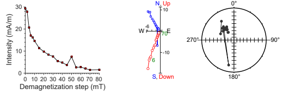
397-U1586A-24F-2, 69 cm | 198.42 m CSF-A | SRM data
