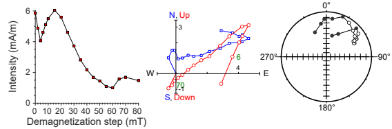
397-U1586A-32X-3, 95 cm | 251.14 m CSF-A | SRM data
