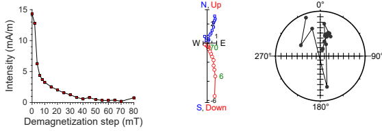
397-U1586A-19H-6, 79 cm | 176.19 m CSF-A | SRM data
