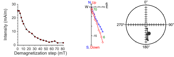
397-U1586A-35X-5, 71 cm | 282.7 m CSF-A | SRM data
