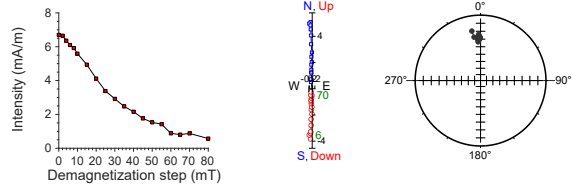
397-U1586A-35X-1, 77 cm | 277.09 m CSF-A | SRM data
