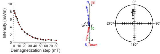
397-U1586A-34X-4, 64 cm | 271.73 m CSF-A | SRM data
