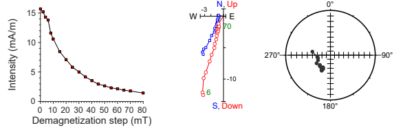
397-U1586A-35X-3, 76 cm | 279.9 m CSF-A | SRM data
