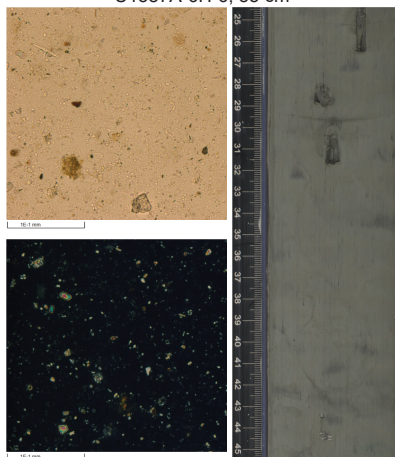
Silty clay with nannofossil ooze U1587A-6H-6, 35 cm
