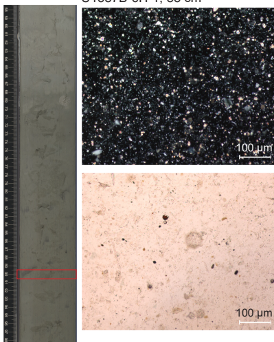
Nannofossil ooze with clay and biosilica U1587B-6H-1, 88 cm
