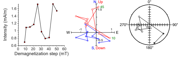
397-U1587B-17X-3, 74 cm | 156.54 m CSF-A | SRM data
