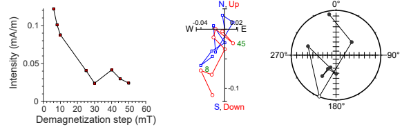
397-U1587B-21X-6, 31 cm | 191.7 m CSF-A | SRM data
