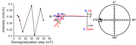
397-U1587B-27X-1, 114 cm | 236.56 m CSF-A | SRM data
