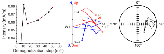
397-U1587B-27X-1, 129 cm | 236.71 m CSF-A | SRM data
