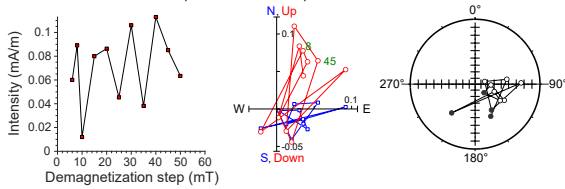
397-U1587B-22X-3, 88 cm | 197.49 m CSF-A | SRM data
