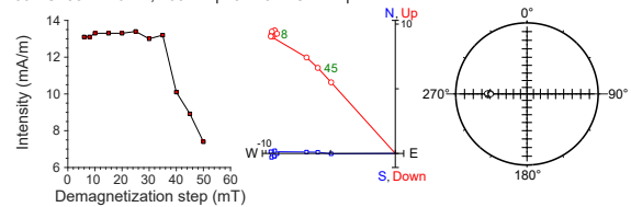
397-U1587B-27X-2, 19 cm | 237.1 m CSF-A | SRM data
