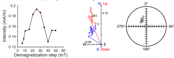
397-U1587B-27X-1, 35 cm | 235.77 m CSF-A | SRM data
