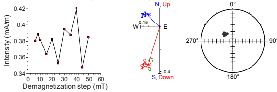
397-U1587B-27X-1, 66 cm | 236.08 m CSF-A | SRM data
