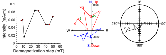
397-U1587B-21X-7, 14 cm | 192.93 m CSF-A | SRM data
